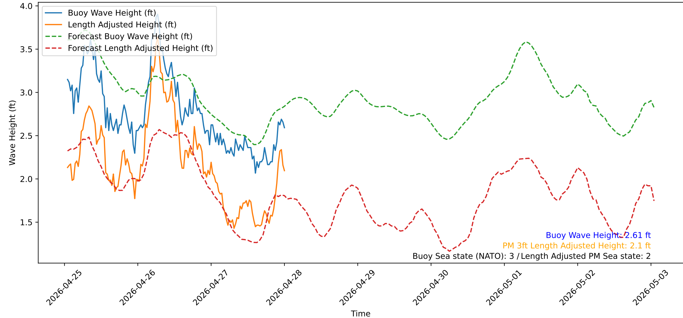
Wave Heights over Time for Oceanside Harbor at 2026-04-28 01:00:31
