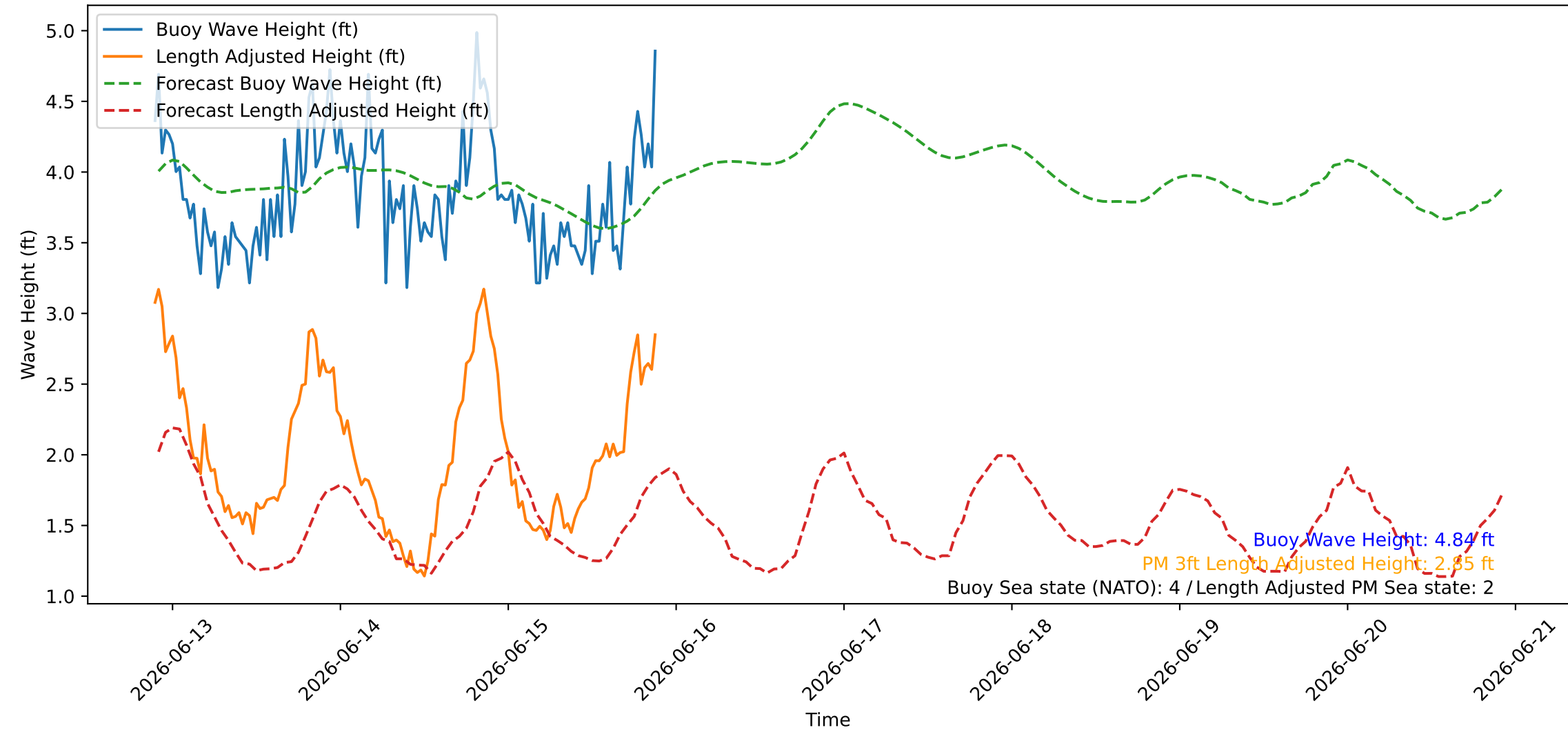
Wave Heights over Time for Oceanside Harbor at 2026-06-15 21:40:25
