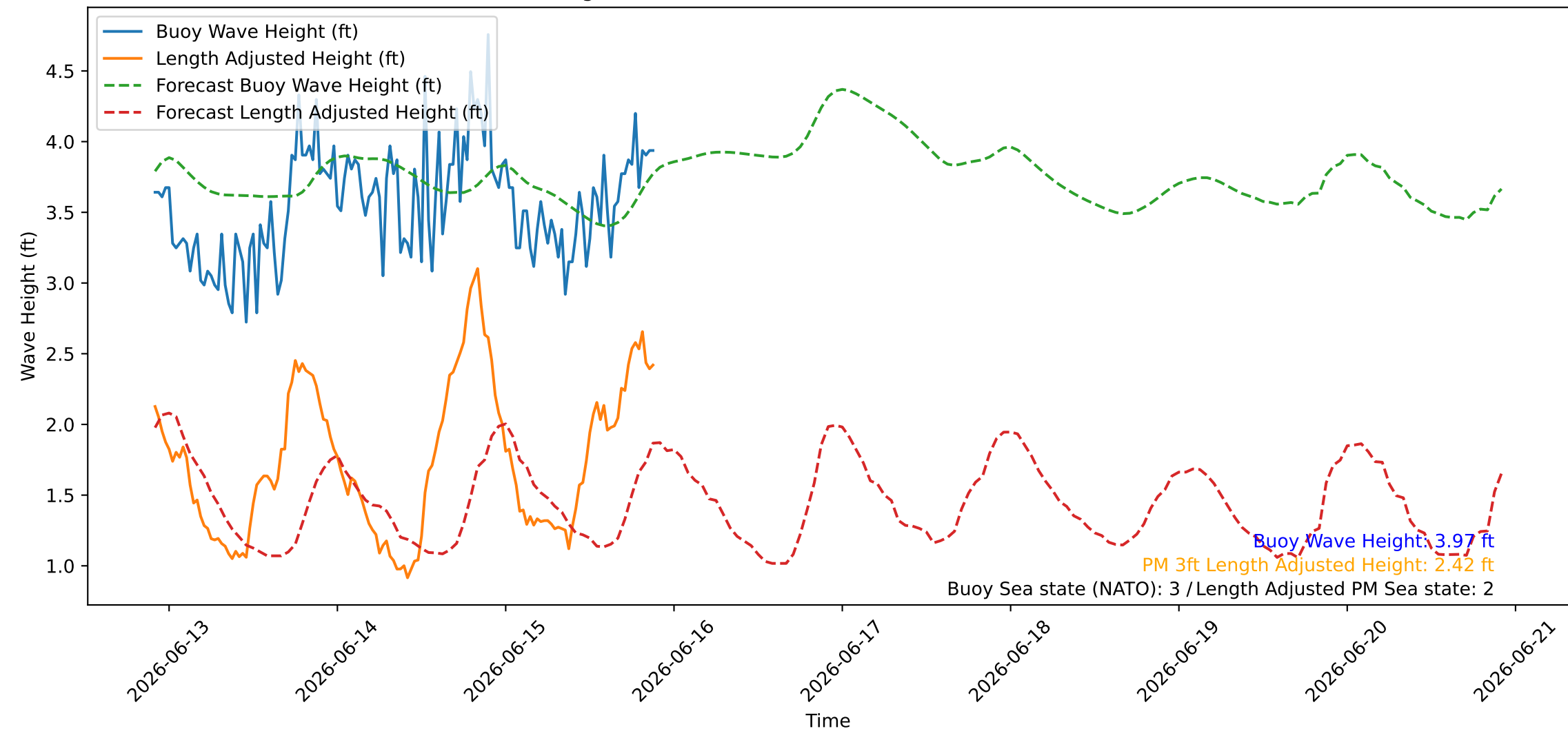
Wave Heights over Time for Red Beach at 2026-06-15 21:40:44
