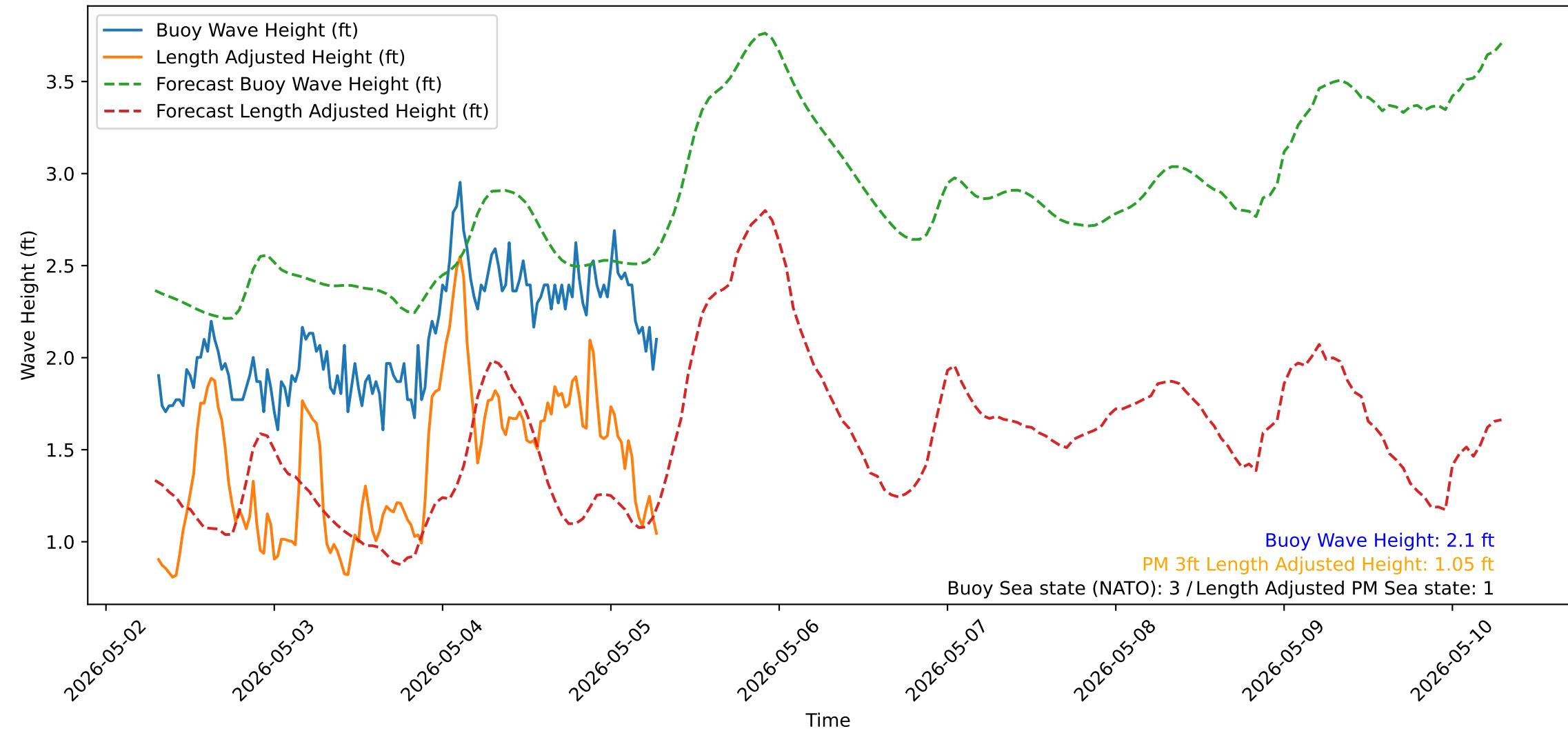
Wave Heights over Time for Red Beach at 2026-05-05 07:20:52
