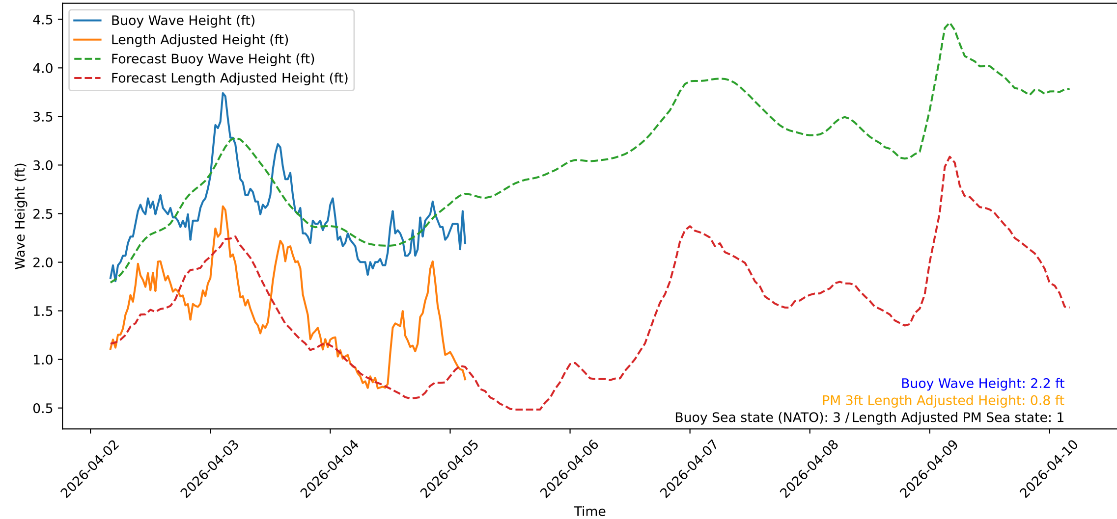
Wave Heights over Time for Red Beach at 2026-04-05 03:50:49
