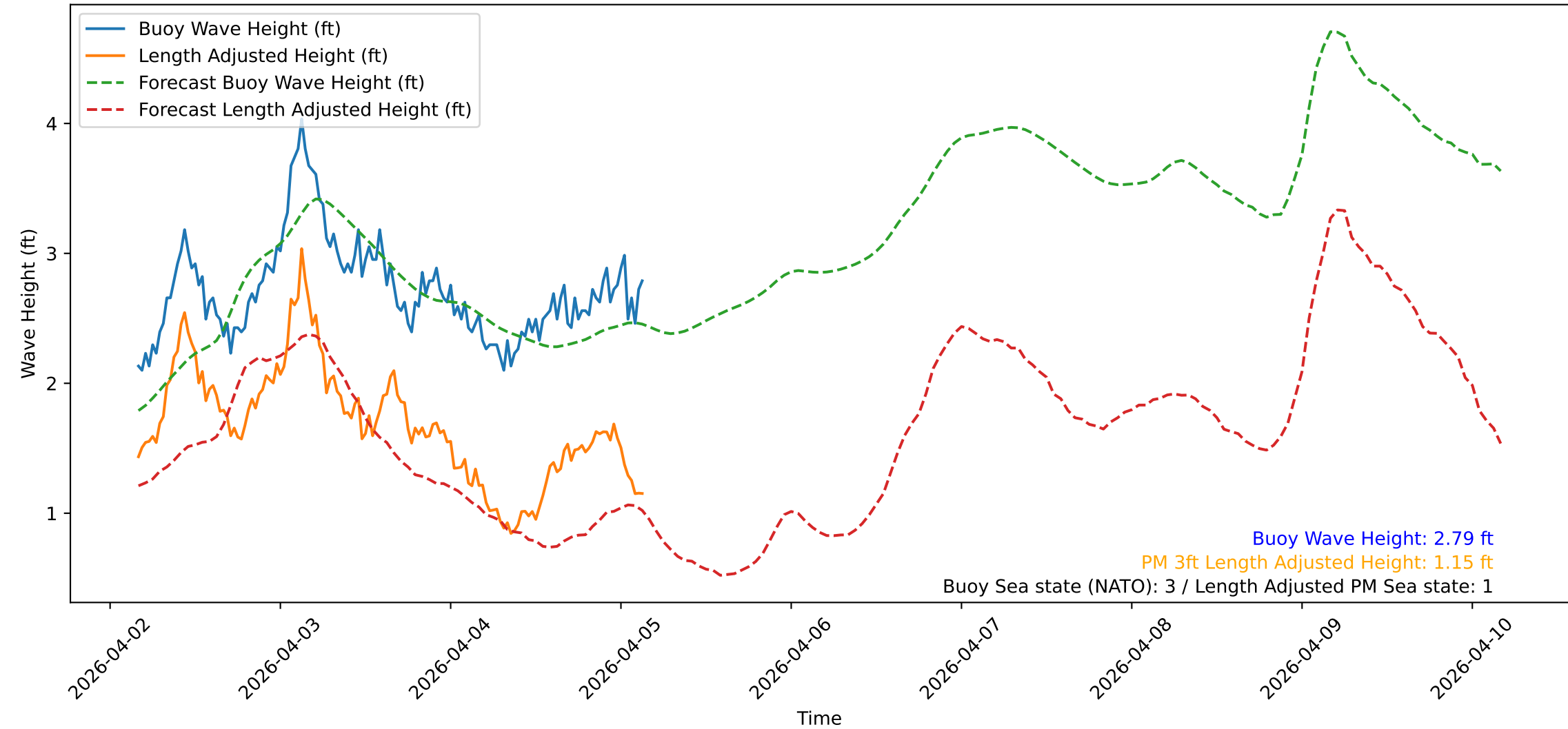
Wave Heights over Time for Oceanside Harbor at 2026-04-05 03:50:32
