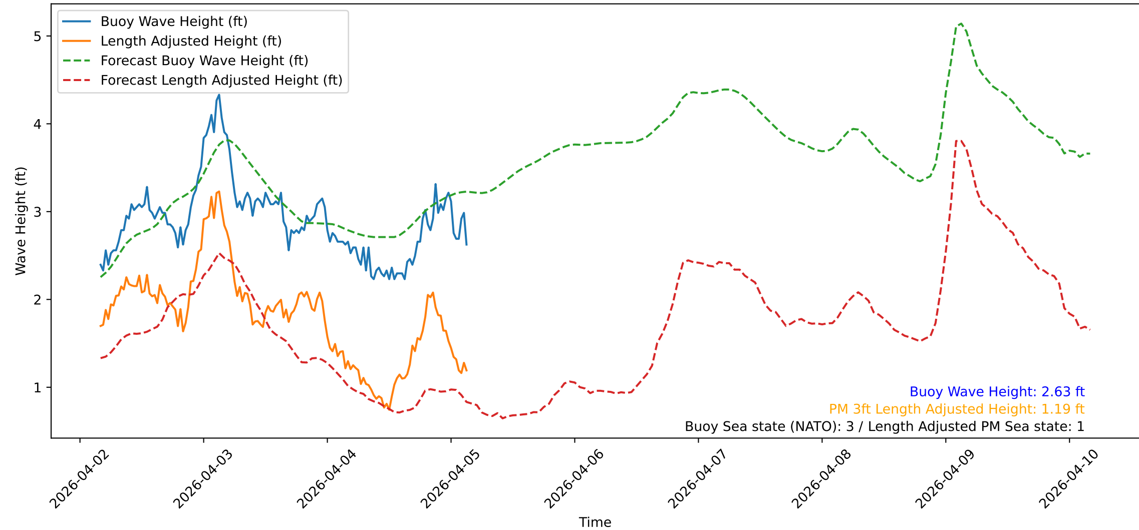
Wave Heights over Time for Green Beach at 2026-04-05 03:51:11
