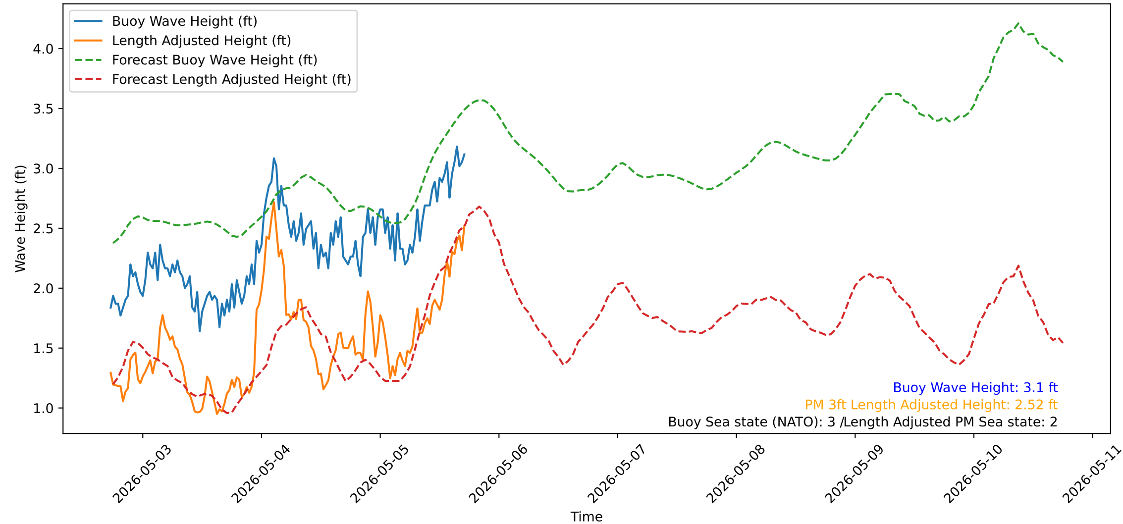
Wave Heights over Time for Oceanside Harbor at 2026-05-05 17:30:31
