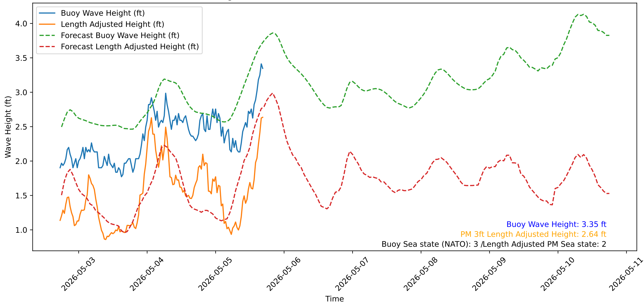
Wave Heights over Time for Green Beach at 2026-05-05 17:31:13
