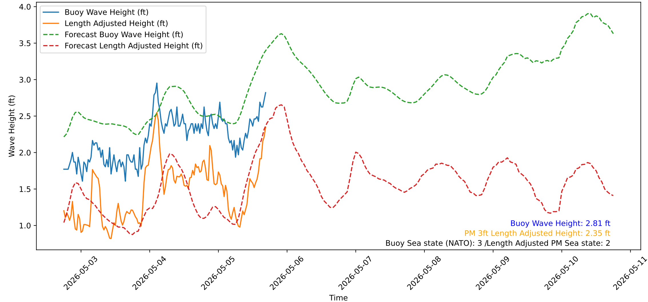
Wave Heights over Time for Red Beach at 2026-05-05 17:30:51
