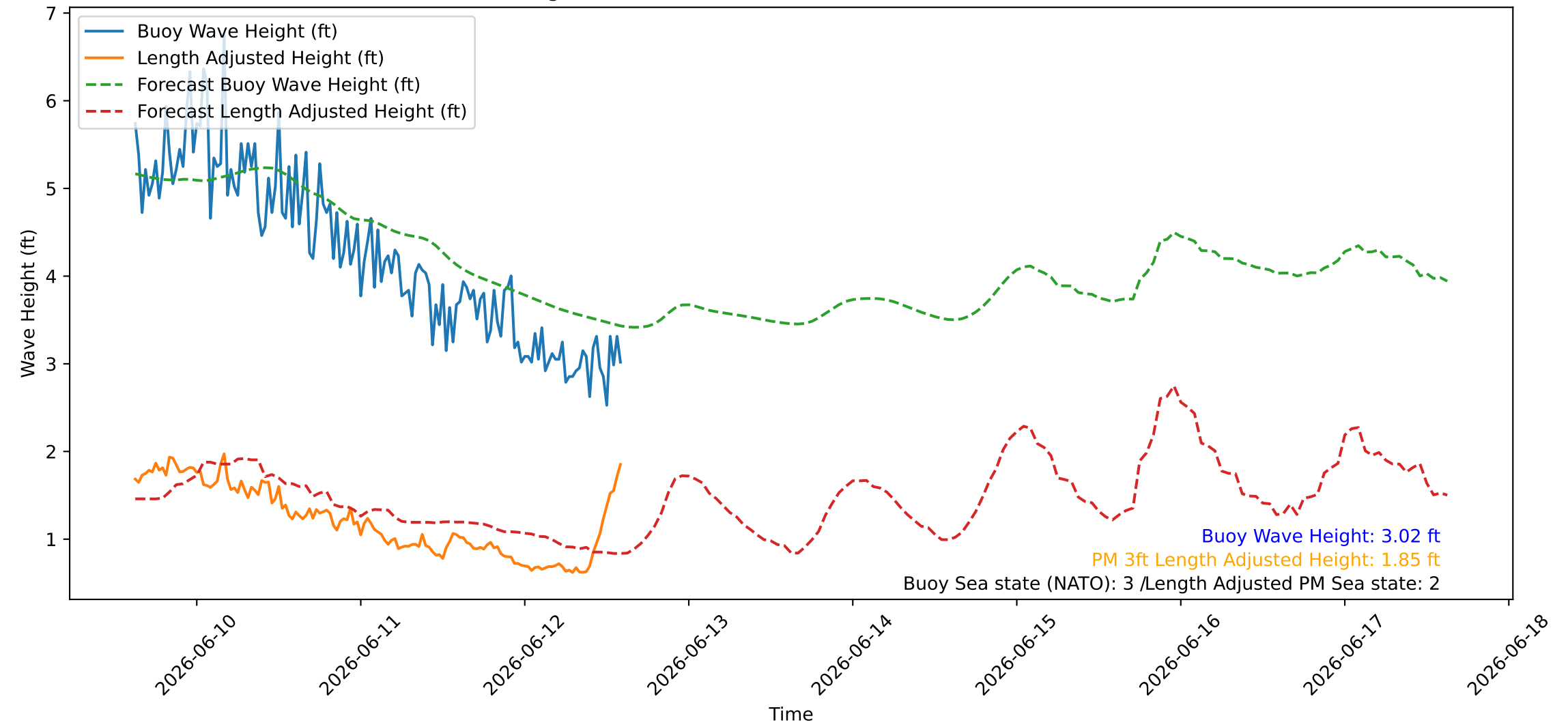
Wave Heights over Time for Red Beach at 2026-06-12 14:40:45
