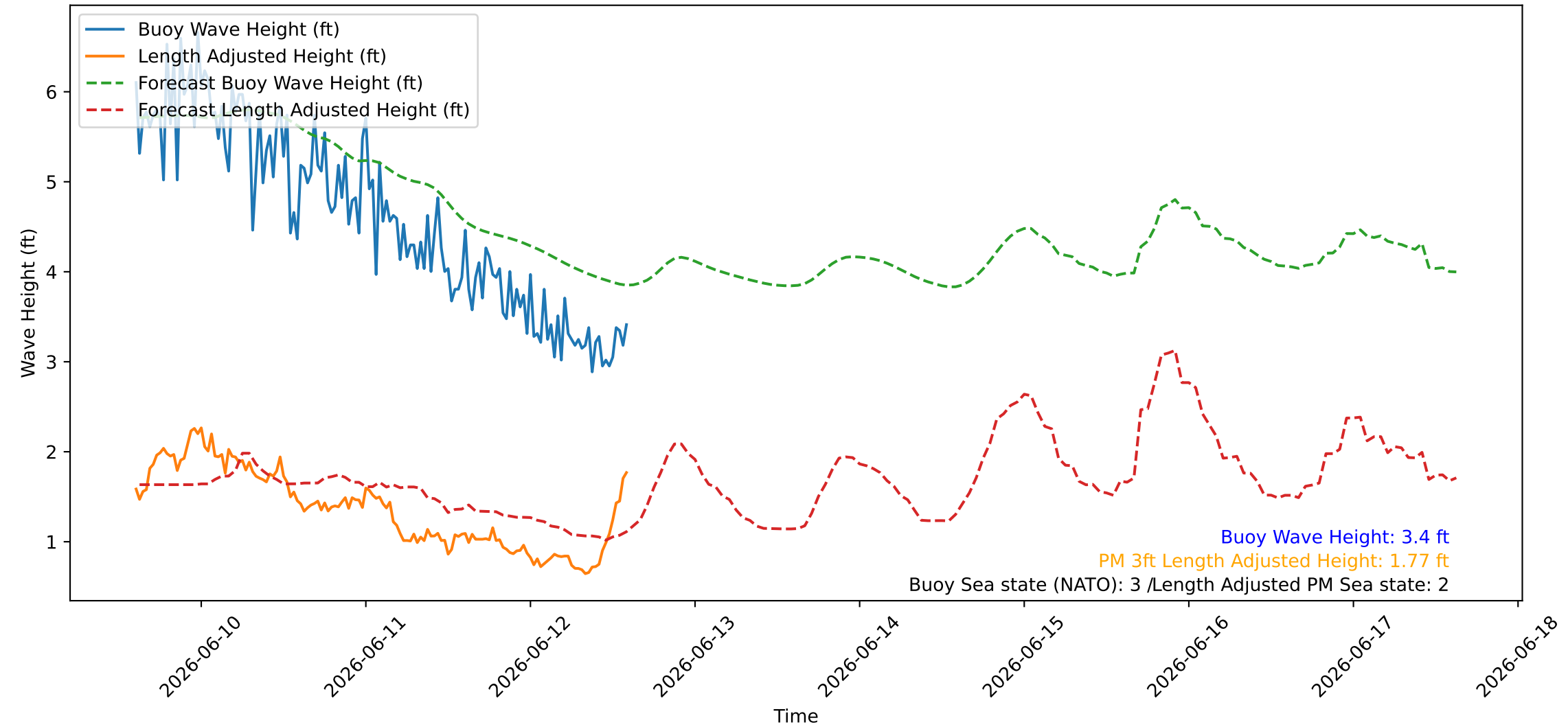
Wave Heights over Time for Green Beach at 2026-06-12 14:41:08
