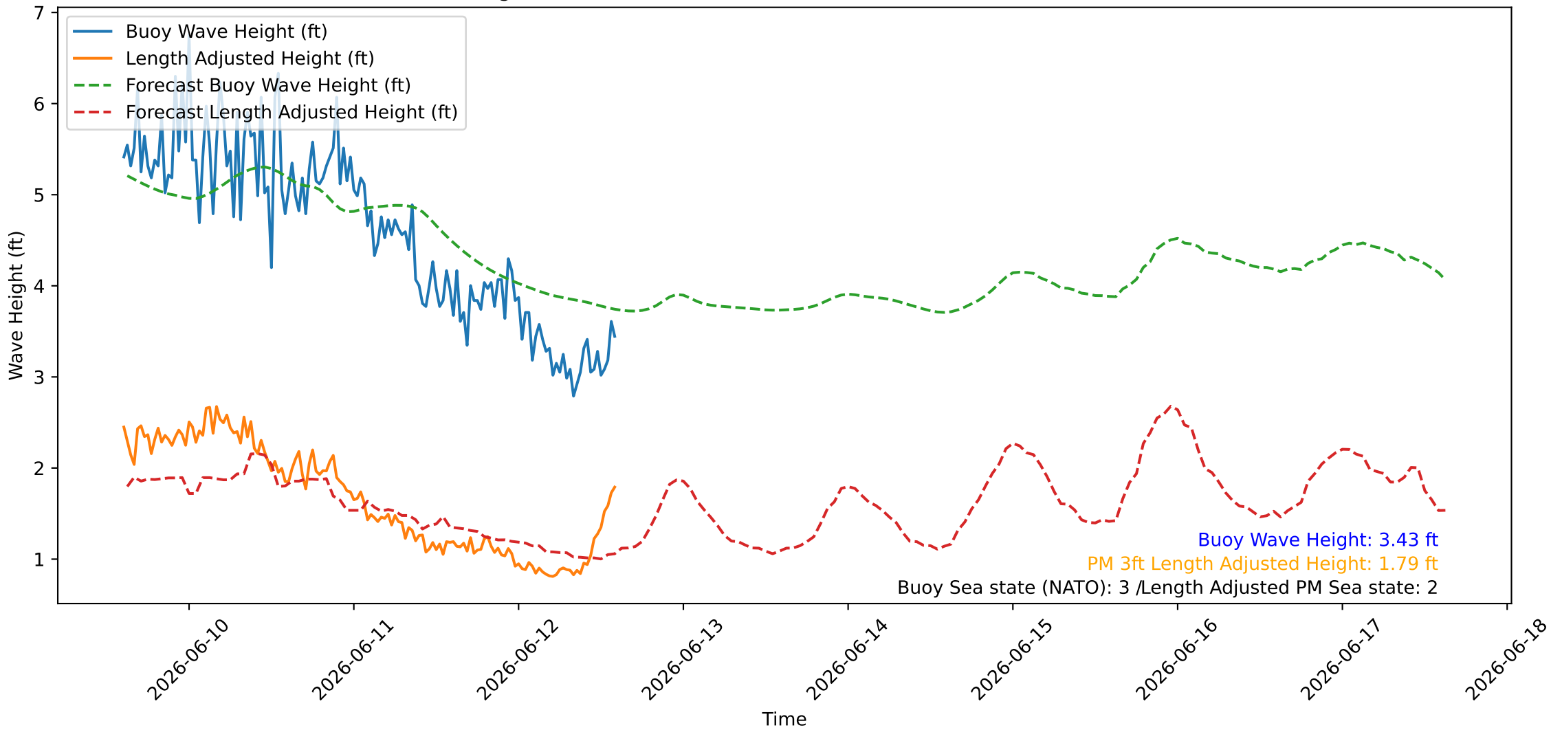
Wave Heights over Time for Oceanside Harbor at 2026-06-12 14:40:26
