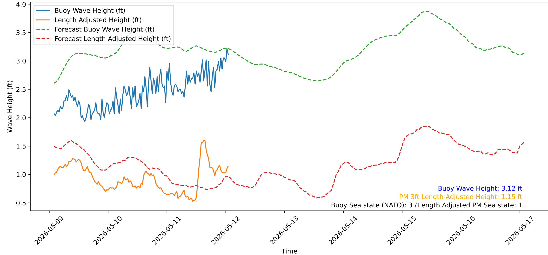
Wave Heights over Time for Red Beach at 2026-05-12 01:50:51
