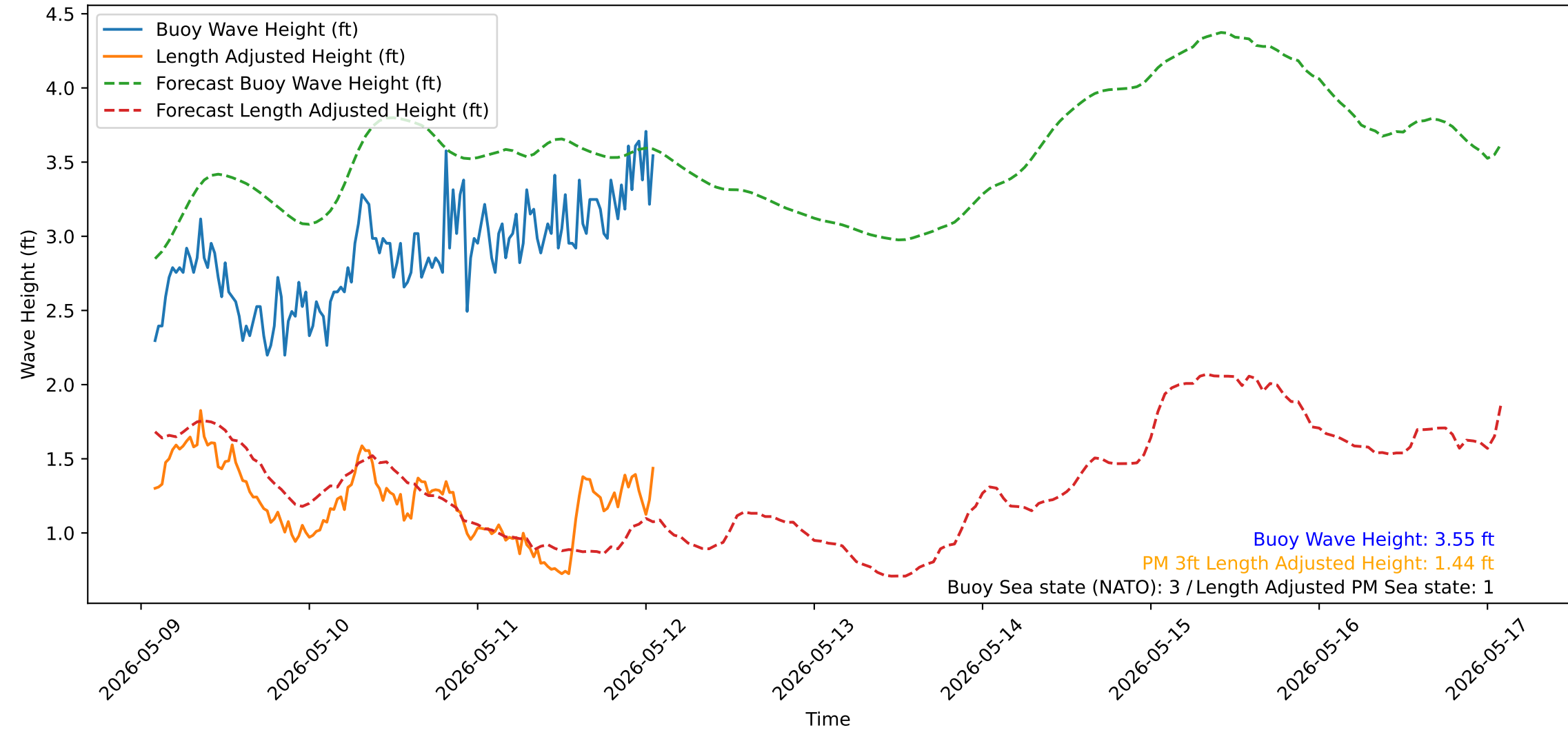
Wave Heights over Time for Oceanside Harbor at 2026-05-12 01:50:31
