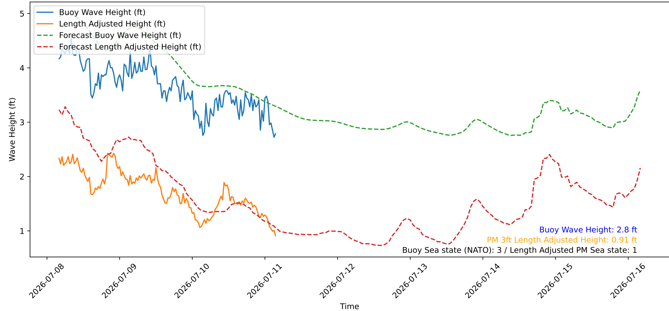
Wave Heights over Time for Green Beach at 2026-07-11 04:11:09
