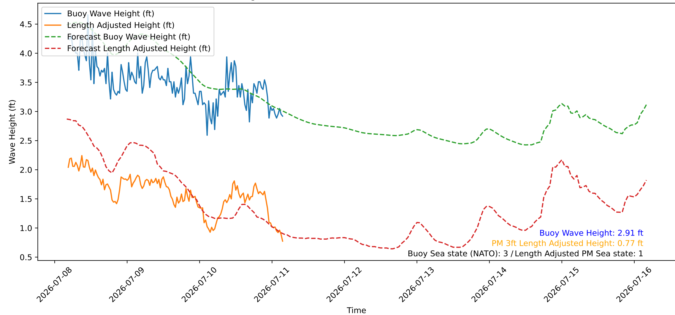
Wave Heights over Time for Red Beach at 2026-07-11 04:10:46
