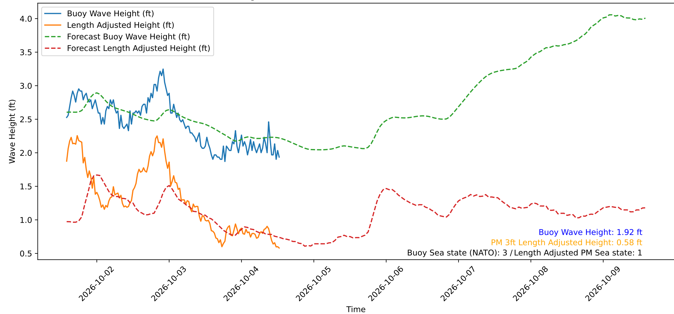
Wave Heights over Time for Red Beach at 2026-10-04 13:30:49
