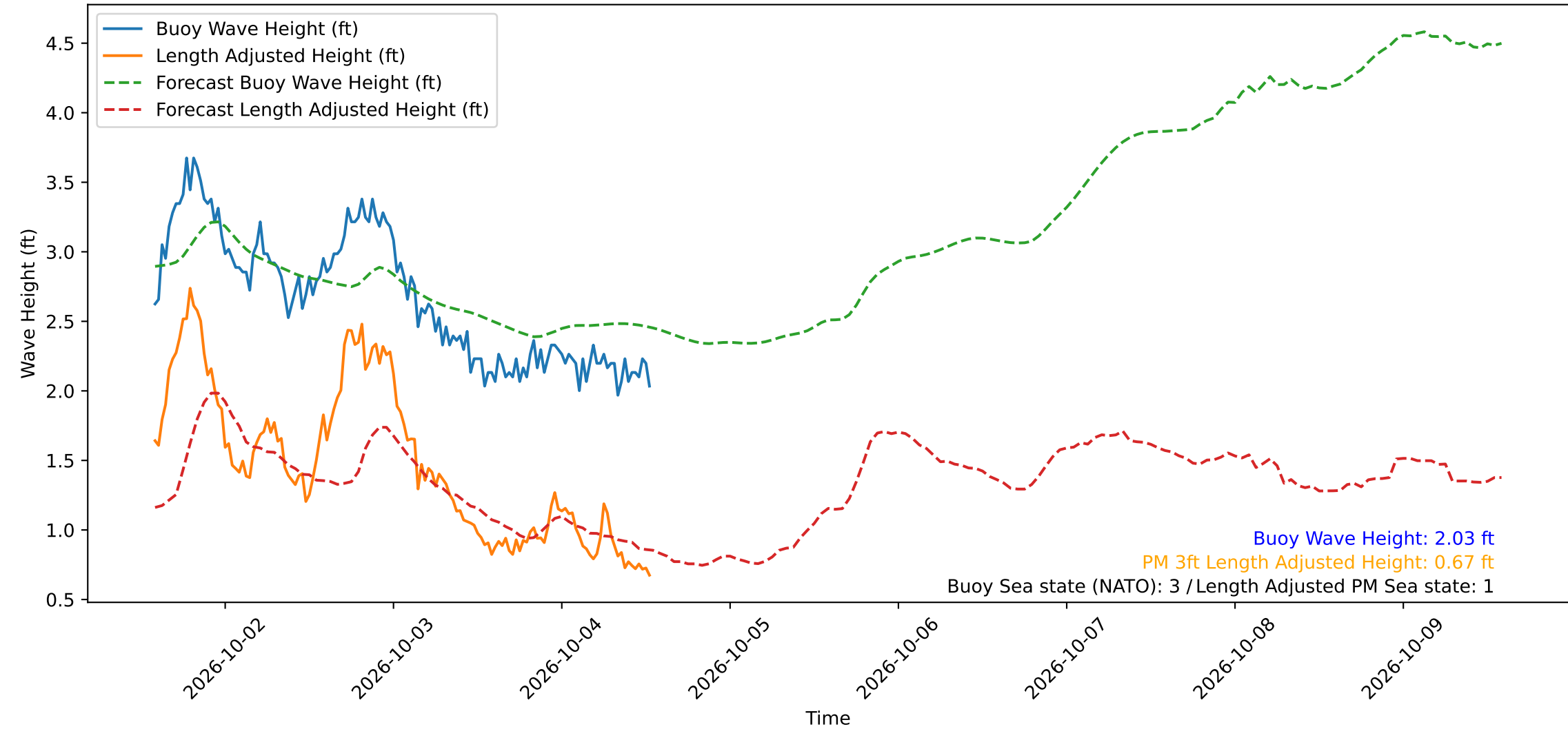
Wave Heights over Time for Green Beach at 2026-10-04 13:31:12
