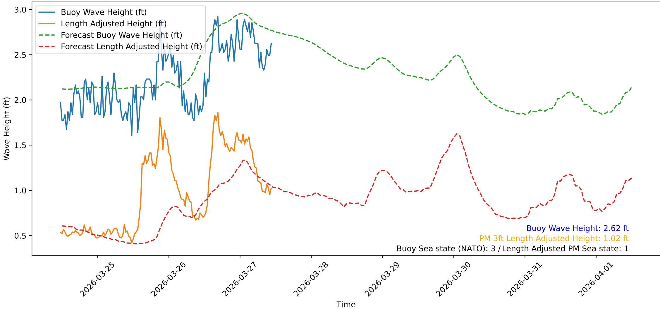
Wave Heights over Time for Oceanside Harbor at 2026-03-27 11:30:32
