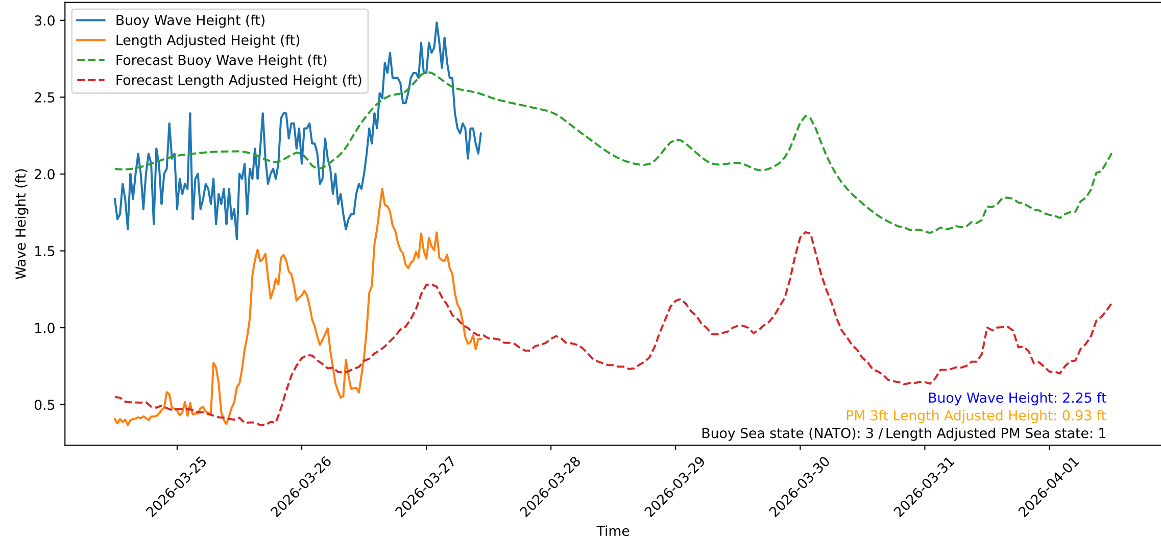
Wave Heights over Time for Red Beach at 2026-03-27 11:30:47
