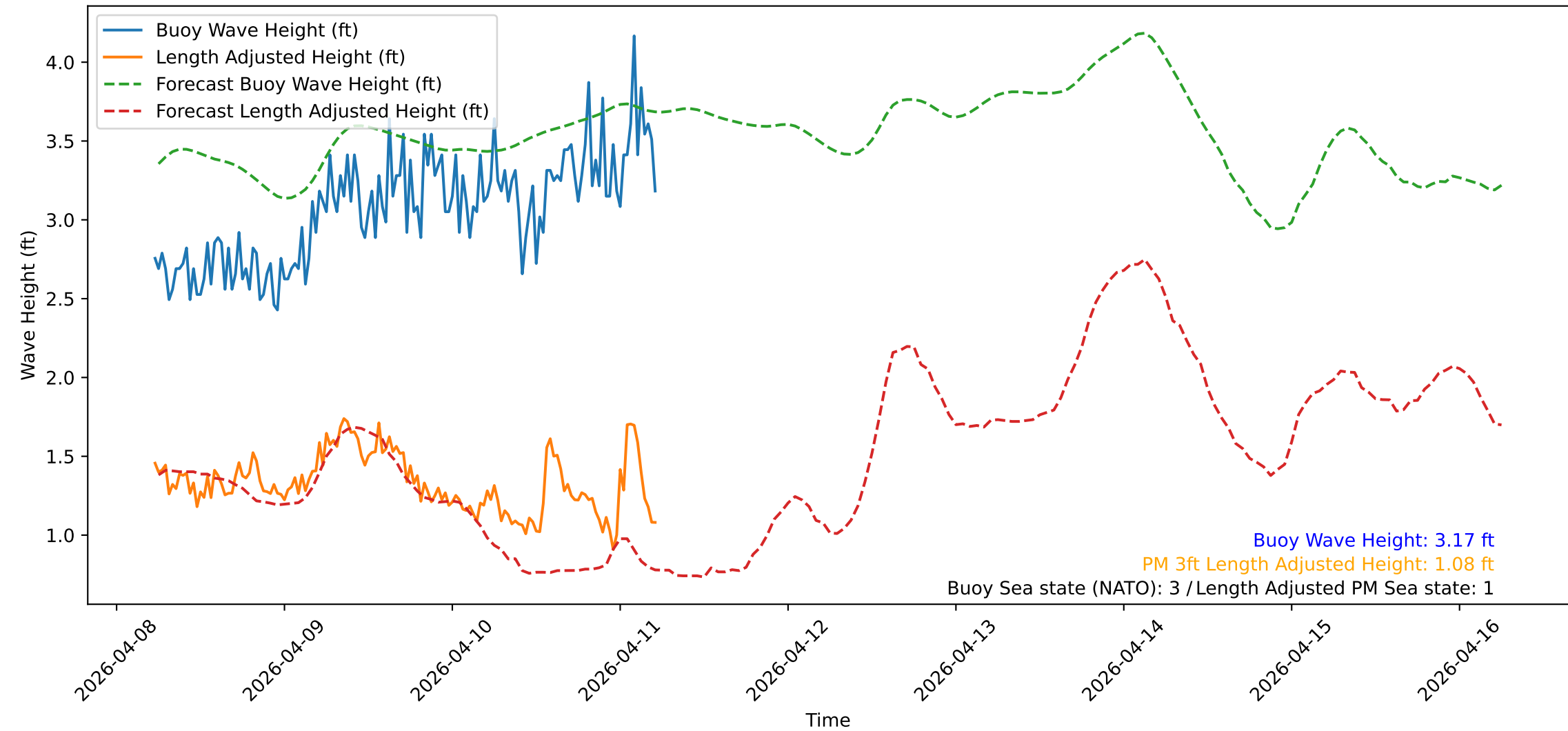
Wave Heights over Time for Oceanside Harbor at 2026-04-11 05:40:31
