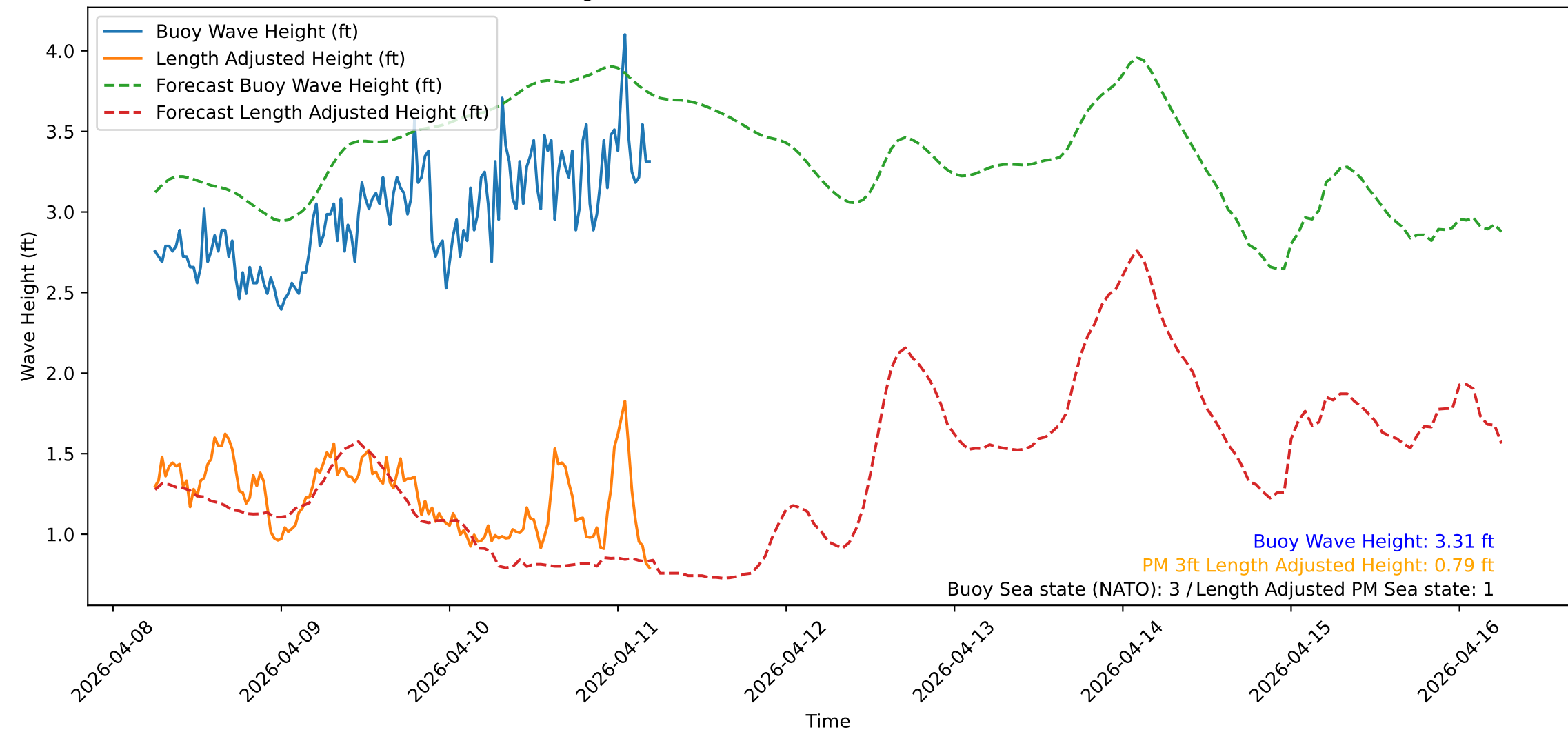
Wave Heights over Time for Red Beach at 2026-04-11 05:40:50
