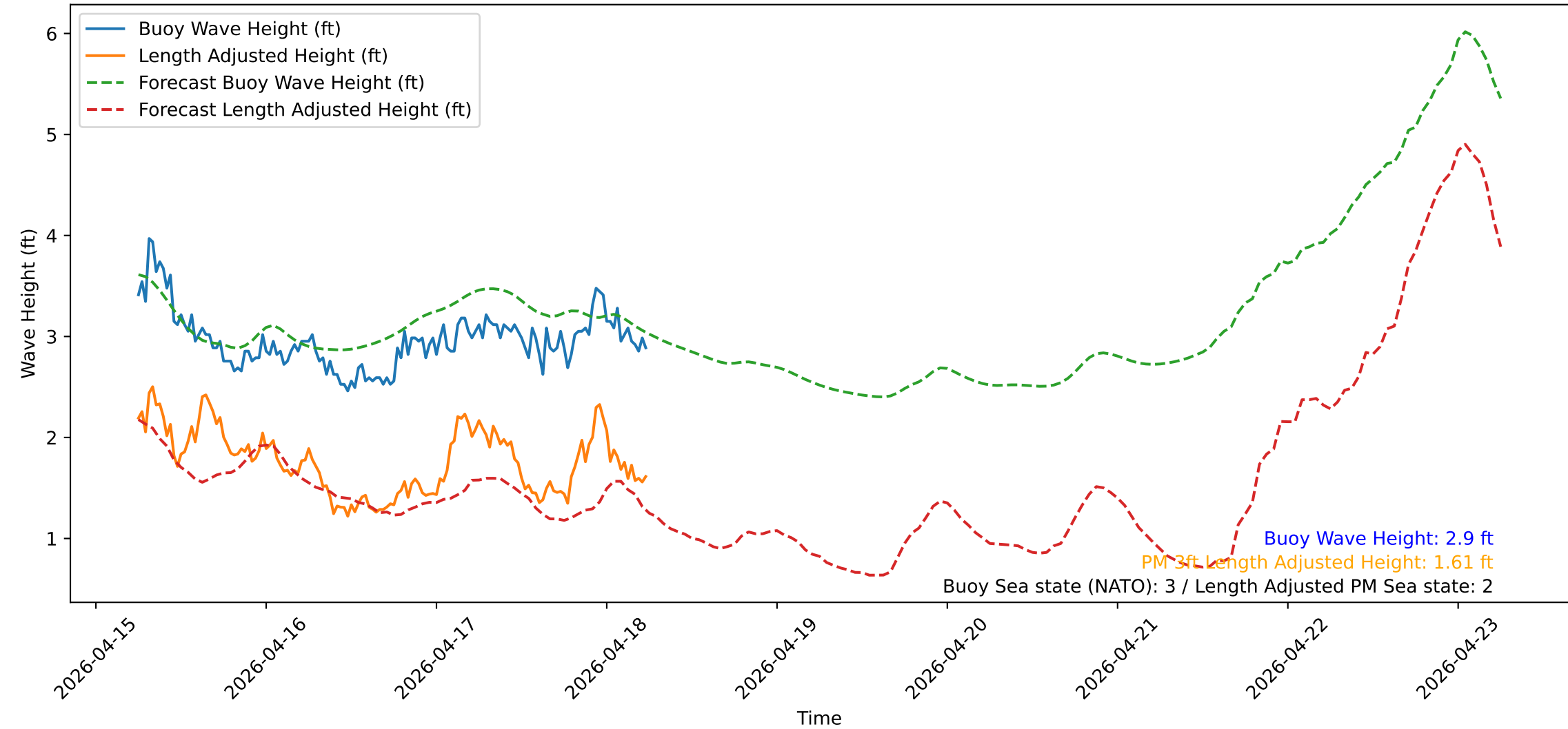
Wave Heights over Time for Green Beach at 2026-04-18 06:11:11
