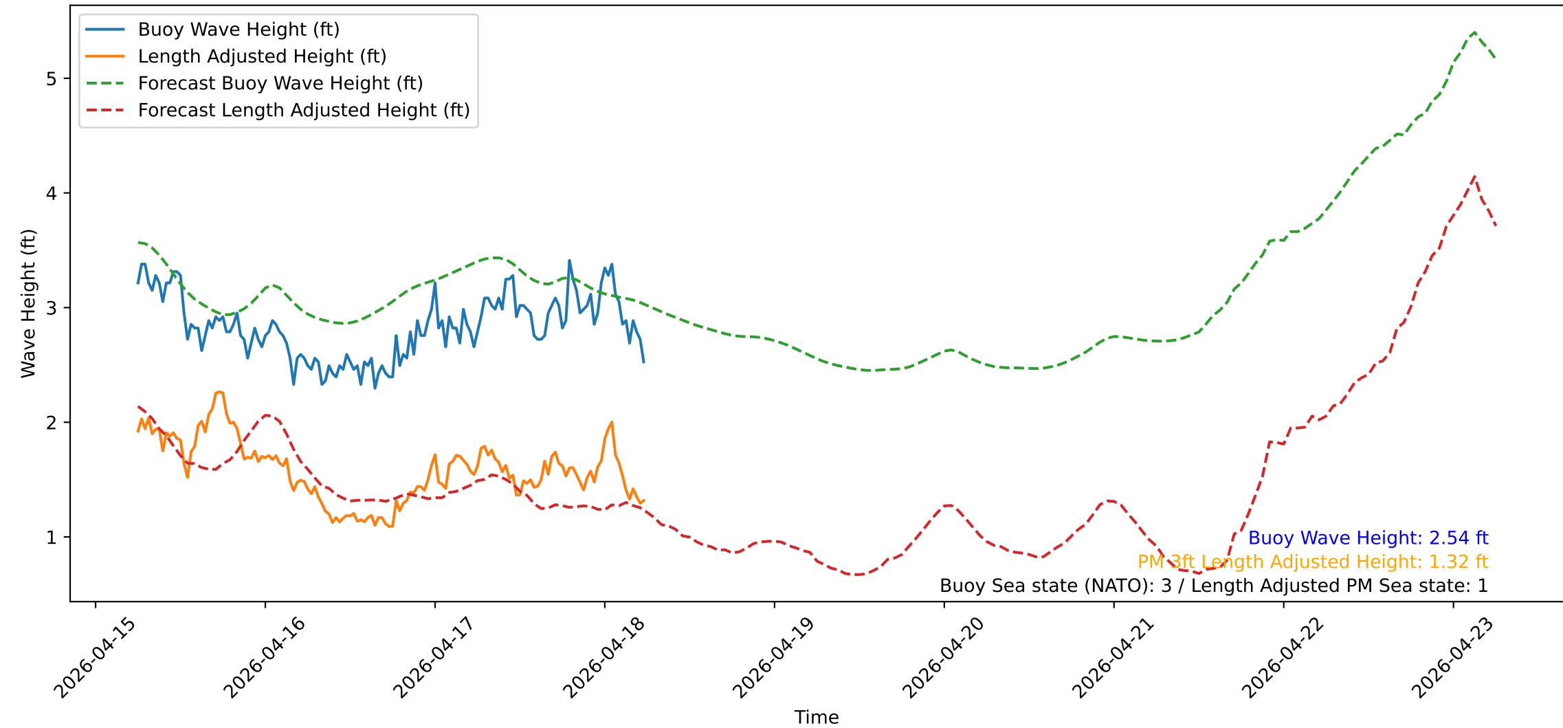
Wave Heights over Time for Oceanside Harbor at 2026-04-18 06:10:31
