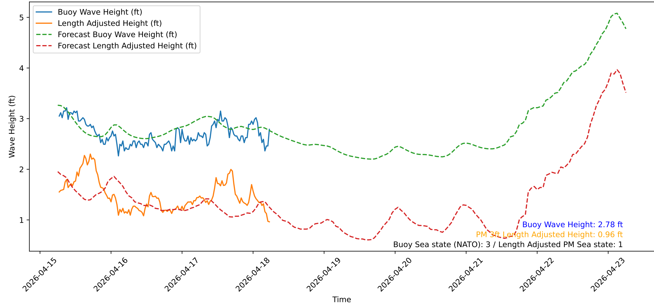
Wave Heights over Time for Red Beach at 2026-04-18 06:10:49
