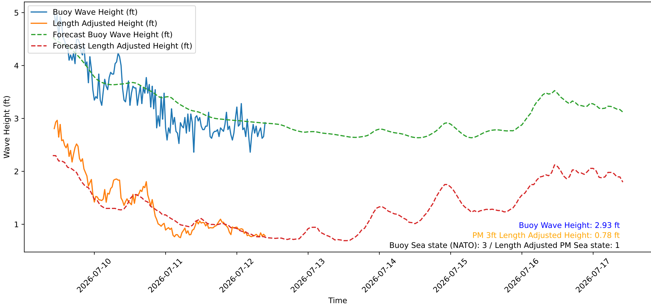
Wave Heights over Time for Oceanside Harbor at 2026-07-12 10:20:26
