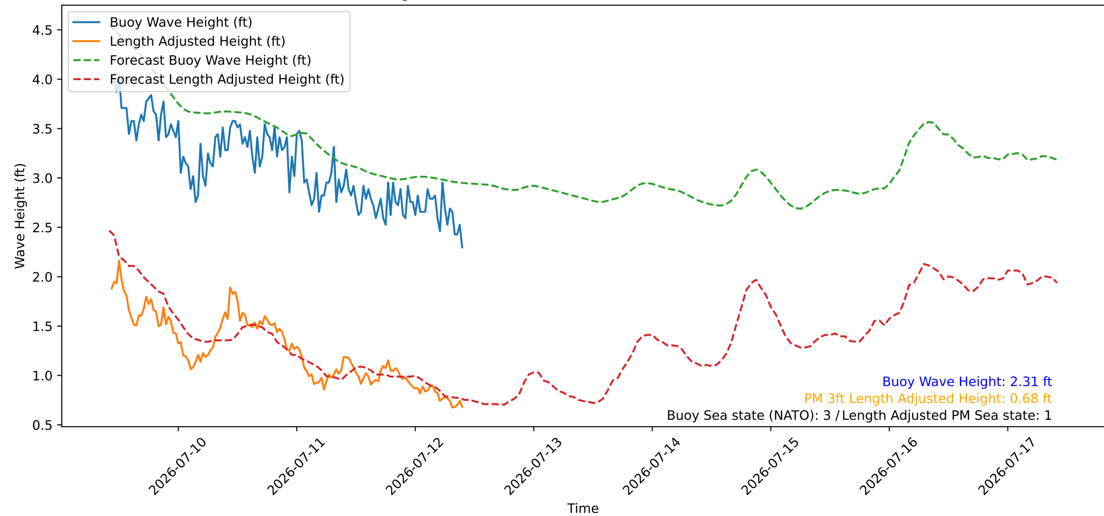
Wave Heights over Time for Green Beach at 2026-07-12 10:21:10
