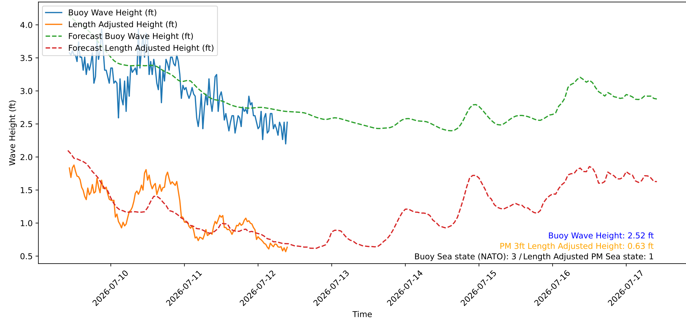
Wave Heights over Time for Red Beach at 2026-07-12 10:20:47
