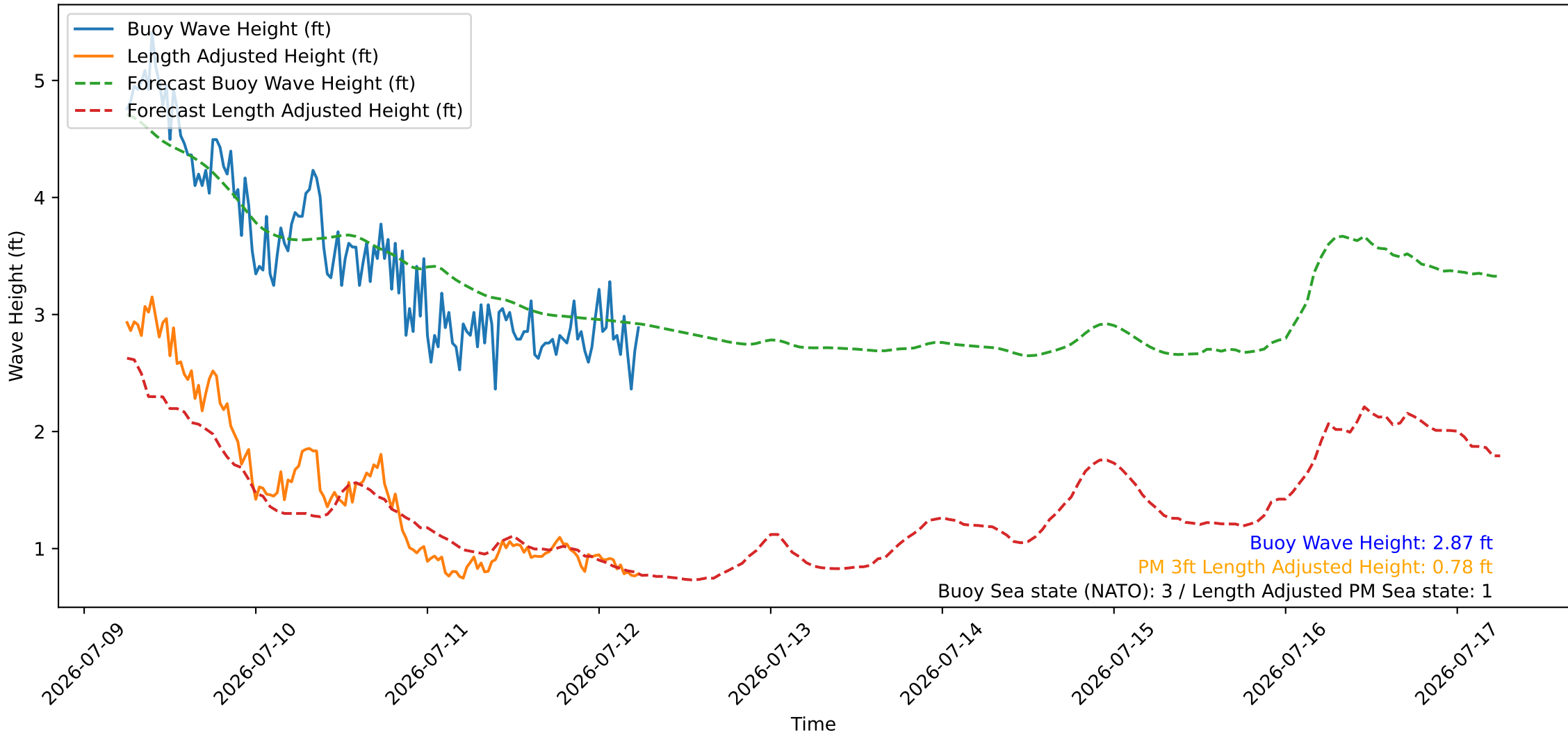
Wave Heights over Time for Oceanside Harbor at 2026-07-12 06:00:26
