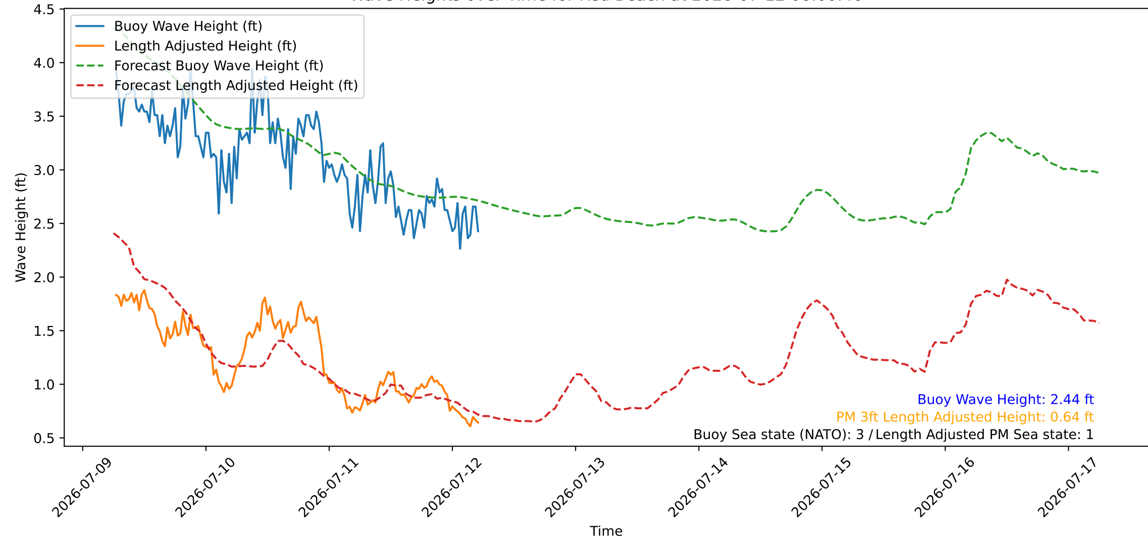
Wave Heights over Time for Red Beach at 2026-07-12 06:00:46
