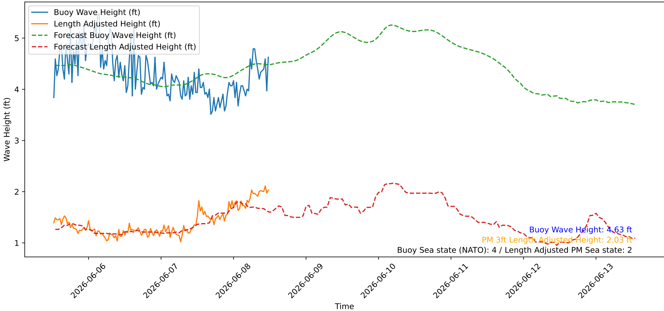
Wave Heights over Time for Oceanside Harbor at 2026-06-08 12:30:25
