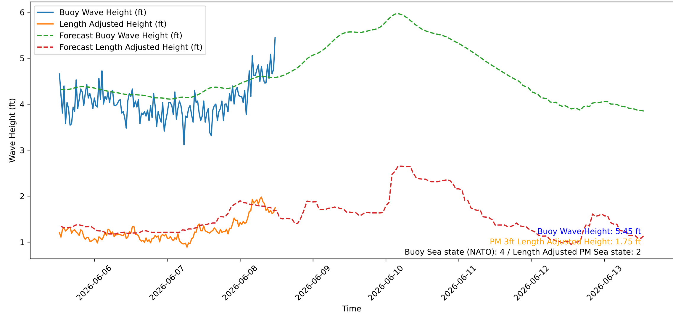
Wave Heights over Time for Green Beach at 2026-06-08 12:31:08
