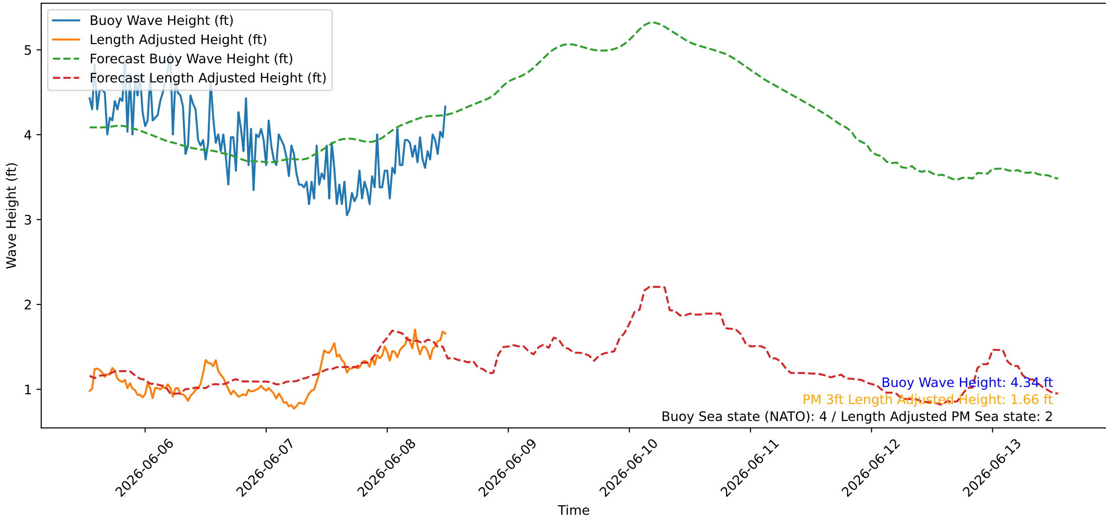
Wave Heights over Time for Red Beach at 2026-06-08 12:30:45
