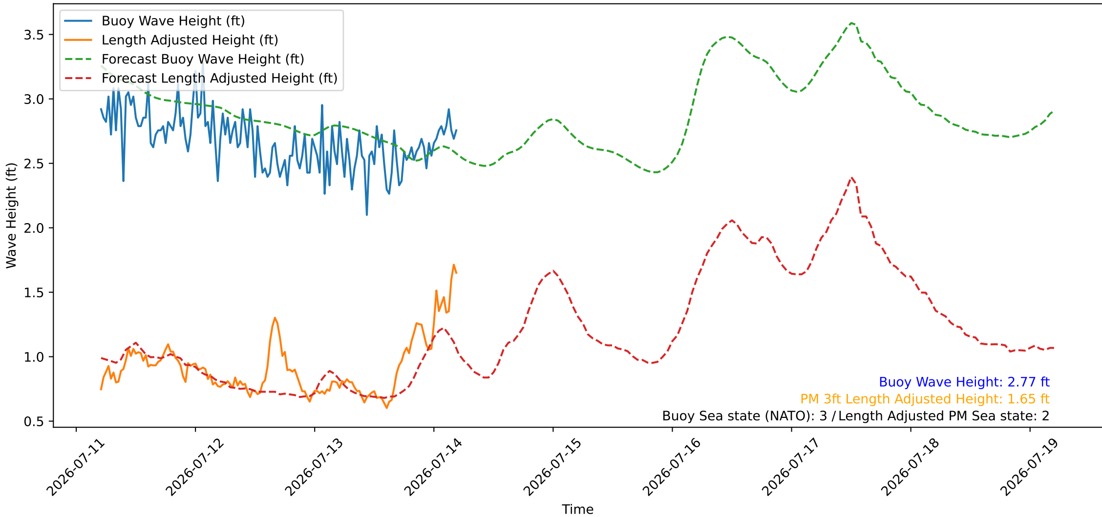
Wave Heights over Time for Oceanside Harbor at 2026-07-14 05:10:27
