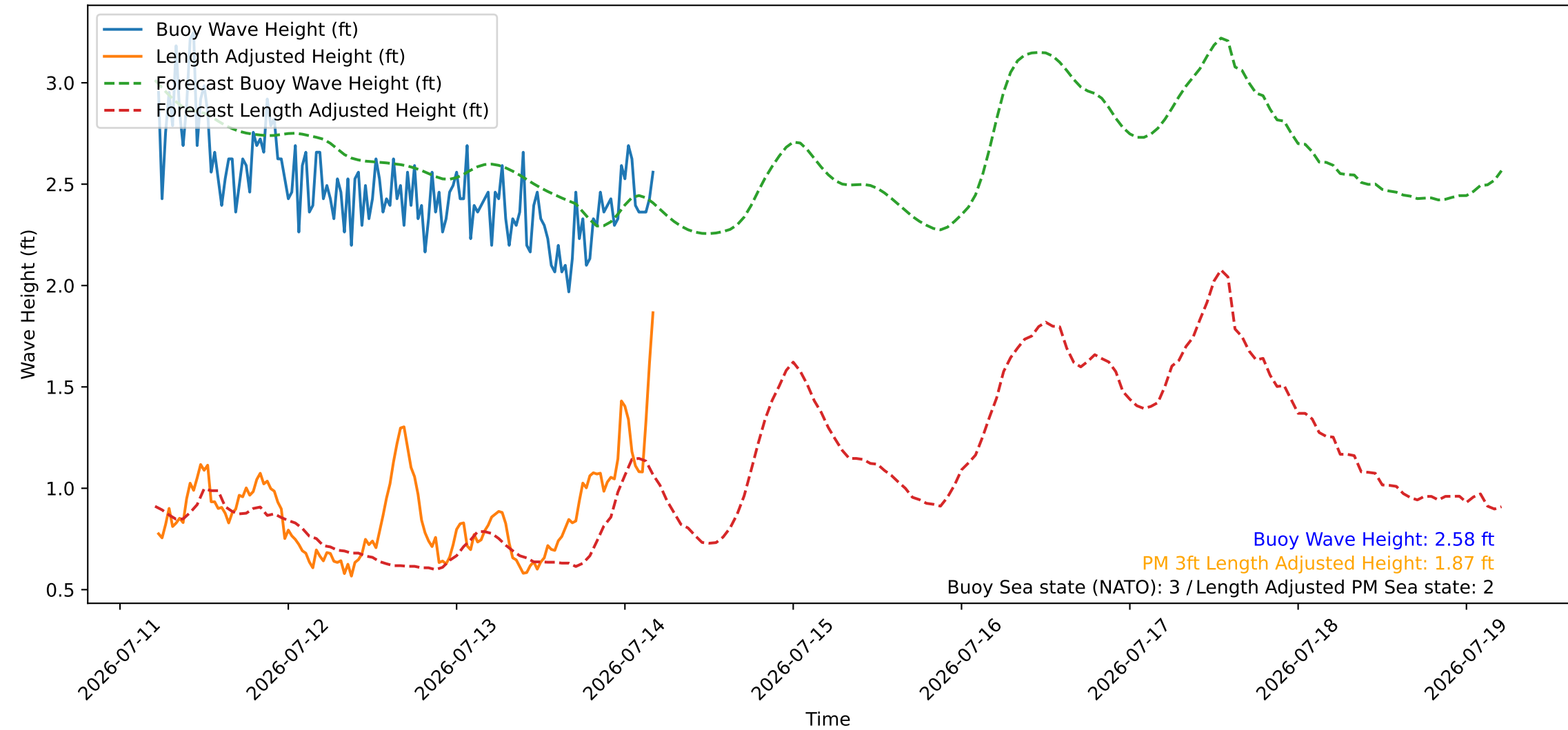
Wave Heights over Time for Red Beach at 2026-07-14 05:10:46
