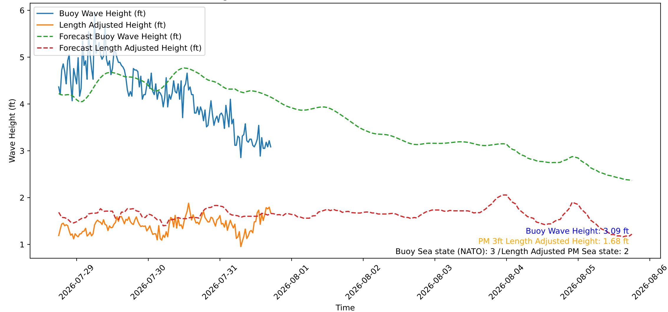
Wave Heights over Time for Oceanside Harbor at 2026-07-31 18:10:26
