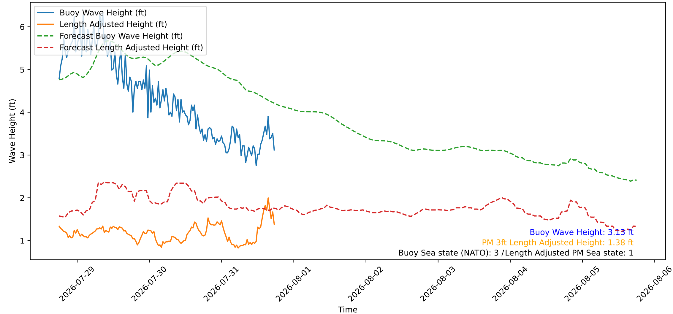
Wave Heights over Time for Green Beach at 2026-07-31 18:11:09
