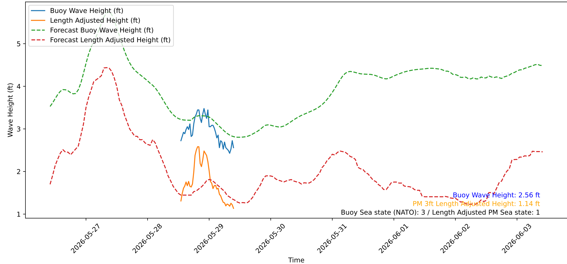
Wave Heights over Time for Oceanside Harbor at 2026-05-29 10:20:21
