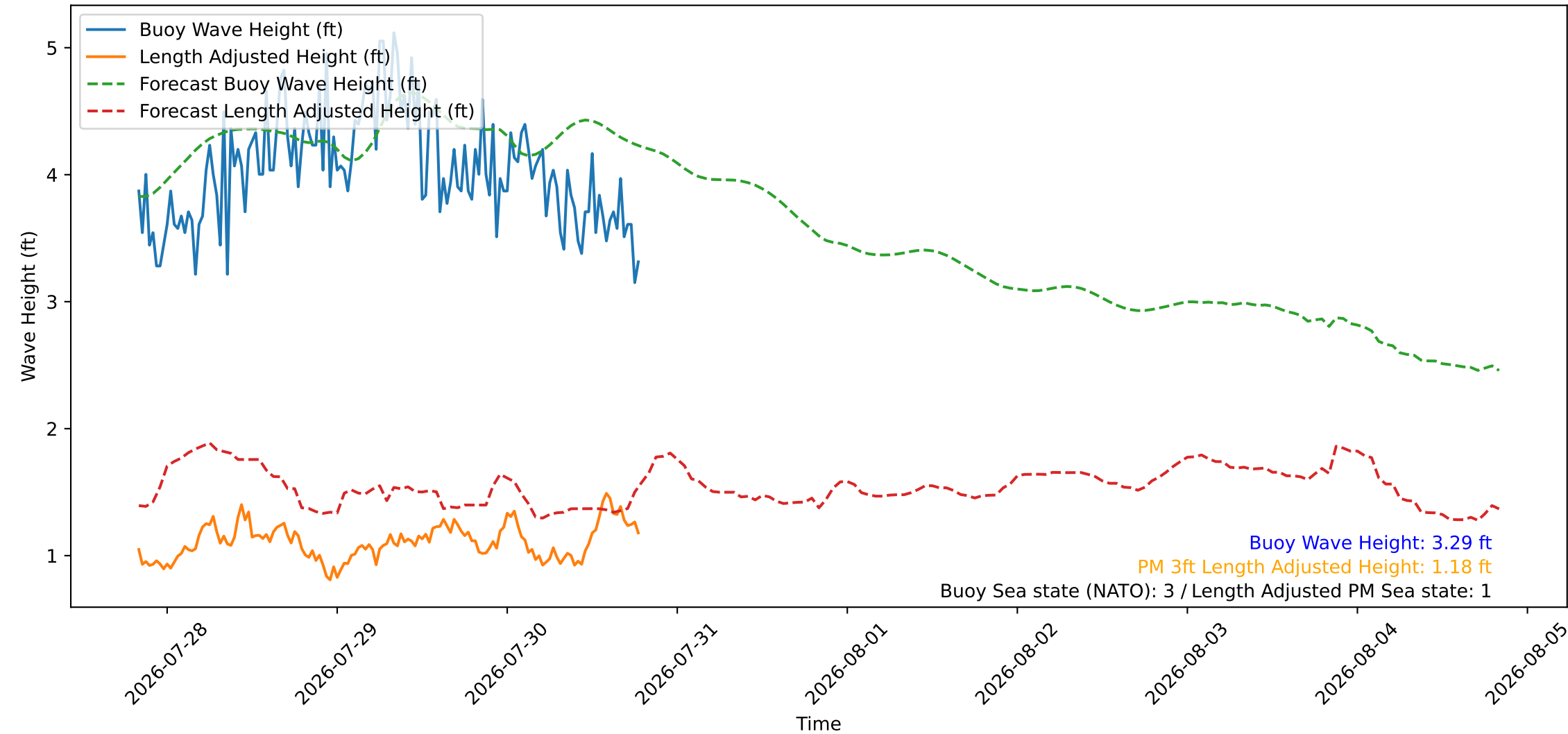
Wave Heights over Time for Red Beach at 2026-07-30 19:30:46
