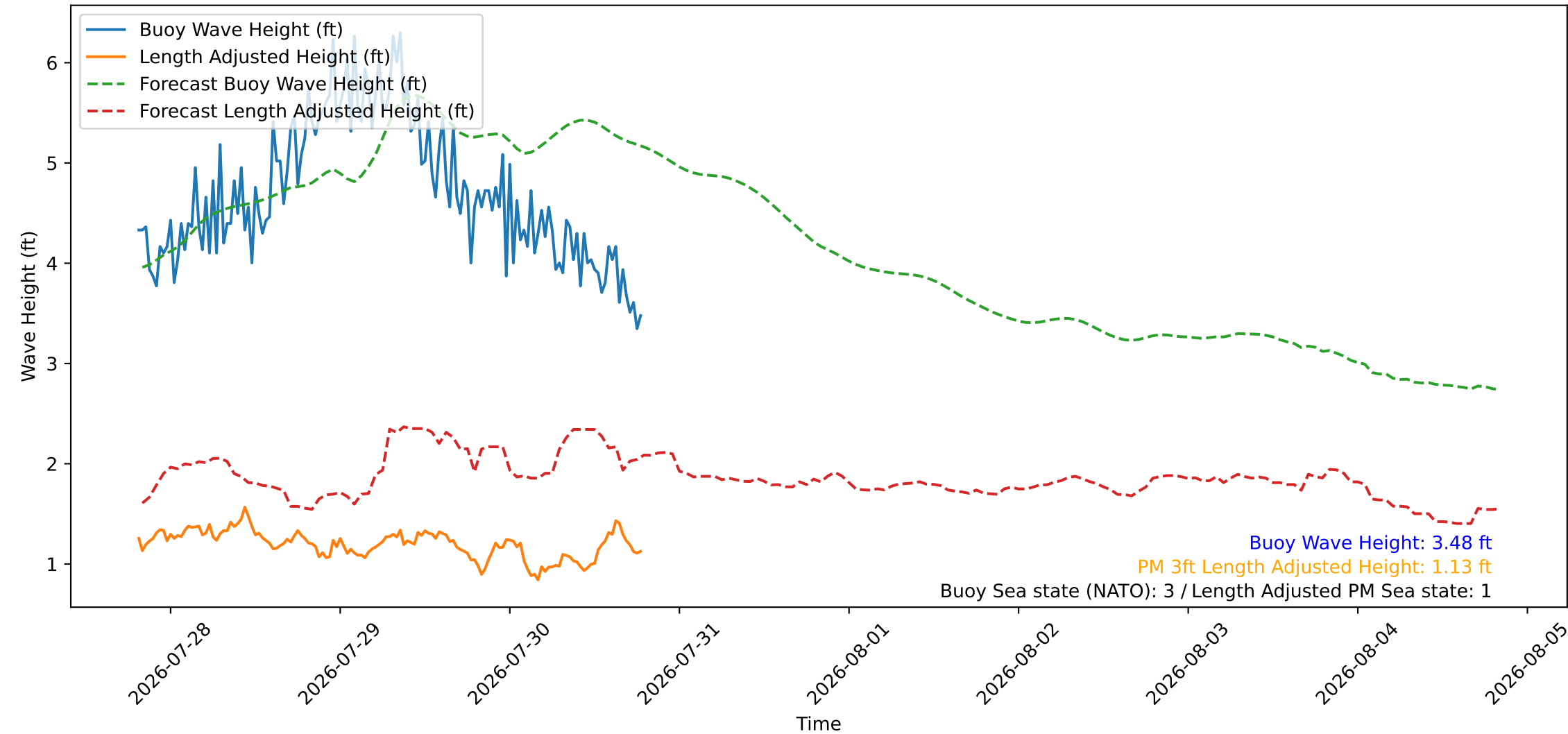
Wave Heights over Time for Green Beach at 2026-07-30 19:31:08
