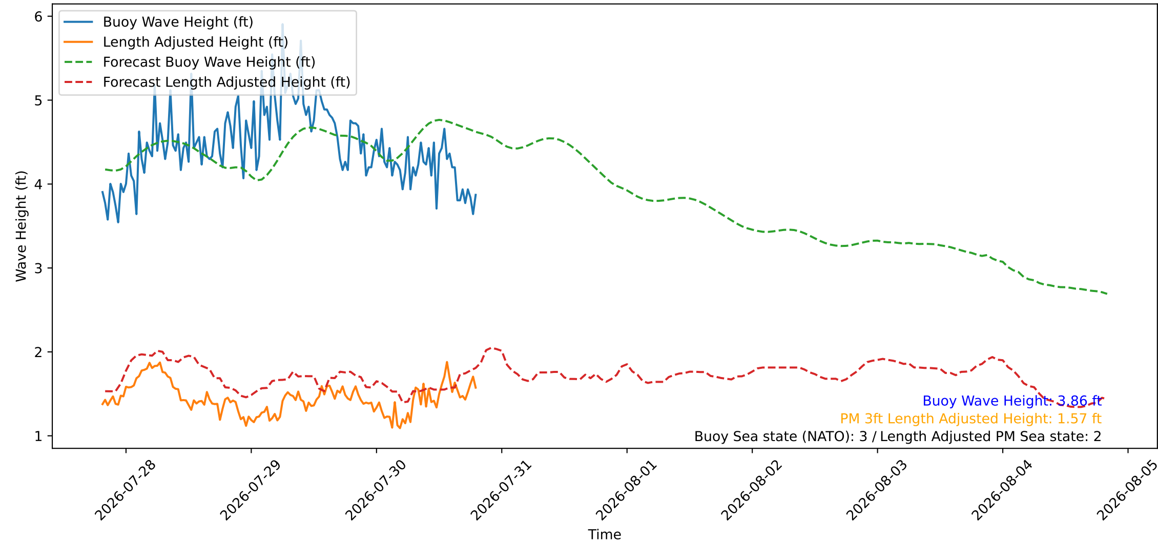
Wave Heights over Time for Oceanside Harbor at 2026-07-30 19:30:26
