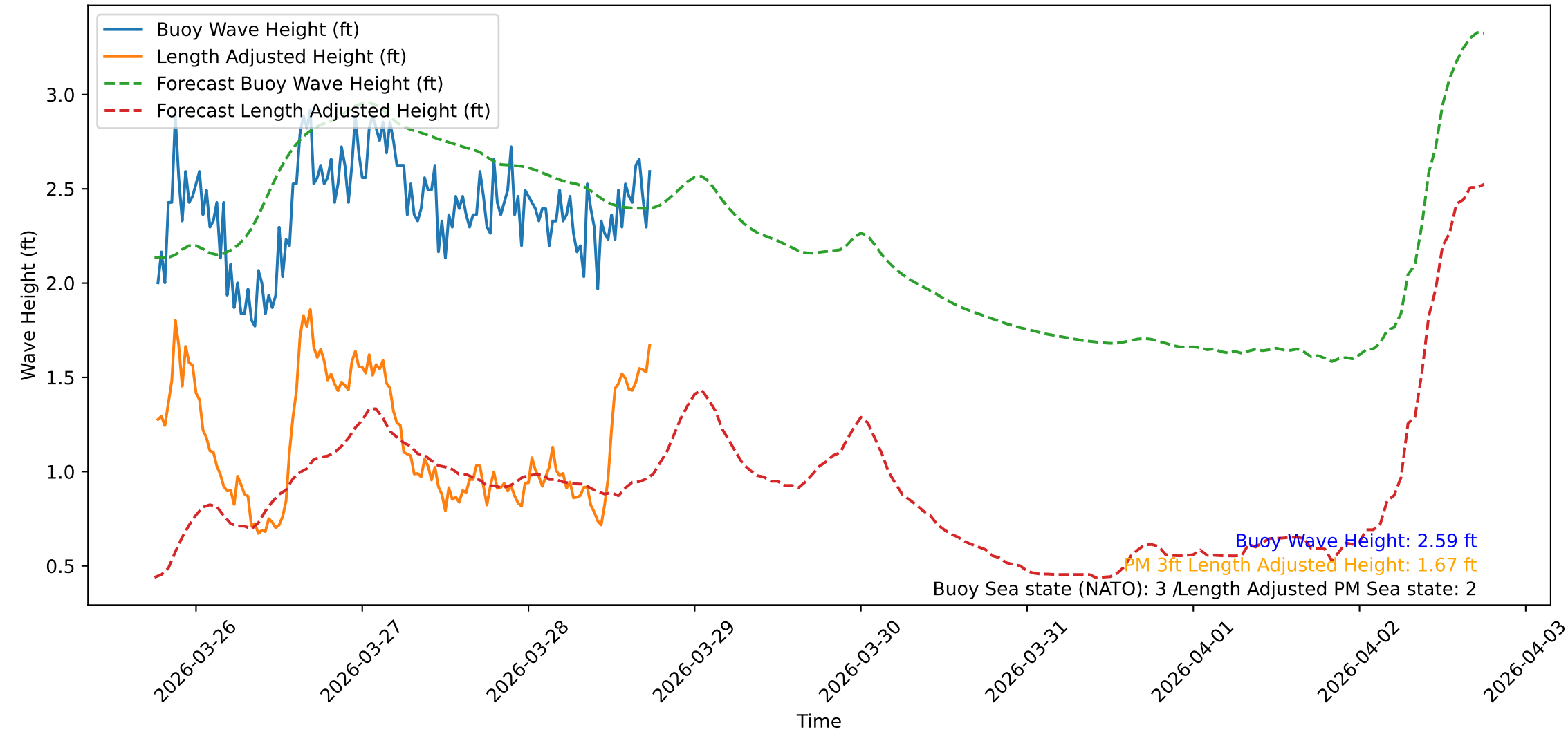
Wave Heights over Time for Oceanside Harbor at 2026-03-28 18:20:32
