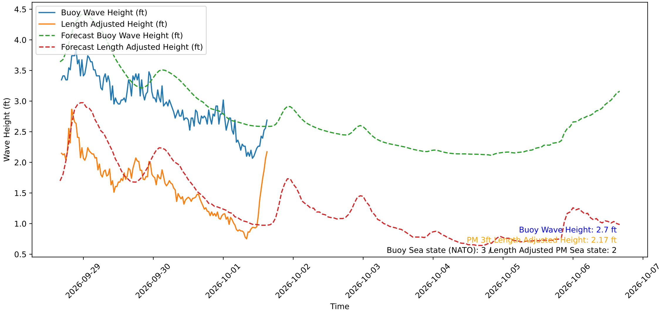
Wave Heights over Time for Red Beach at 2026-10-01 16:00:49
