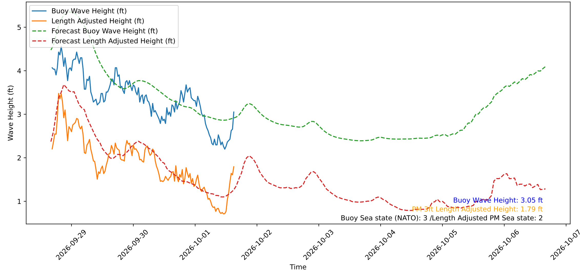
Wave Heights over Time for Green Beach at 2026-10-01 16:01:11
