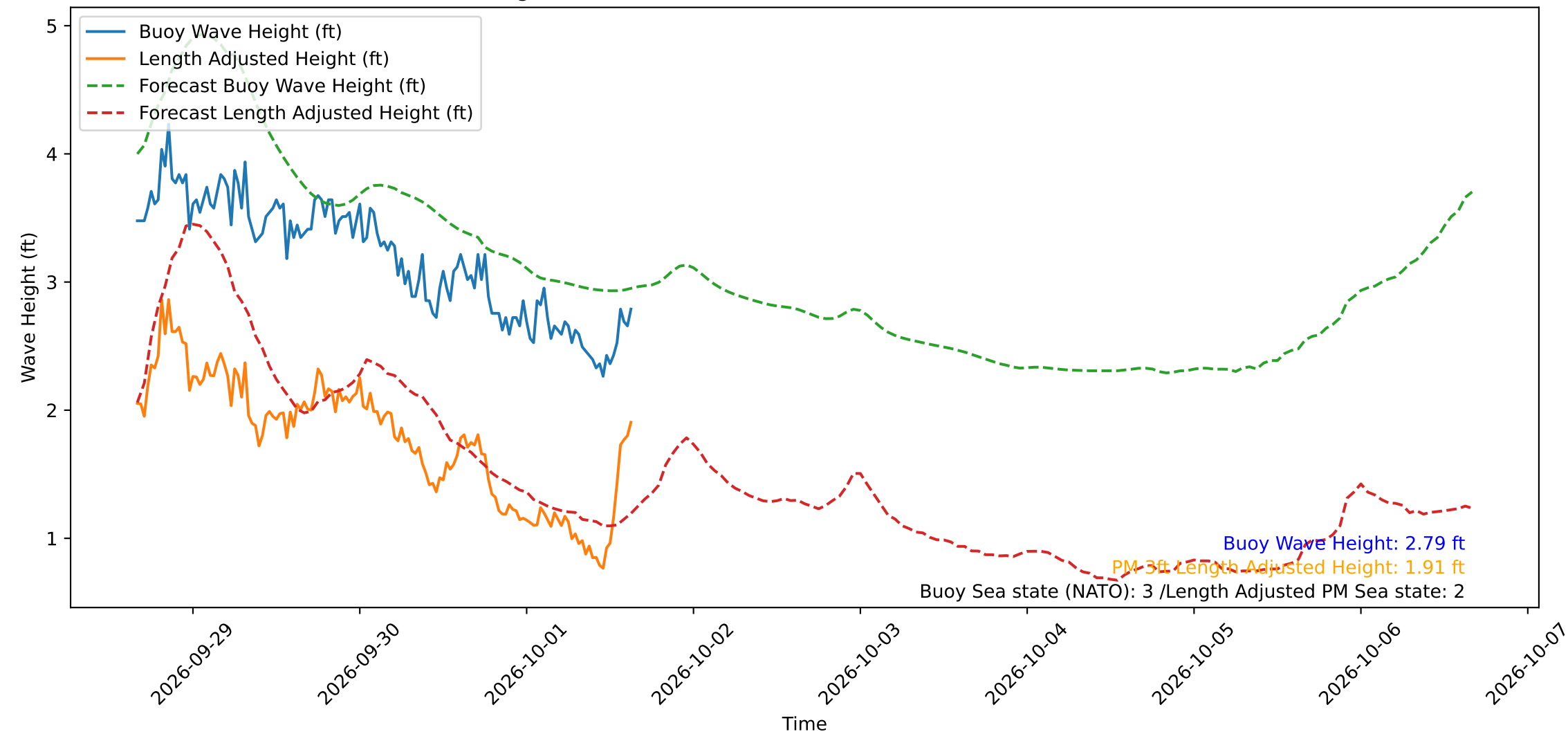
Wave Heights over Time for Oceanside Harbor at 2026-10-01 16:00:29
