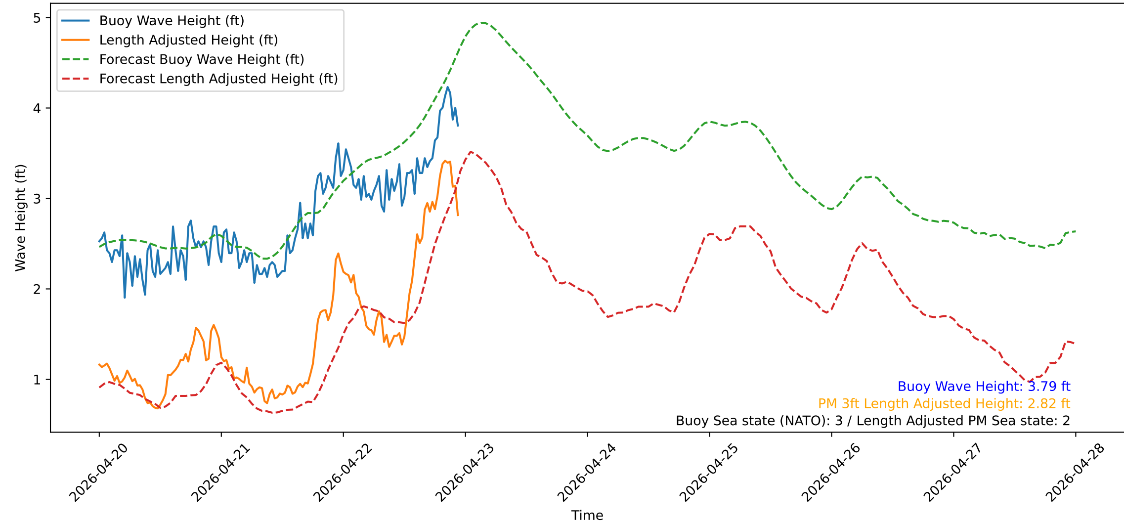
Wave Heights over Time for Oceanside Harbor at 2026-04-22 23:50:31
