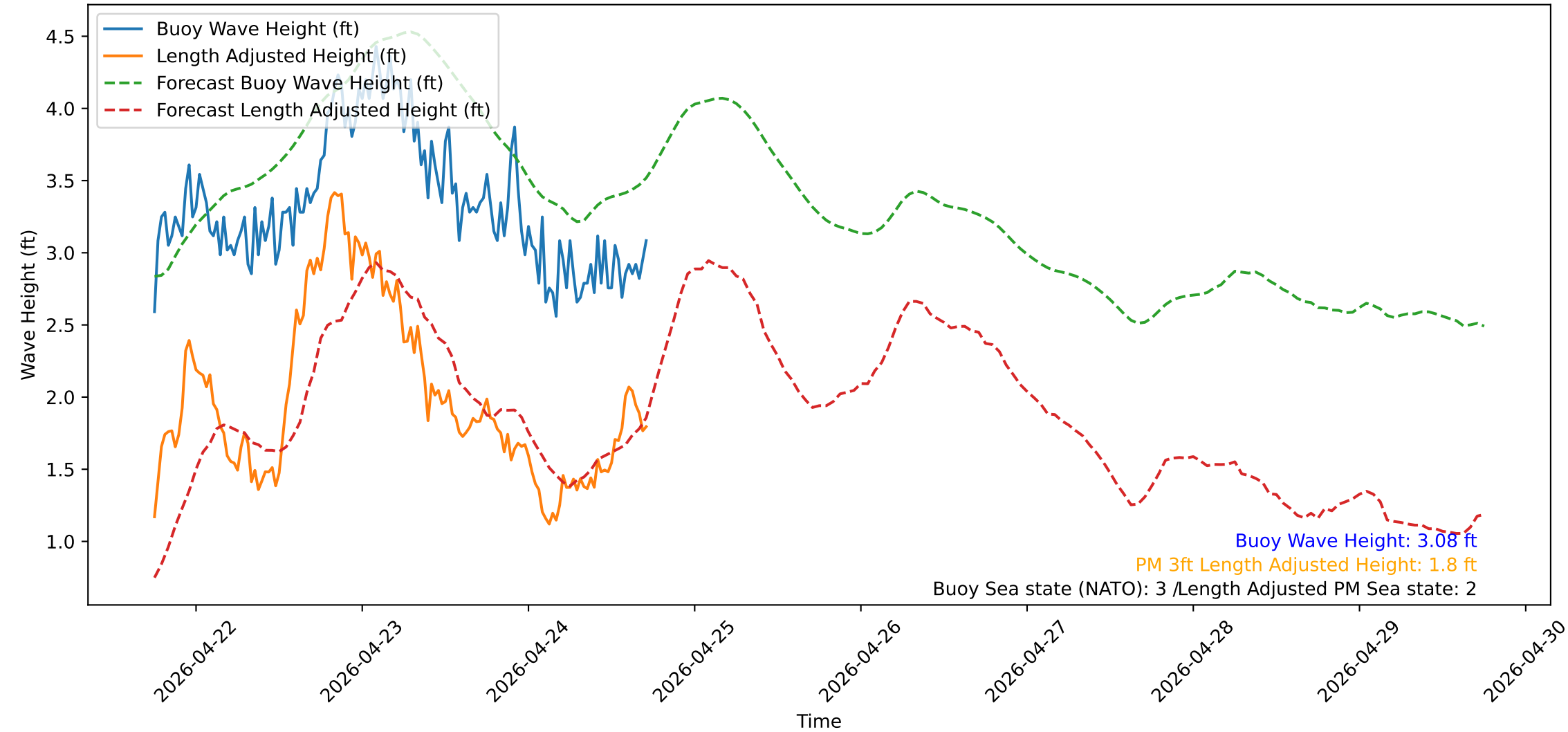
Wave Heights over Time for Oceanside Harbor at 2026-04-24 17:50:31
