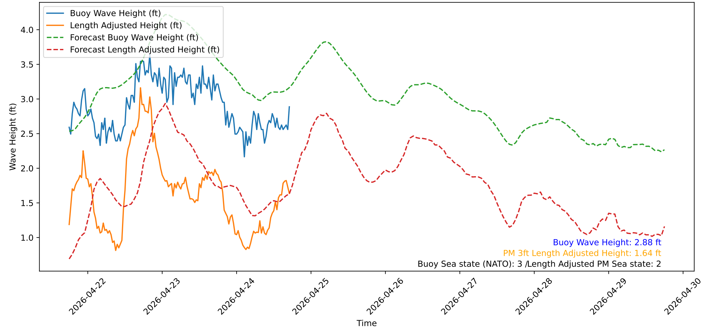
Wave Heights over Time for Red Beach at 2026-04-24 17:50:51
