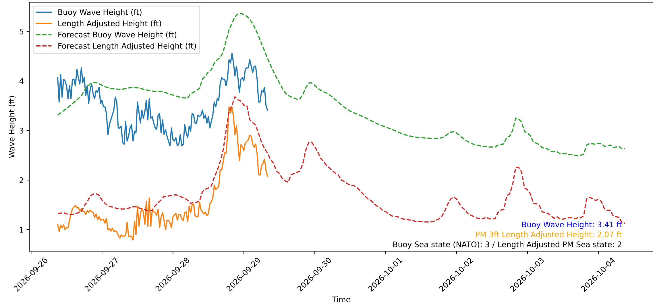
Wave Heights over Time for Green Beach at 2026-09-29 08:41:12
