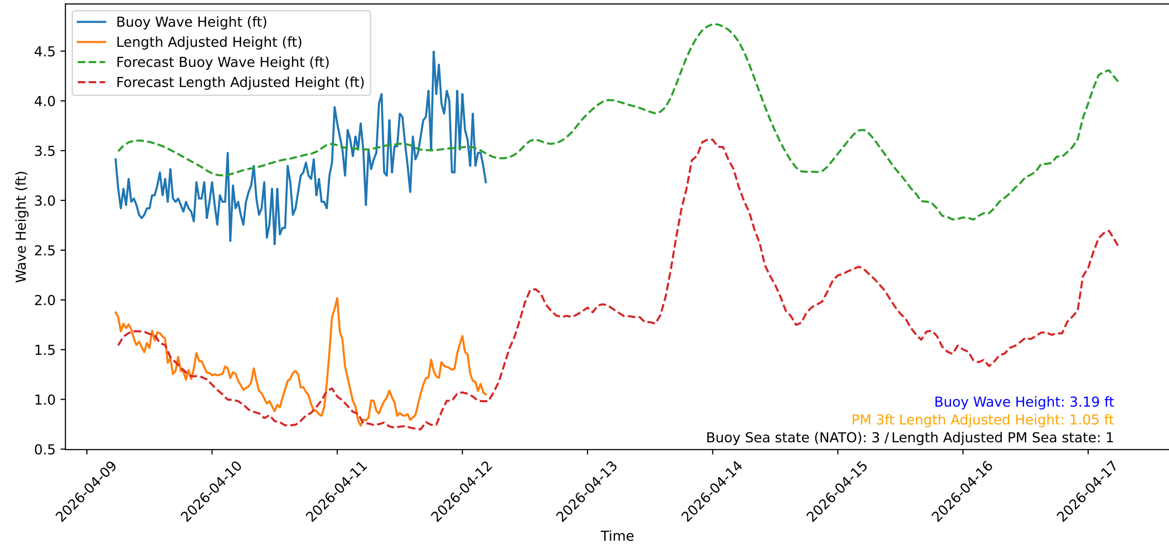
Wave Heights over Time for Green Beach at 2026-04-12 05:31:12
