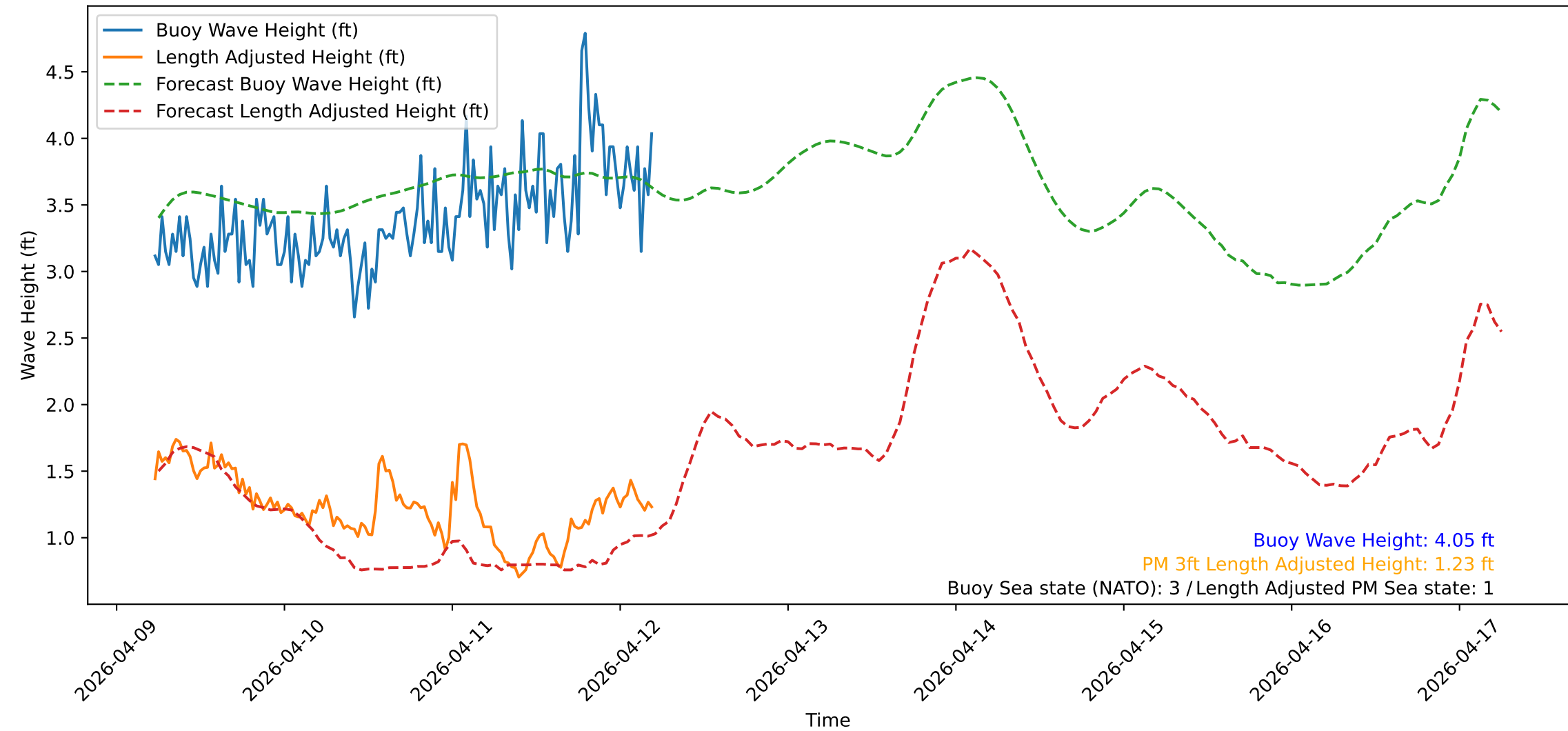
Wave Heights over Time for Oceanside Harbor at 2026-04-12 05:30:31
