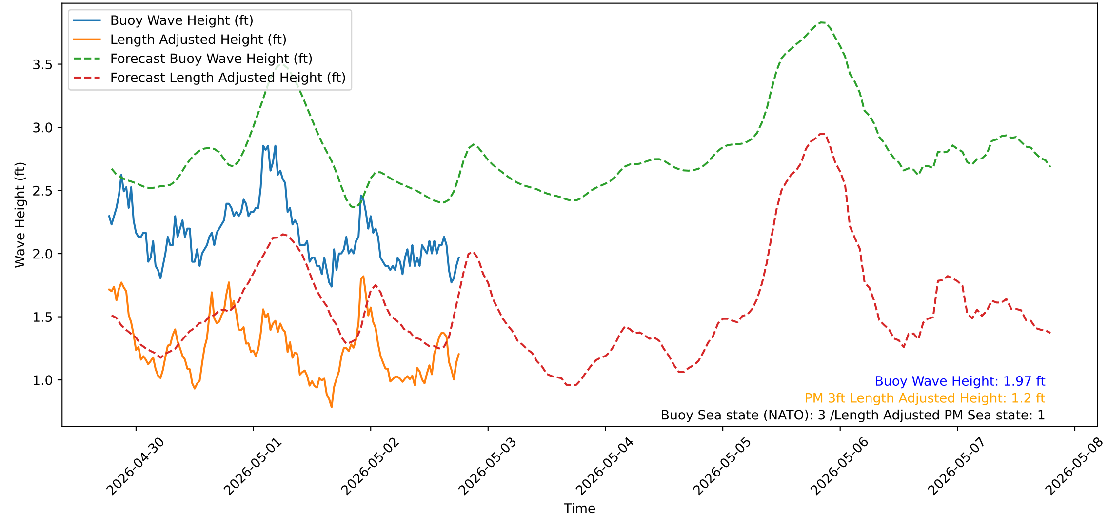
Wave Heights over Time for Green Beach at 2026-05-02 18:41:14
