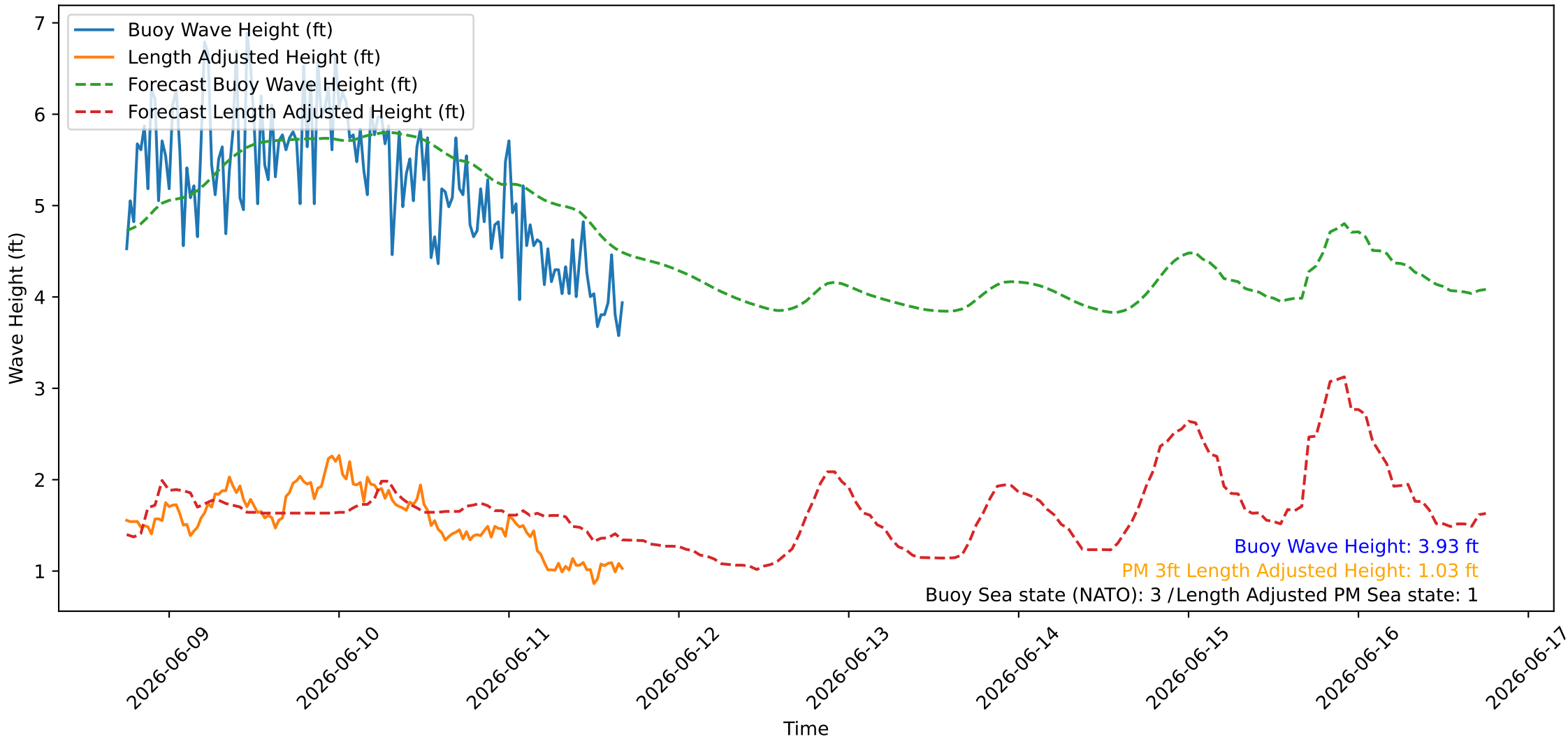
Wave Heights over Time for Green Beach at 2026-06-11 17:51:10
