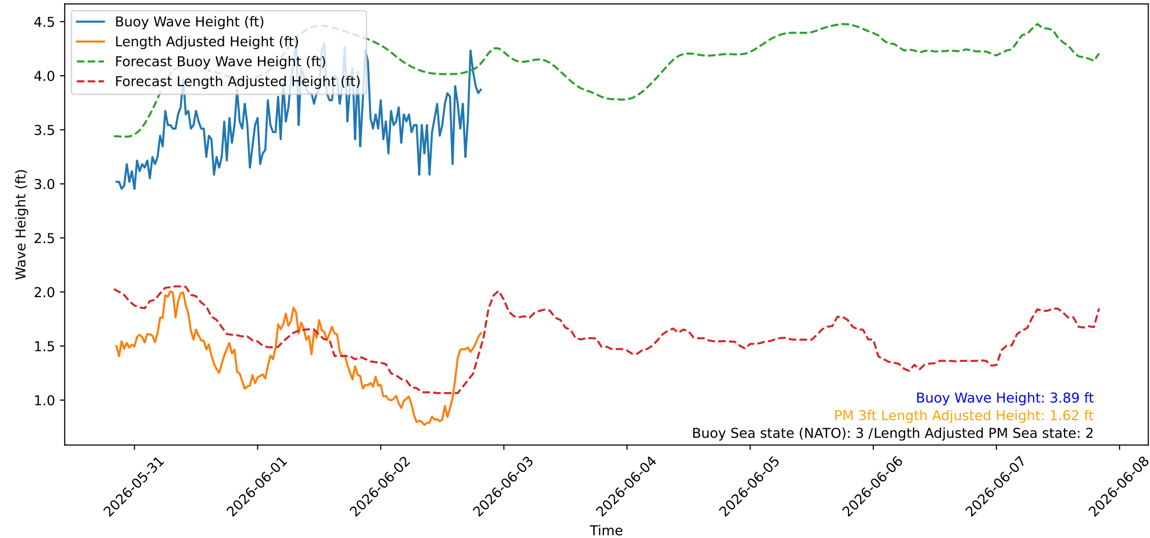
Wave Heights over Time for Green Beach at 2026-06-02 20:21:10
