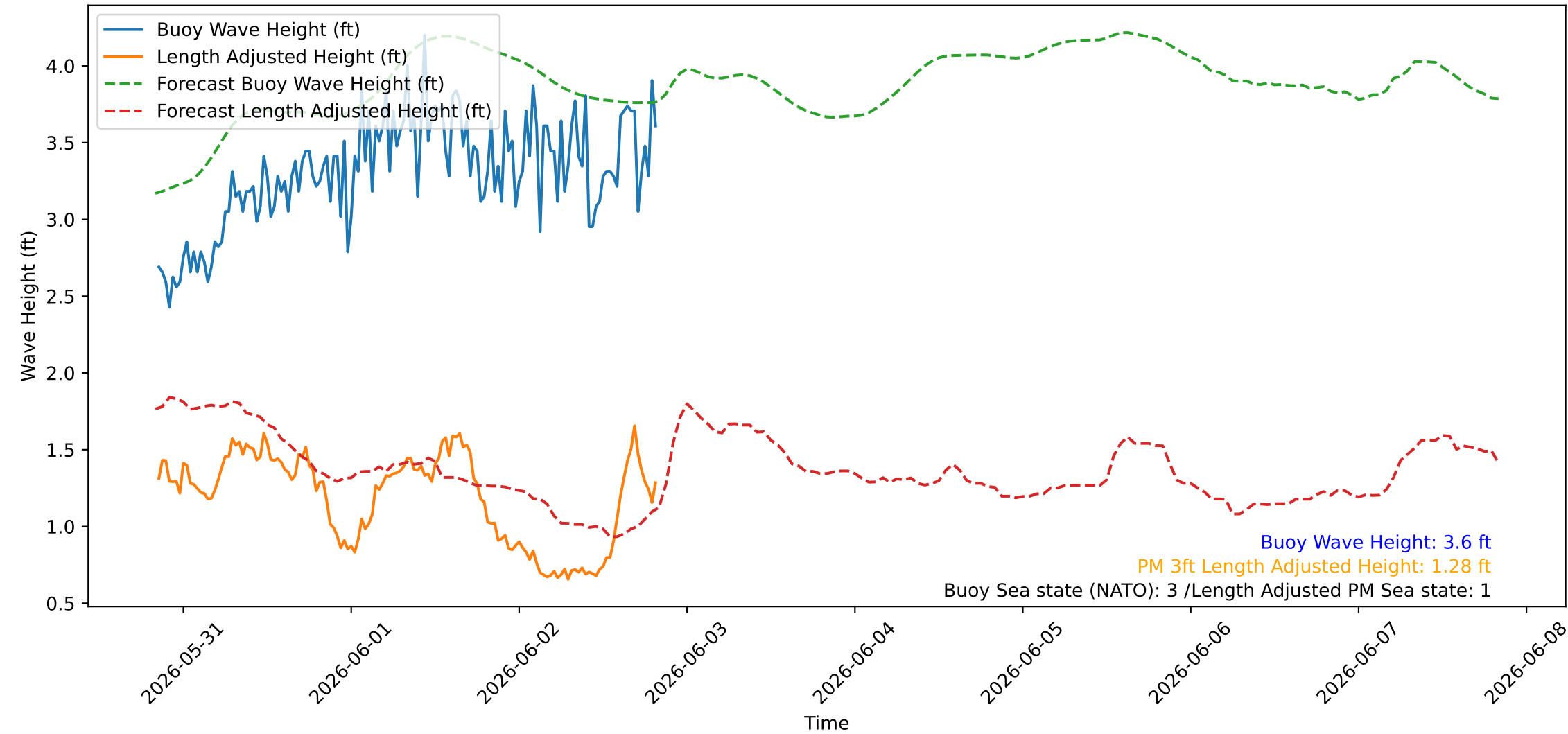
Wave Heights over Time for Red Beach at 2026-06-02 20:20:47
