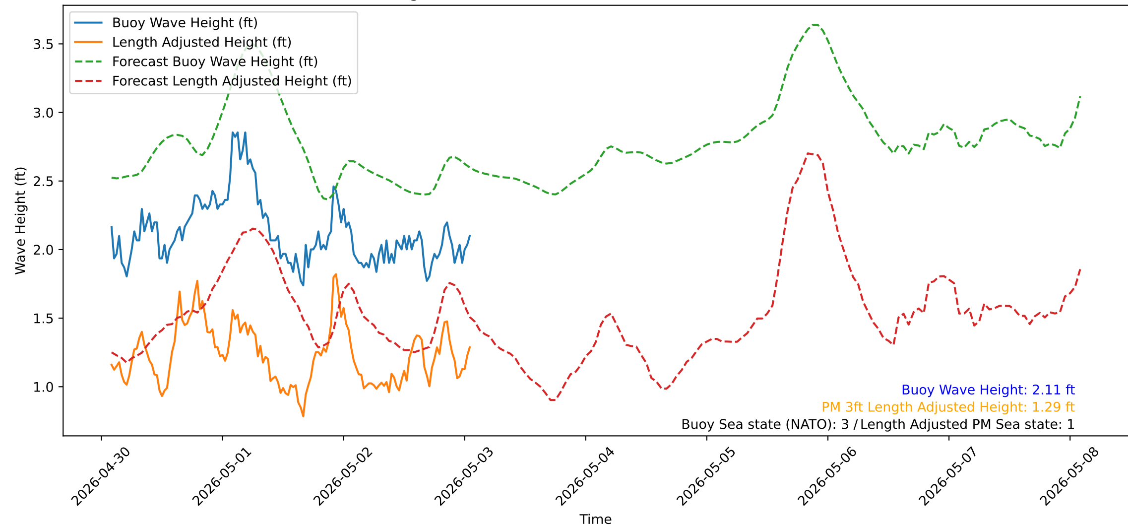
Wave Heights over Time for Green Beach at 2026-05-03 01:51:13
