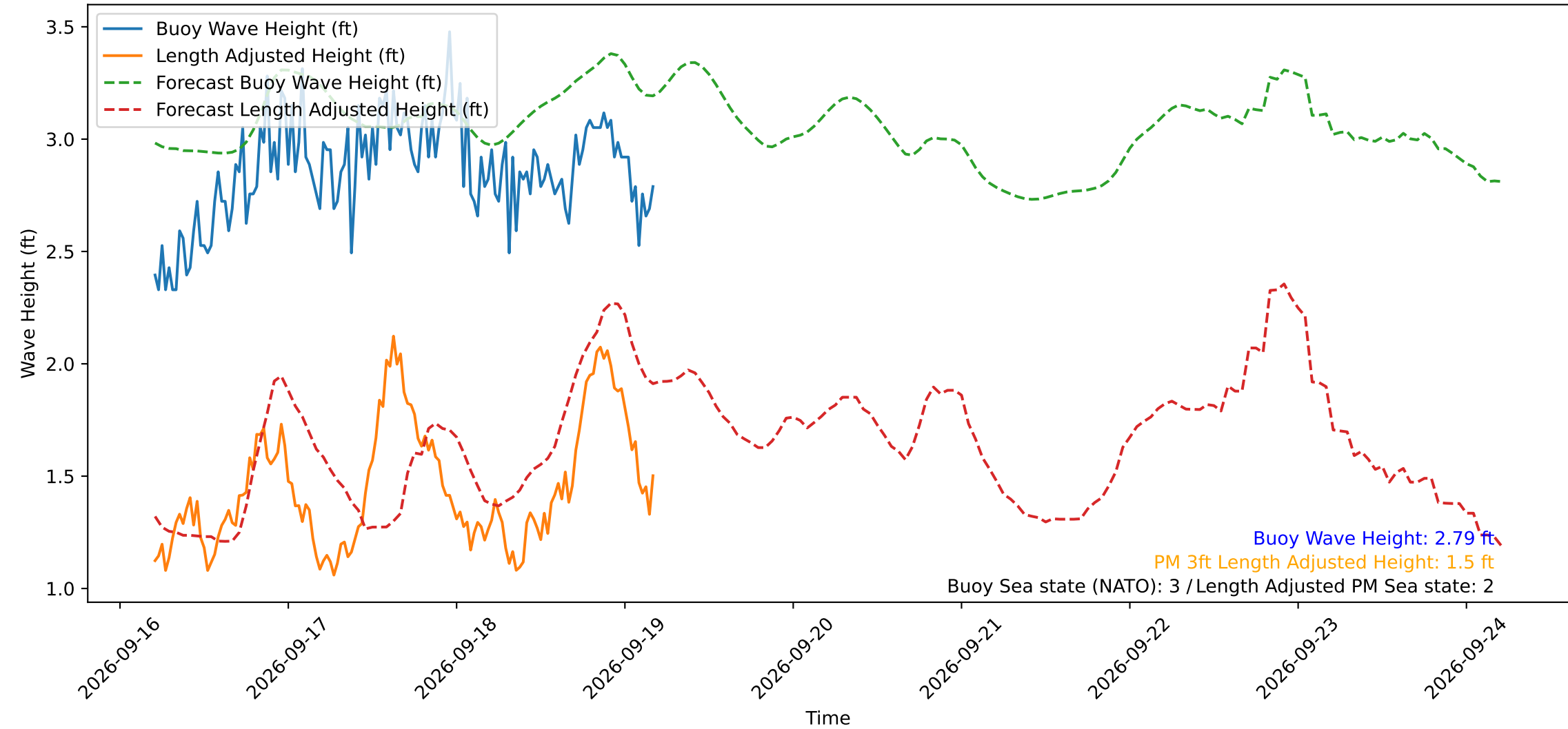
Wave Heights over Time for Green Beach at 2026-09-19 04:51:14
