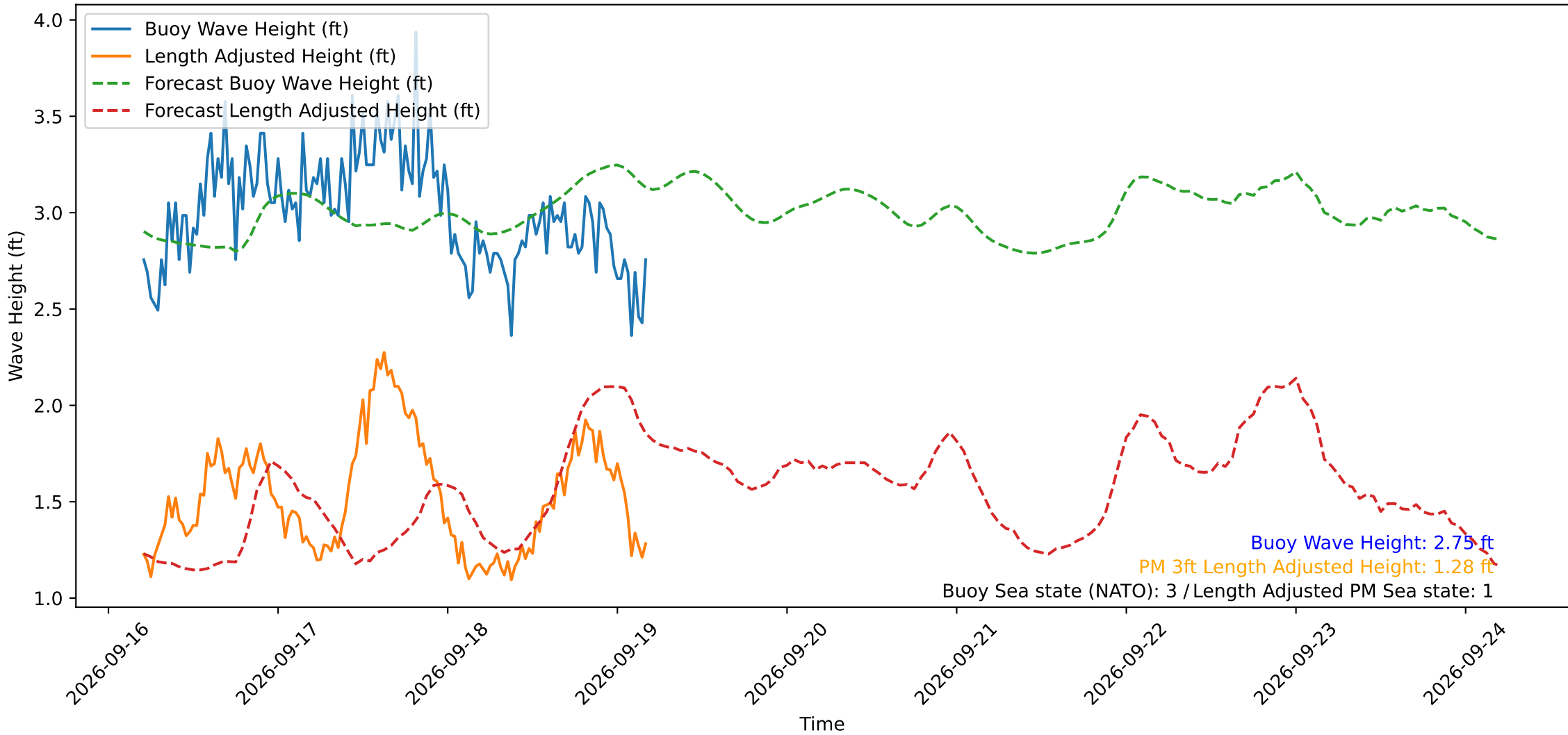
Wave Heights over Time for Oceanside Harbor at 2026-09-19 04:50:30
