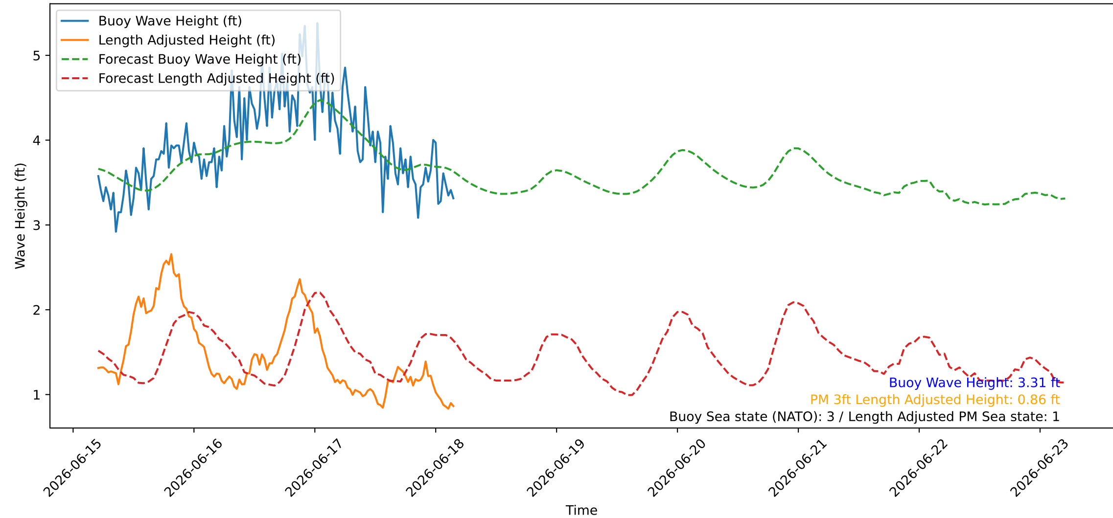
Wave Heights over Time for Red Beach at 2026-06-18 04:30:46
