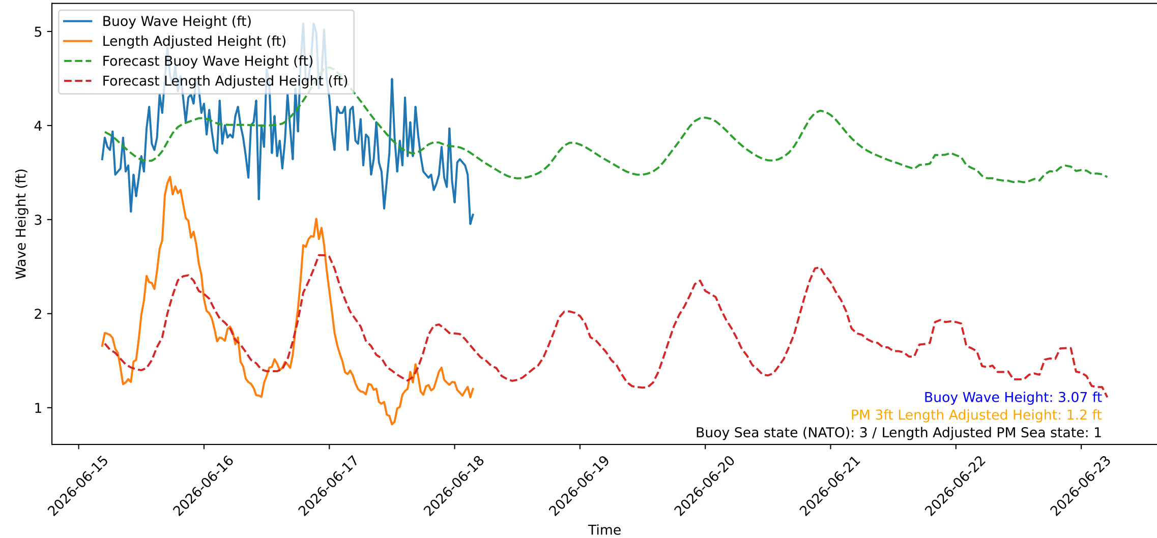
Wave Heights over Time for Green Beach at 2026-06-18 04:31:09
