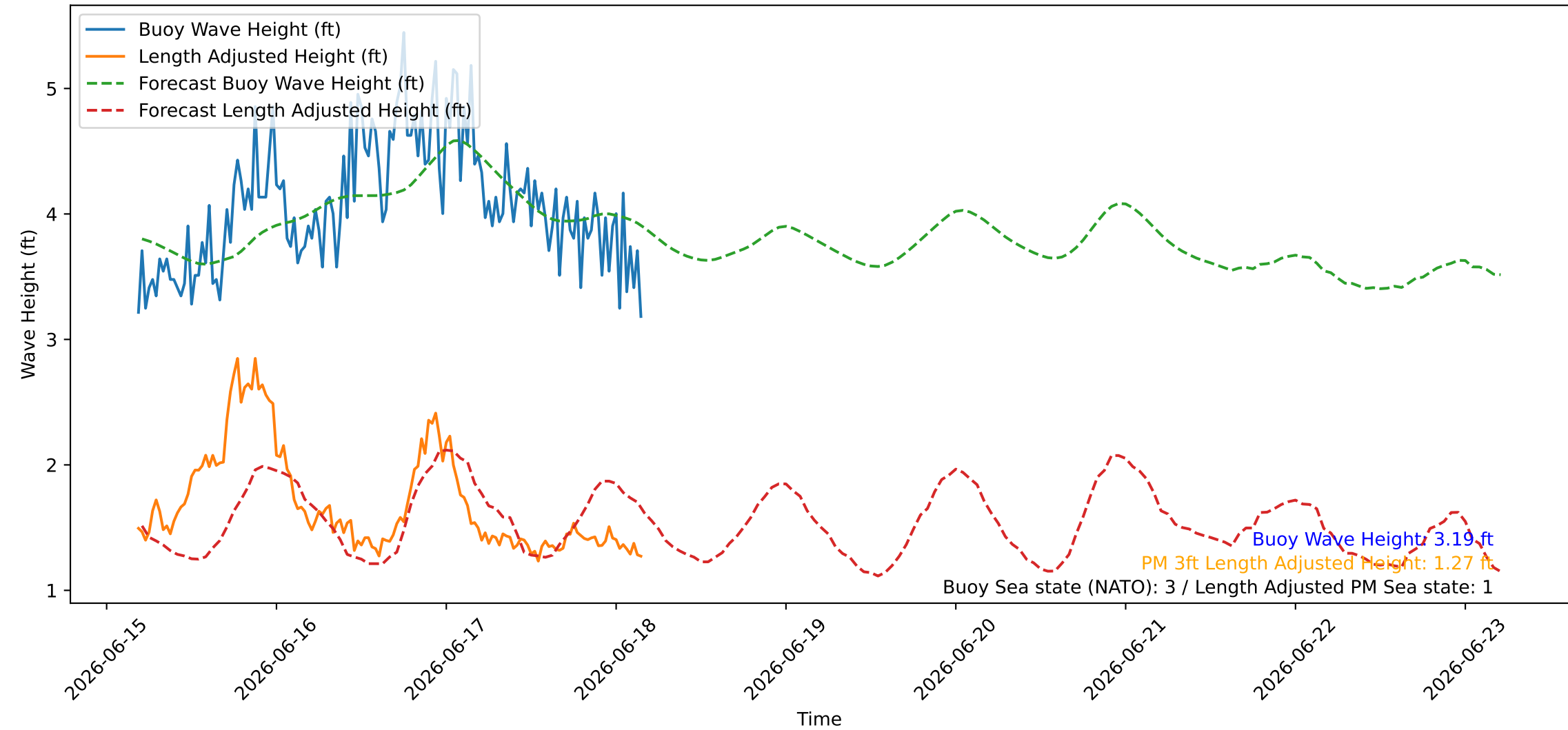
Wave Heights over Time for Oceanside Harbor at 2026-06-18 04:30:27
