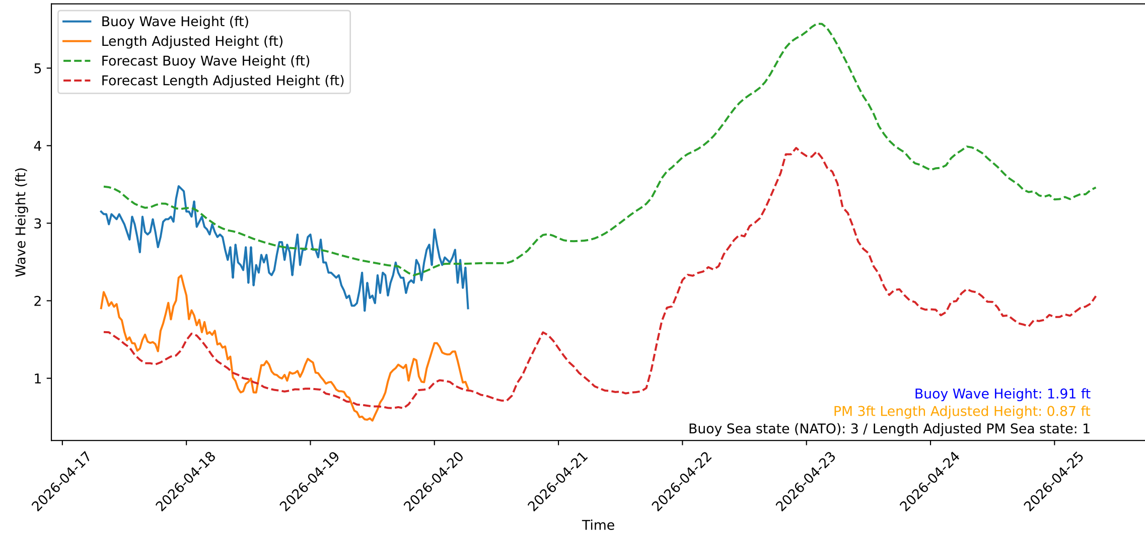
Wave Heights over Time for Green Beach at 2026-04-20 07:31:12
