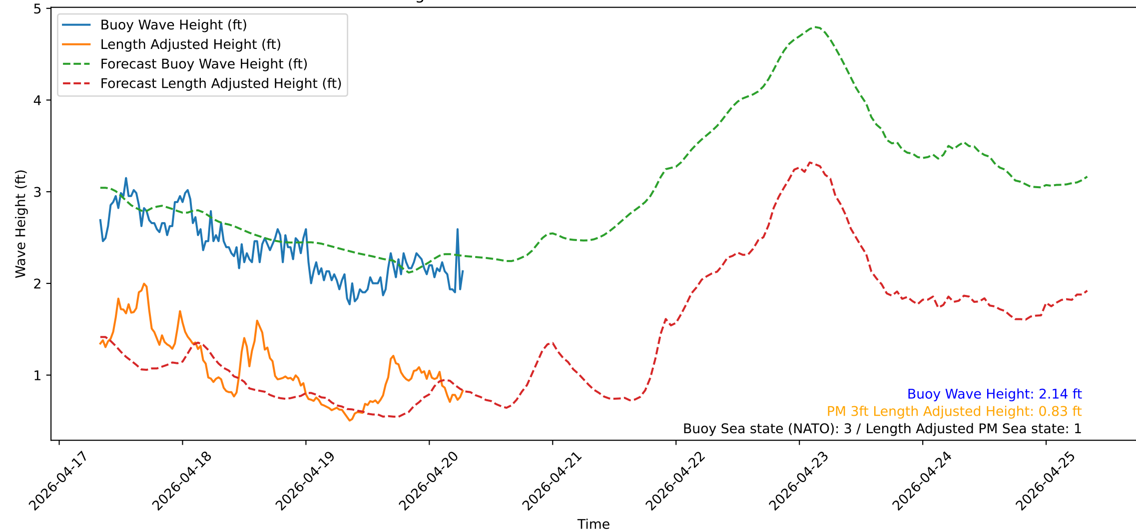
Wave Heights over Time for Red Beach at 2026-04-20 07:30:50
