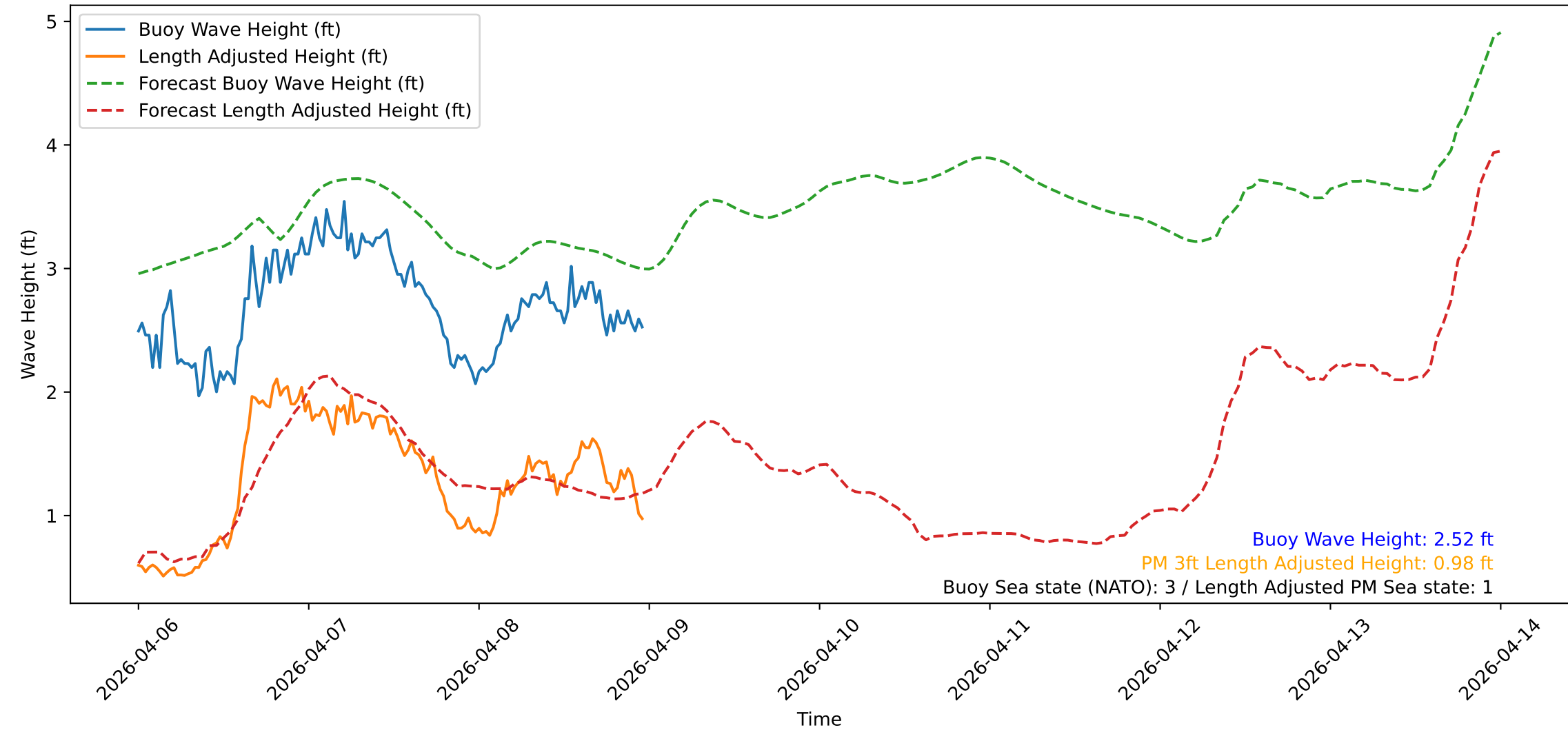
Wave Heights over Time for Red Beach at 2026-04-08 23:40:48
