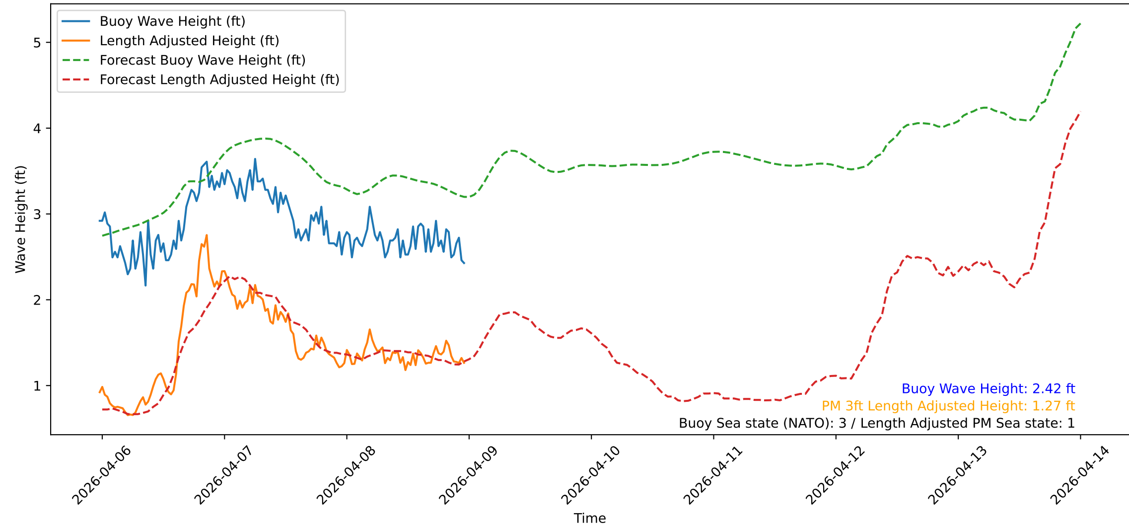
Wave Heights over Time for Oceanside Harbor at 2026-04-08 23:40:31
