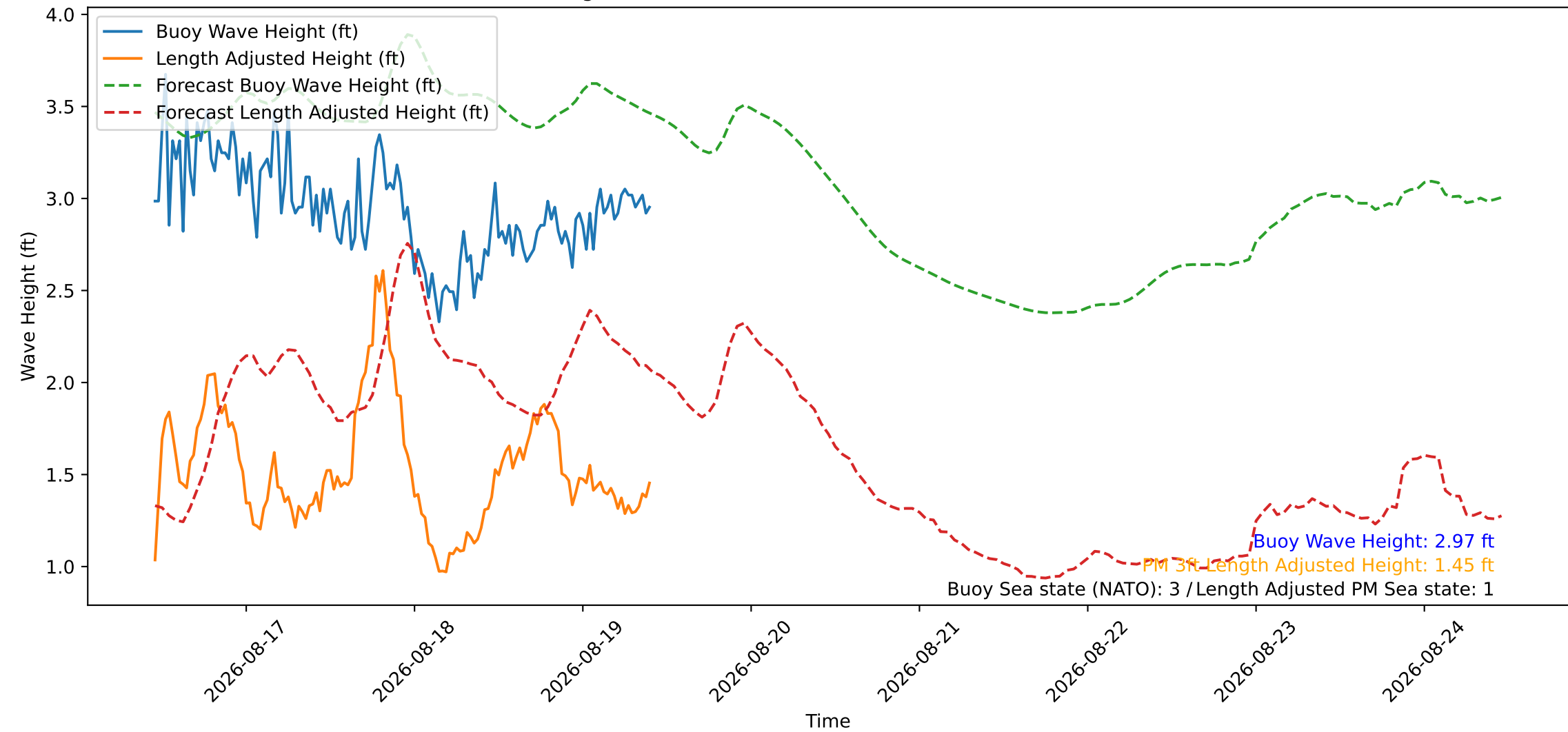
Wave Heights over Time for Red Beach at 2026-08-19 10:40:46
