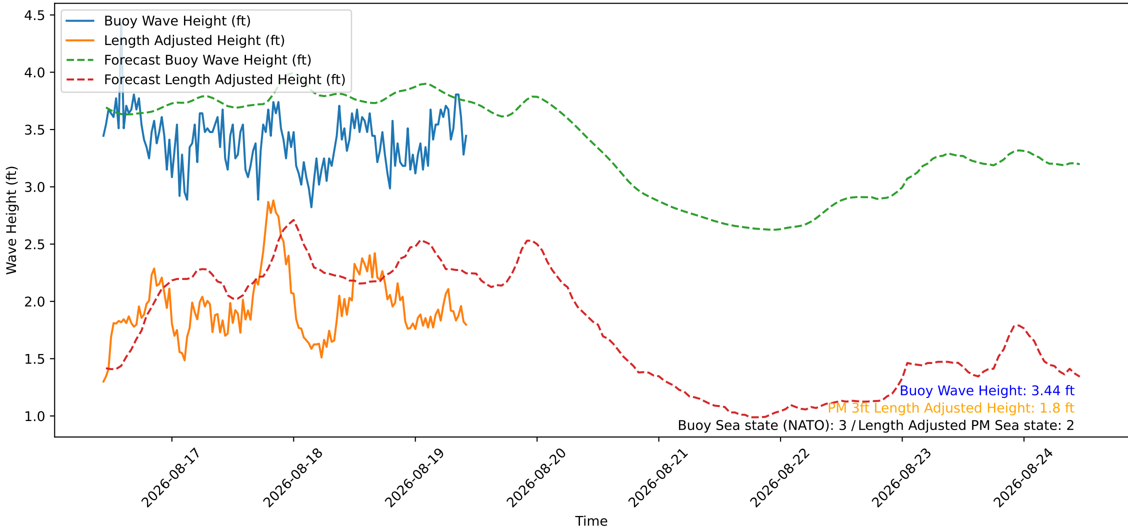
Wave Heights over Time for Oceanside Harbor at 2026-08-19 10:40:27
