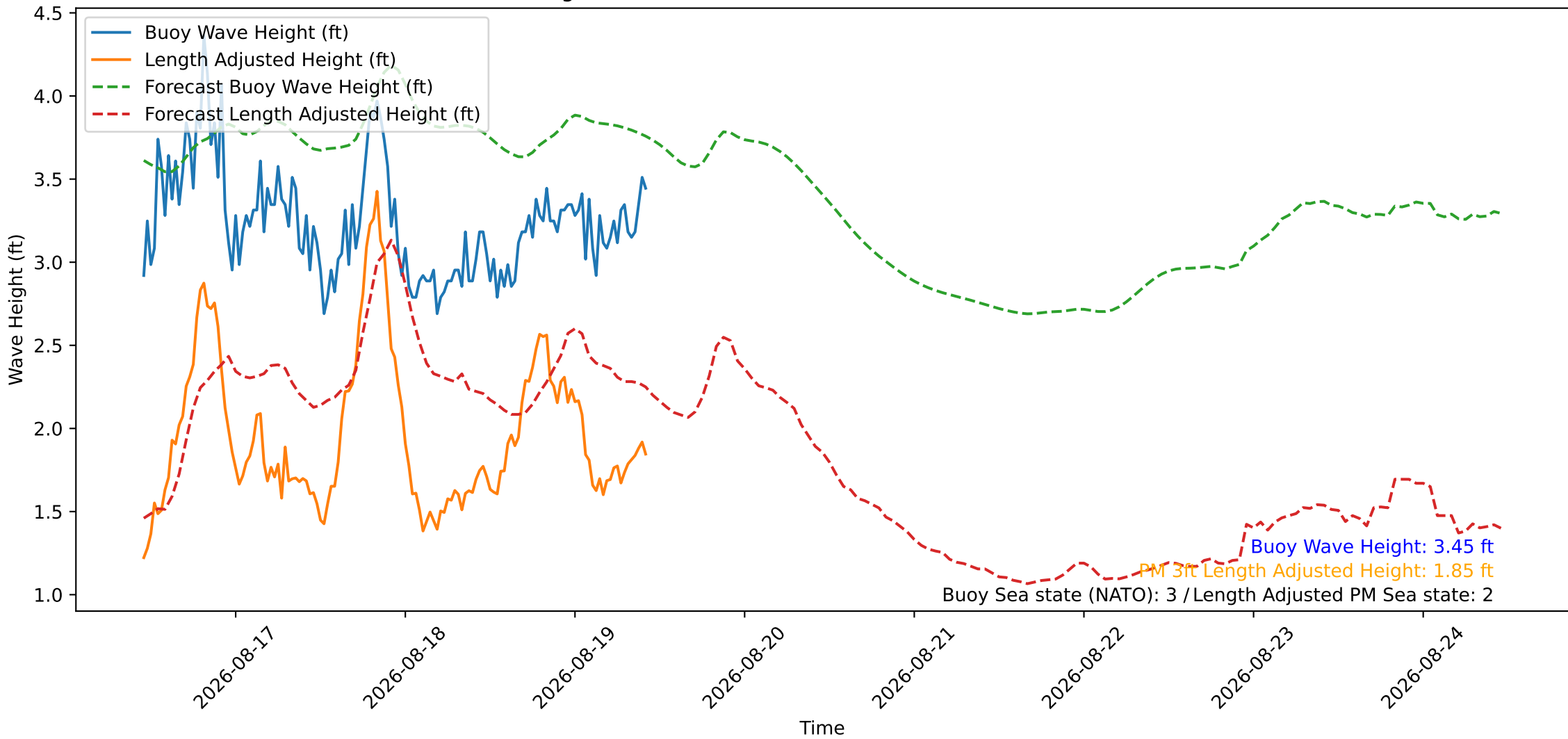
Wave Heights over Time for Green Beach at 2026-08-19 10:41:09
