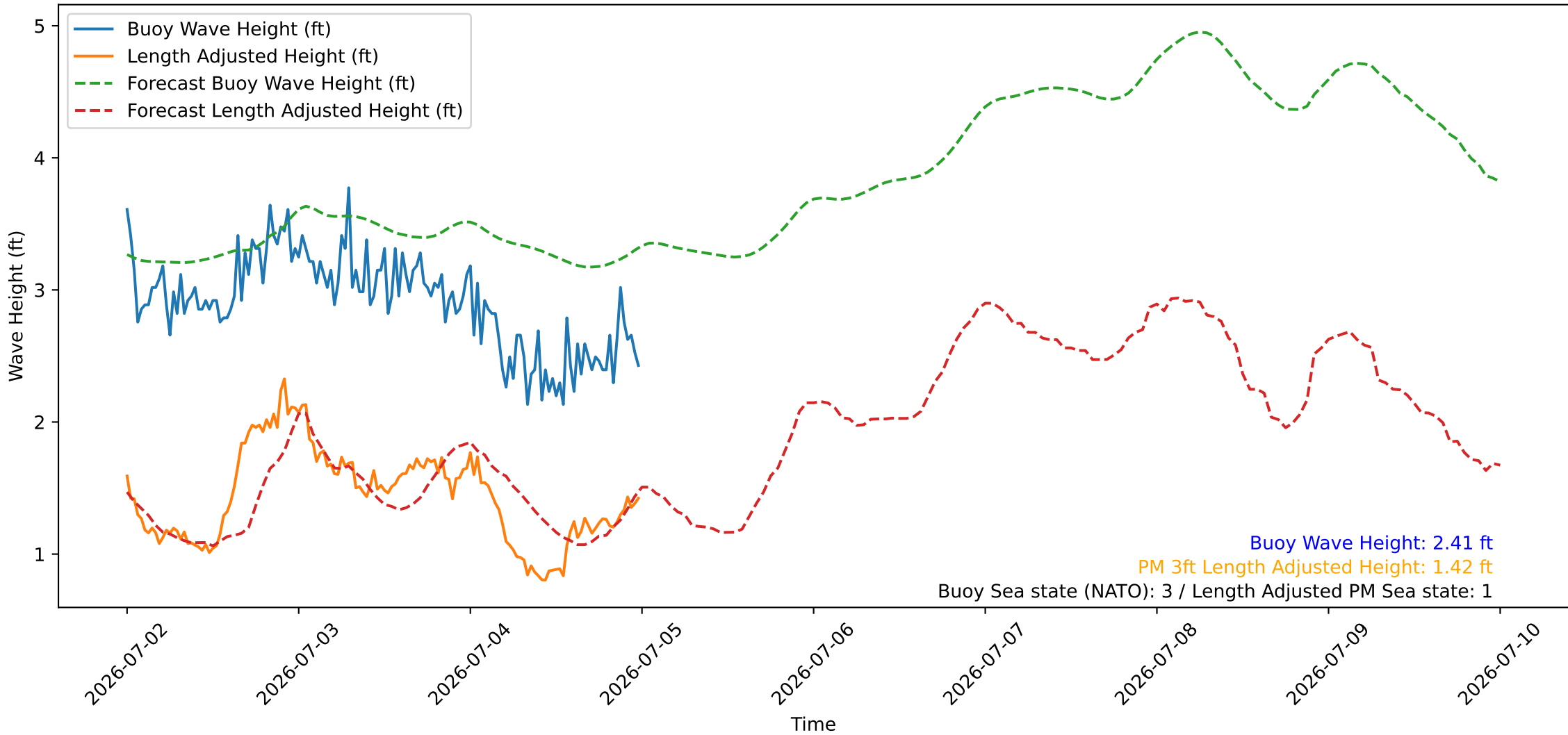
Wave Heights over Time for Oceanside Harbor at 2026-07-05 00:10:26
