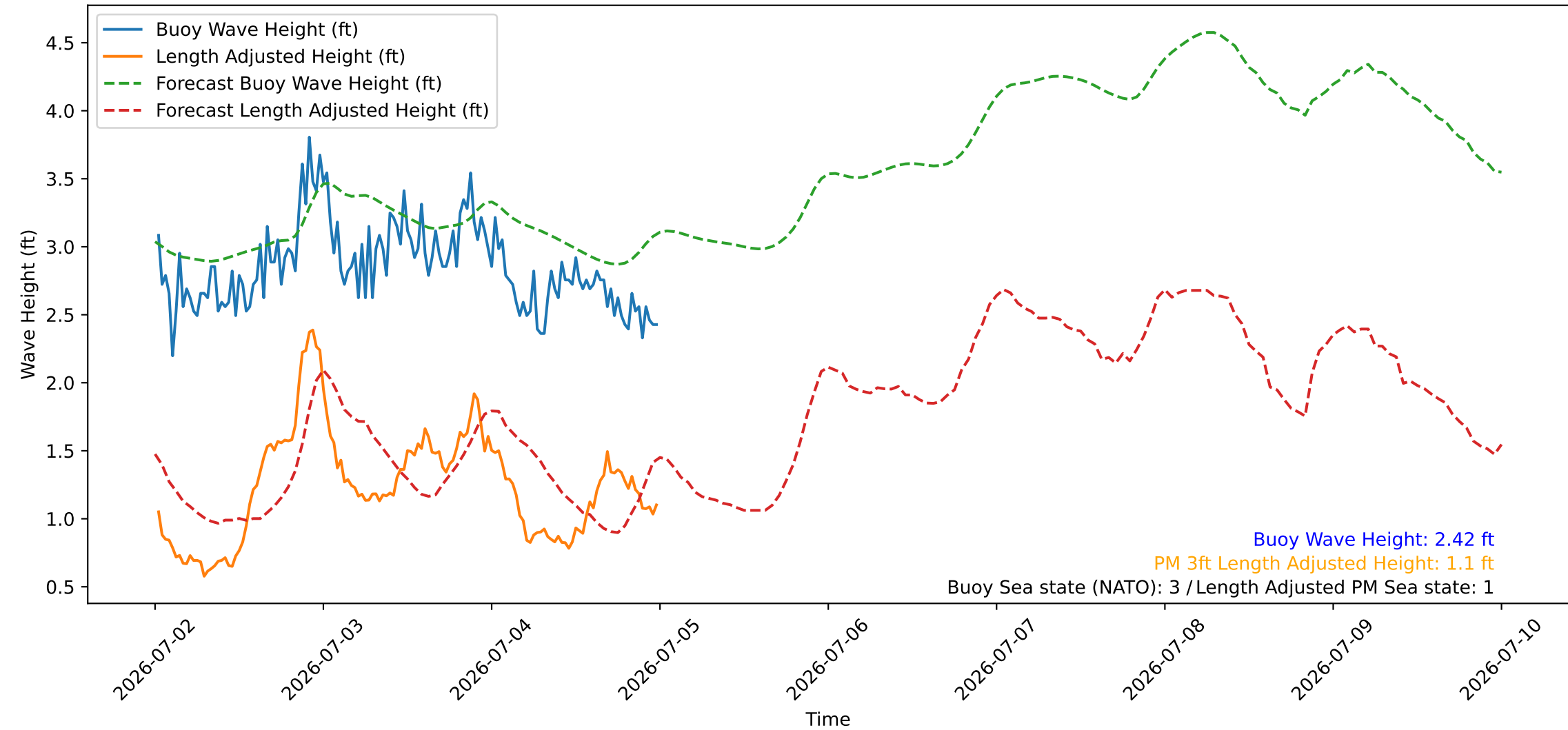
Wave Heights over Time for Red Beach at 2026-07-05 00:10:46
