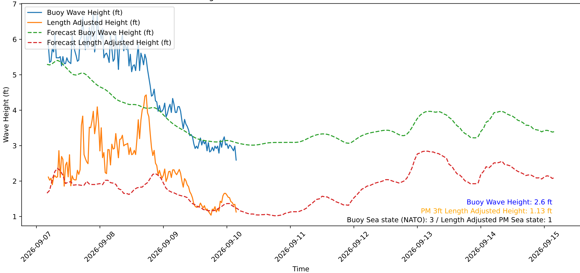
Wave Heights over Time for Red Beach at 2026-09-10 04:10:49
