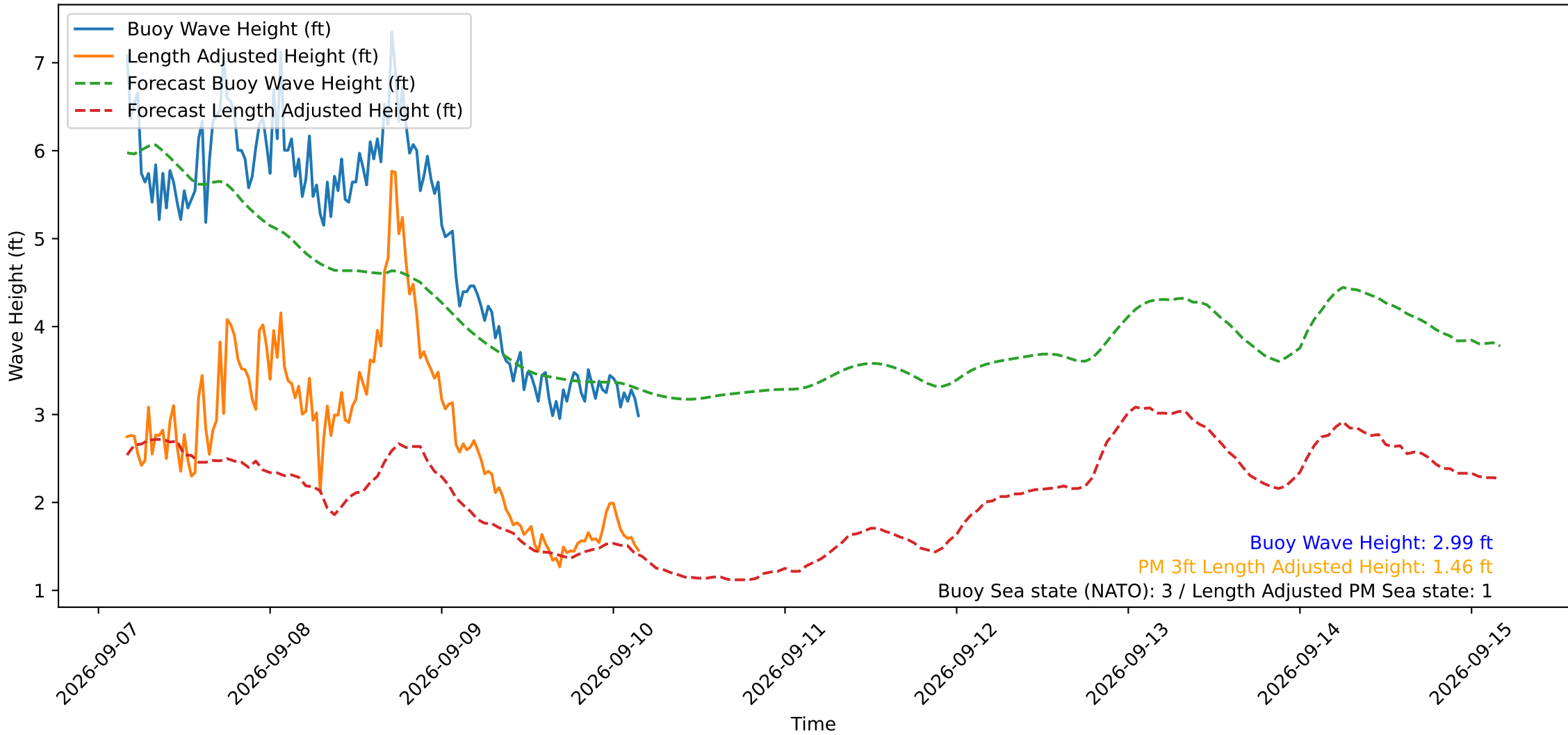
Wave Heights over Time for Oceanside Harbor at 2026-09-10 04:10:29
