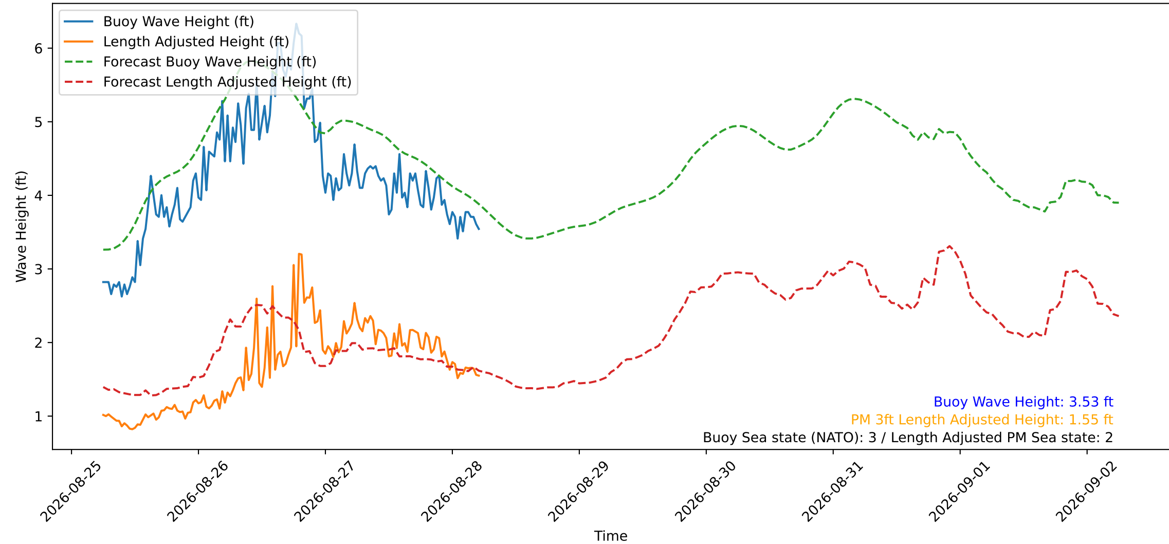
Wave Heights over Time for Green Beach at 2026-08-28 05:41:11
