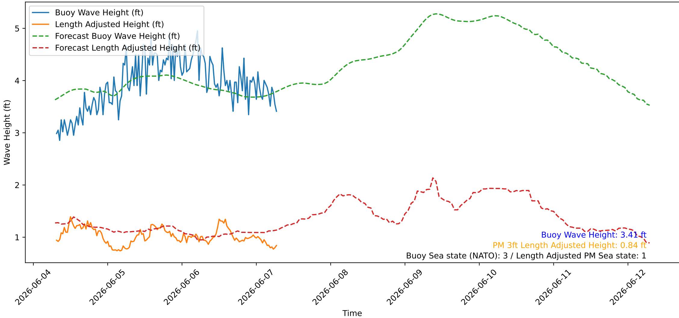
Wave Heights over Time for Red Beach at 2026-06-07 07:20:47
