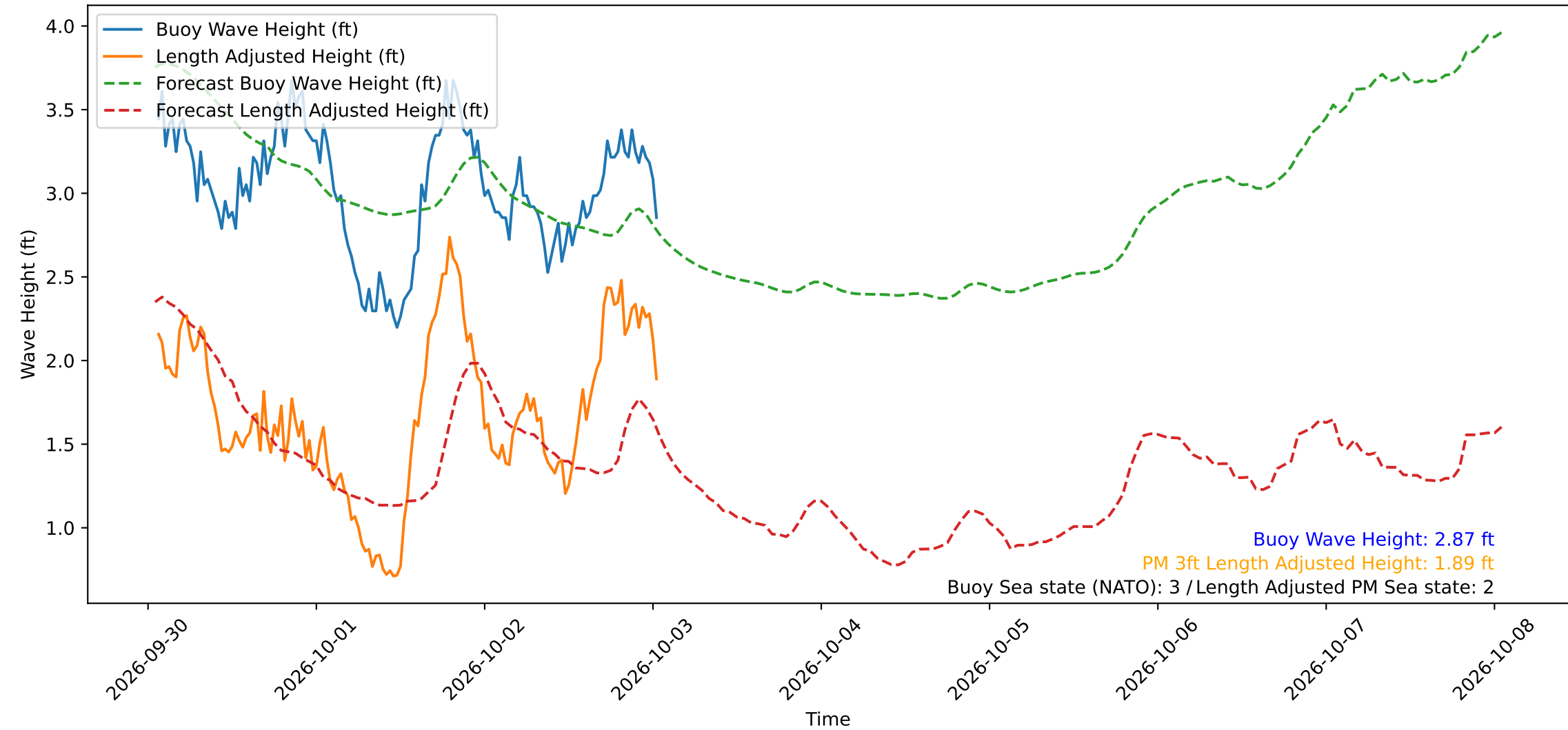
Wave Heights over Time for Green Beach at 2026-10-03 01:21:14
