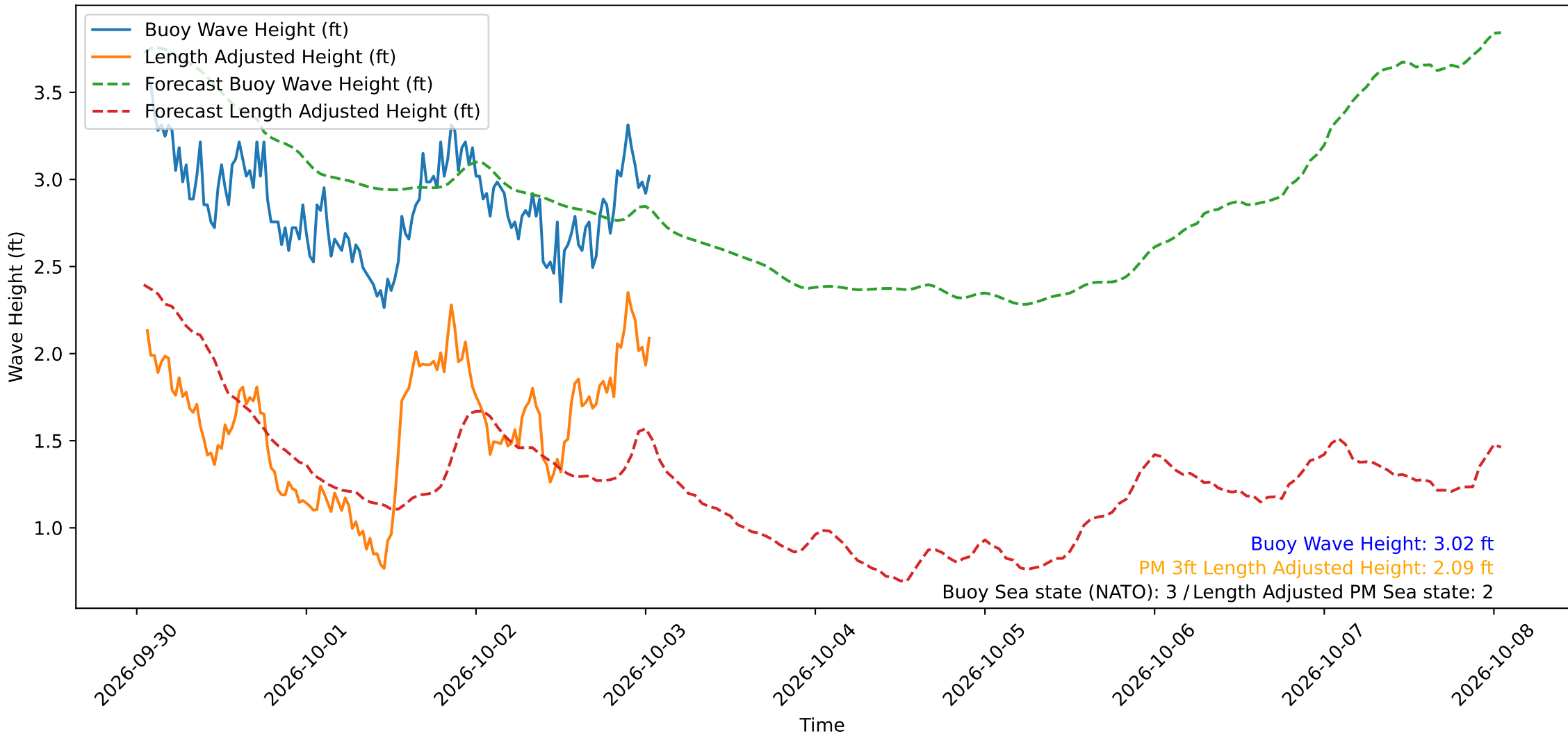
Wave Heights over Time for Oceanside Harbor at 2026-10-03 01:20:29
