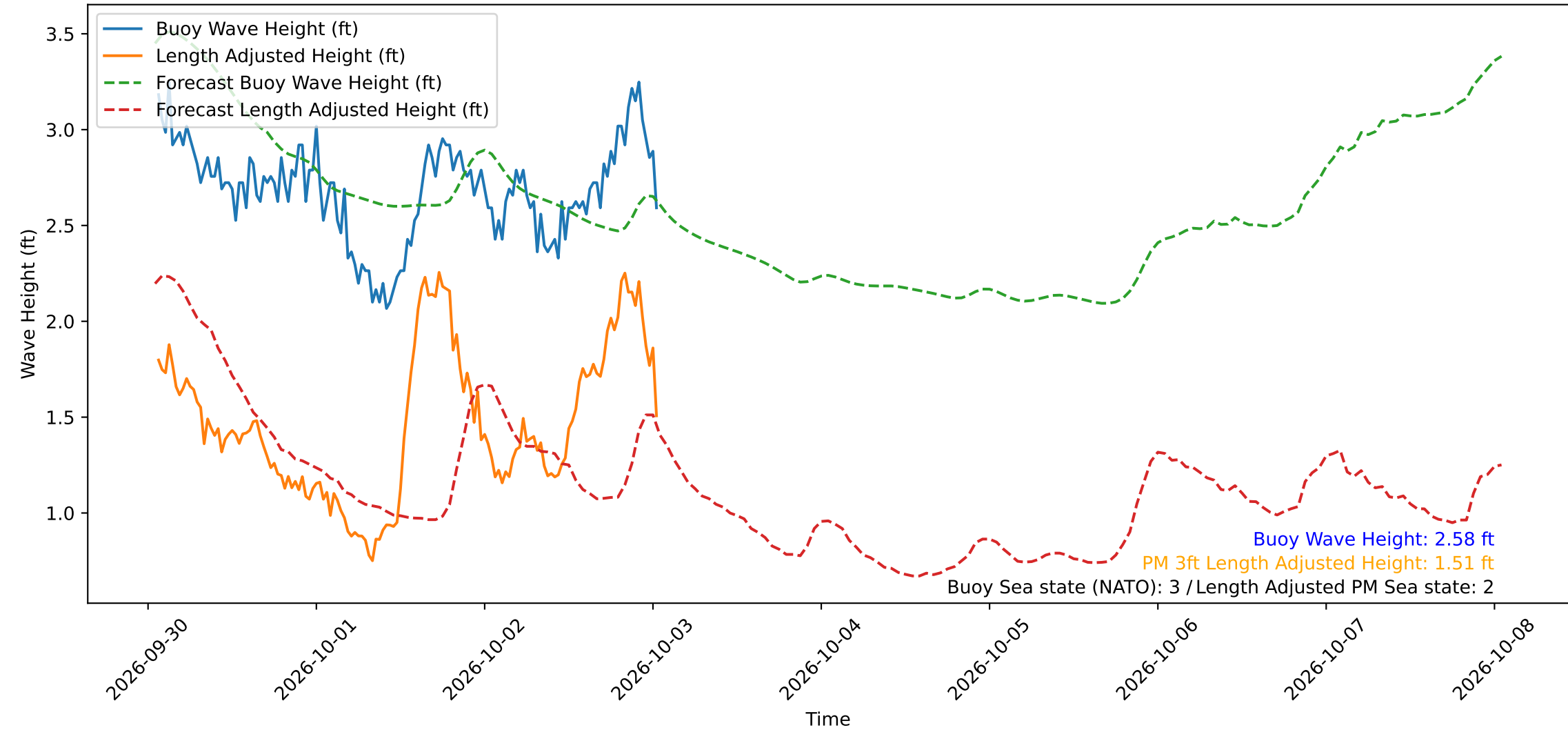
Wave Heights over Time for Red Beach at 2026-10-03 01:20:50
