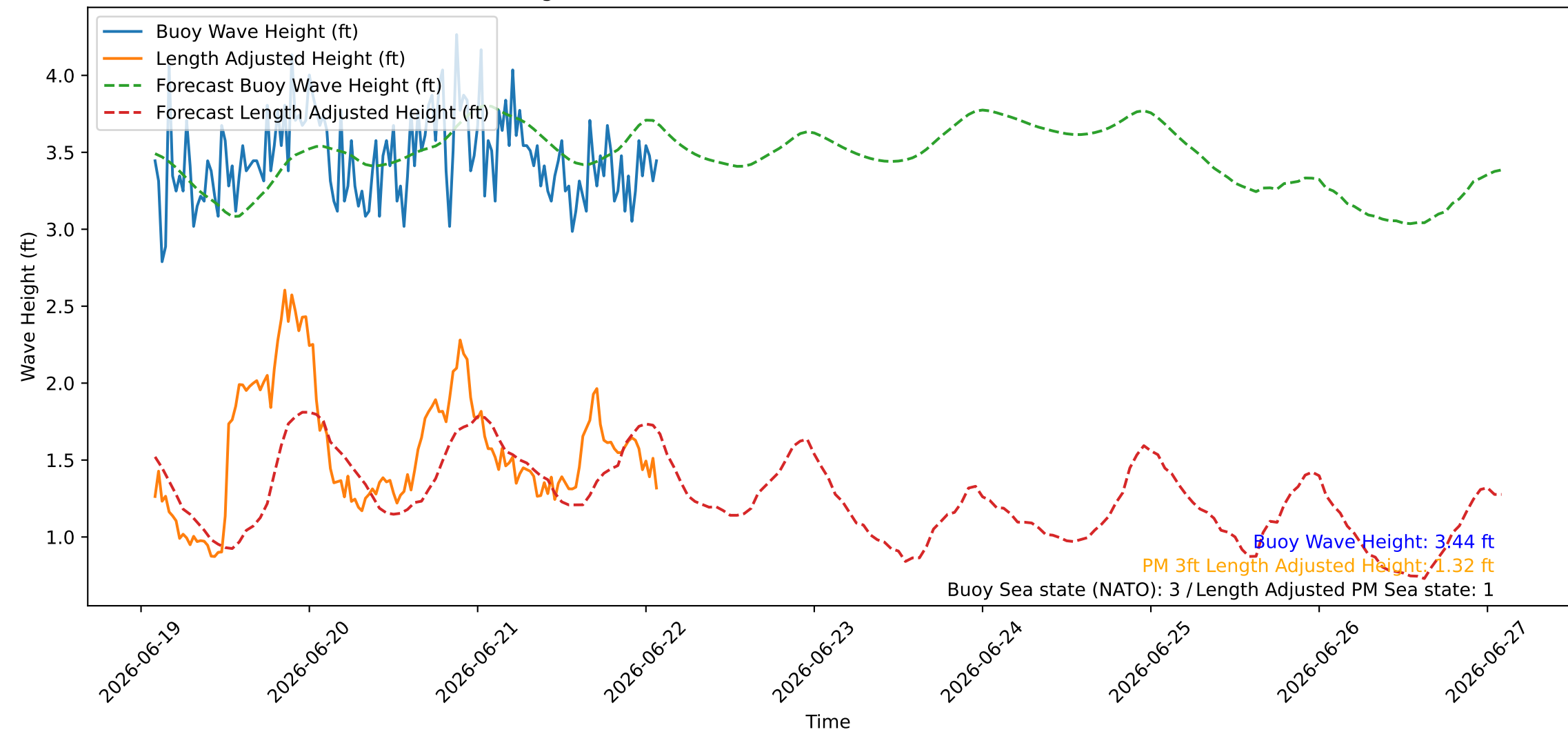
Wave Heights over Time for Oceanside Harbor at 2026-06-22 02:10:26
