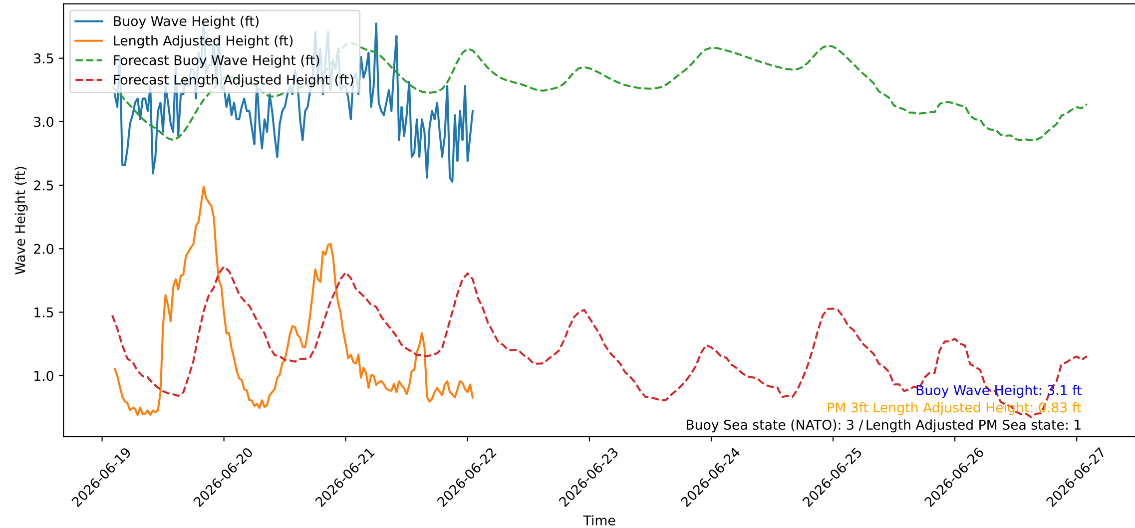
Wave Heights over Time for Red Beach at 2026-06-22 02:10:45
