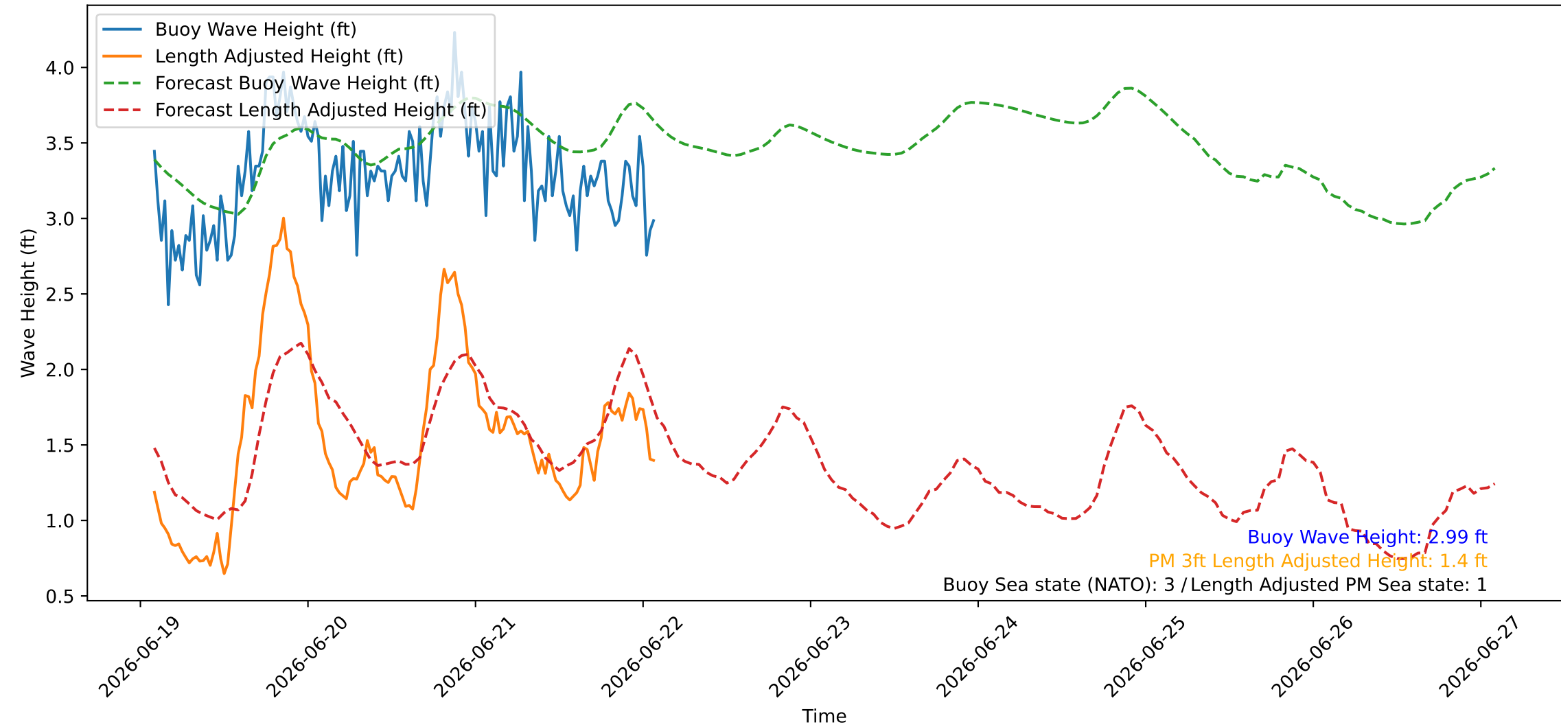
Wave Heights over Time for Green Beach at 2026-06-22 02:11:08
