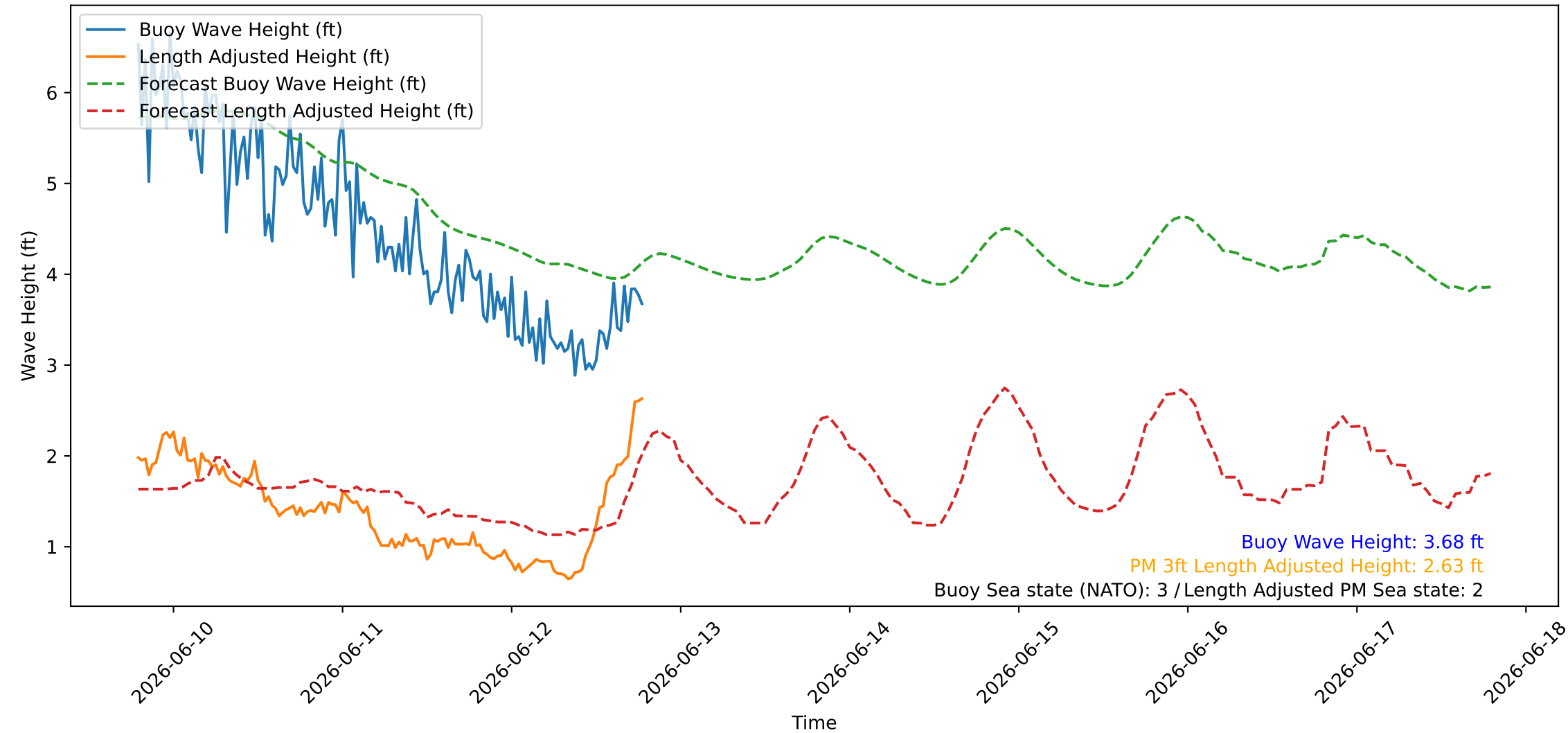
Wave Heights over Time for Green Beach at 2026-06-12 19:11:09
