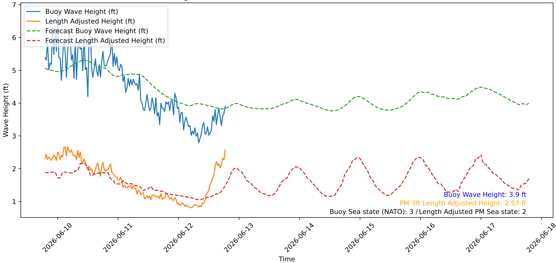
Wave Heights over Time for Oceanside Harbor at 2026-06-12 19:10:26
