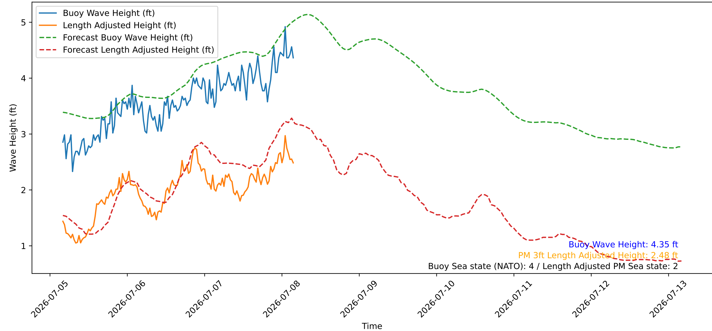
Wave Heights over Time for Oceanside Harbor at 2026-07-08 04:10:26
