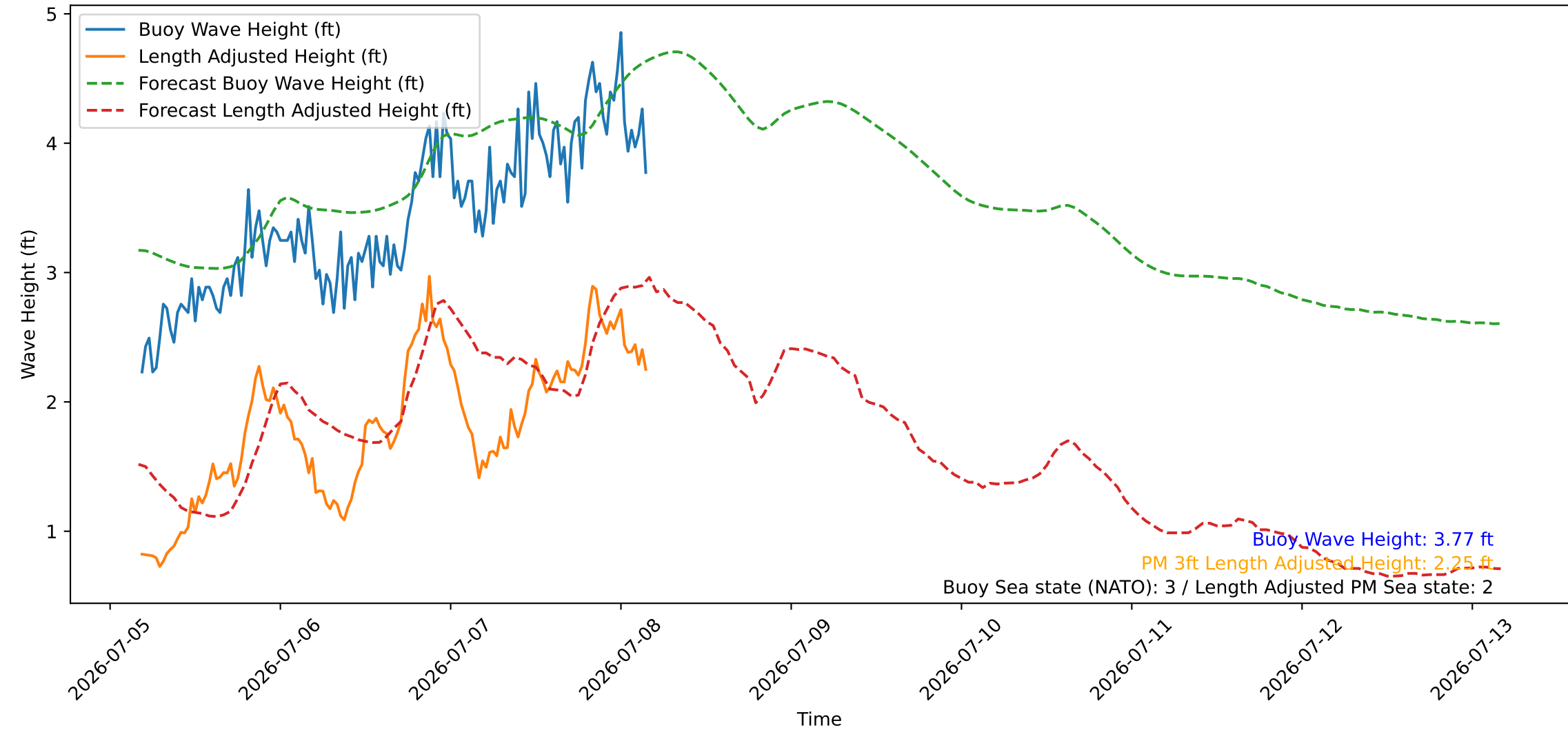
Wave Heights over Time for Red Beach at 2026-07-08 04:10:46
