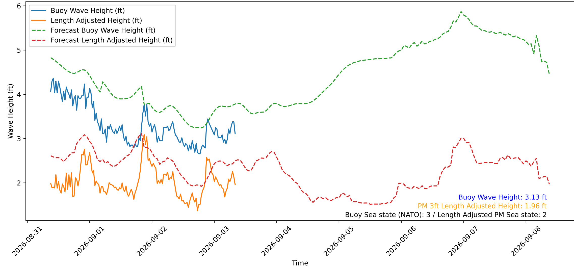
Wave Heights over Time for Green Beach at 2026-09-03 08:41:11
