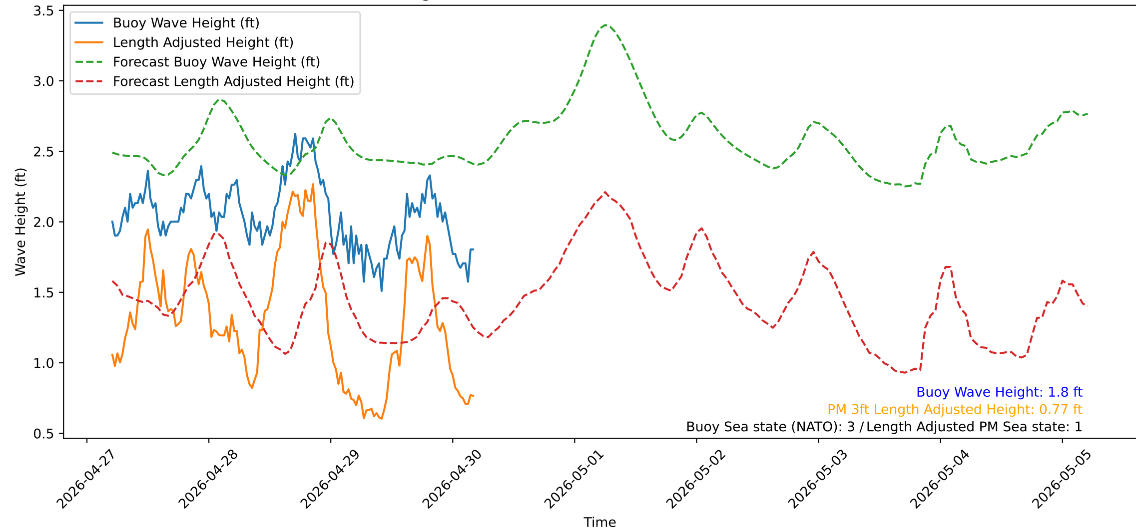
Wave Heights over Time for Red Beach at 2026-04-30 04:40:50
