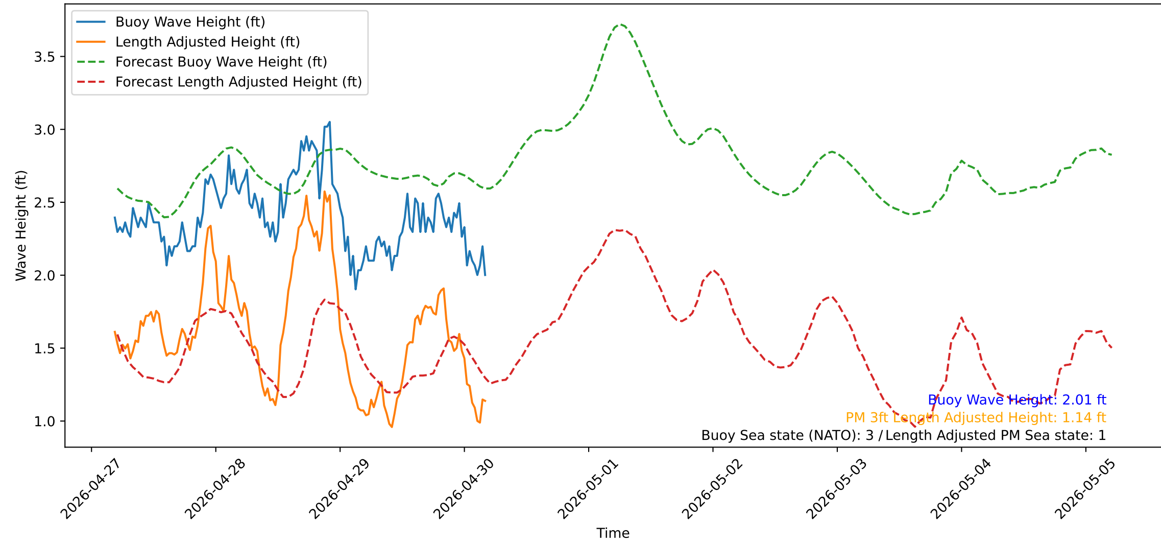
Wave Heights over Time for Oceanside Harbor at 2026-04-30 04:40:31
