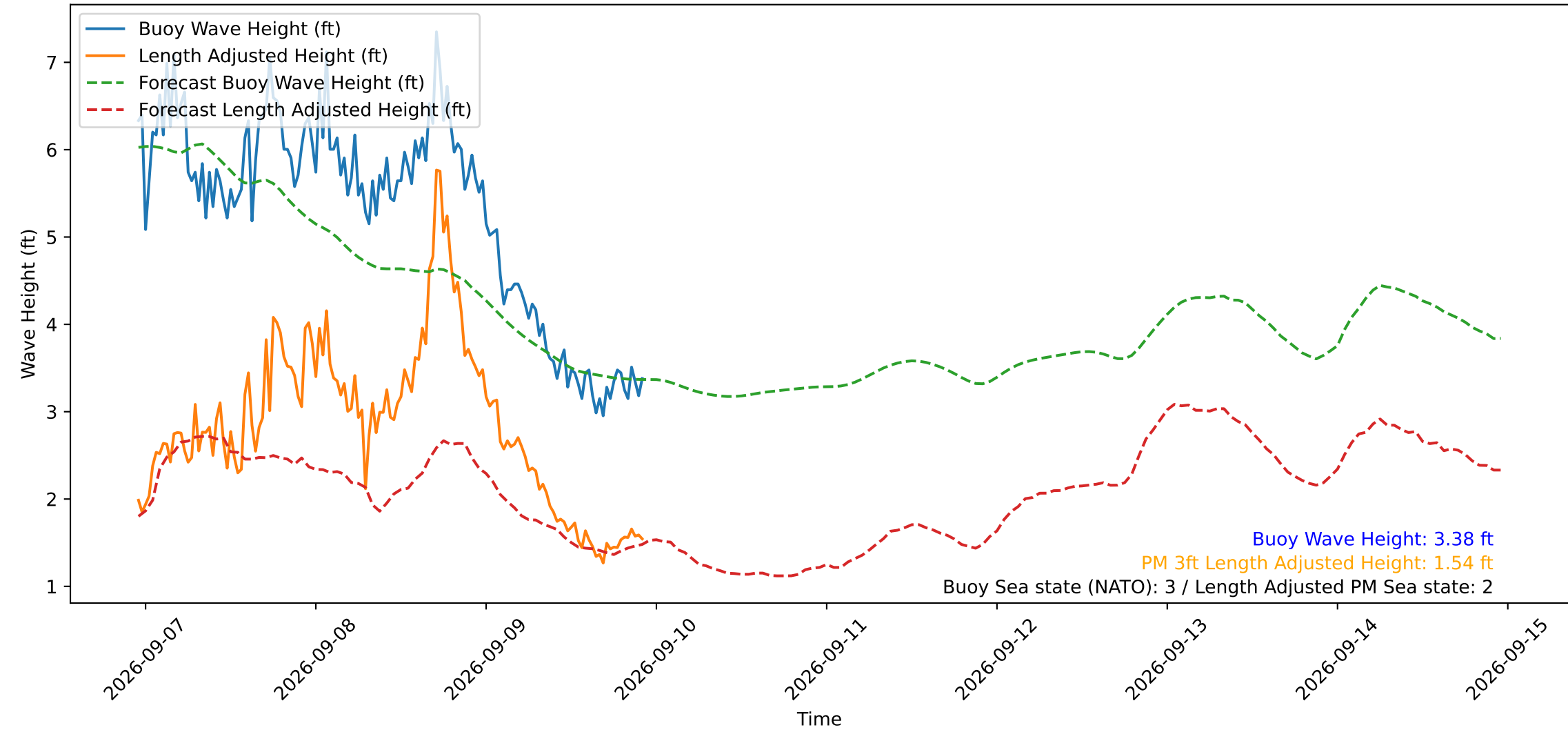
Wave Heights over Time for Oceanside Harbor at 2026-09-09 23:00:29
