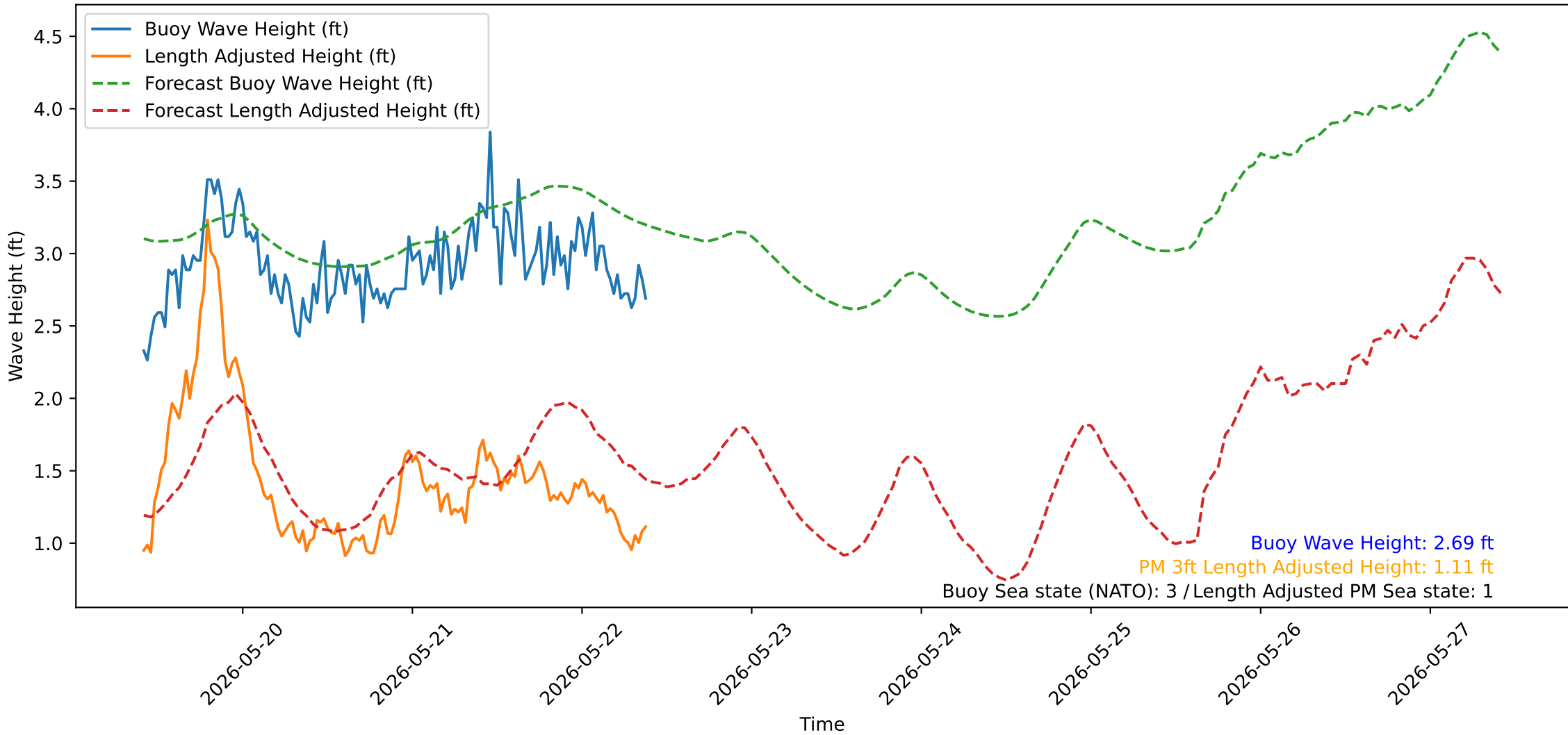
Wave Heights over Time for Oceanside Harbor at 2026-05-22 09:50:31
