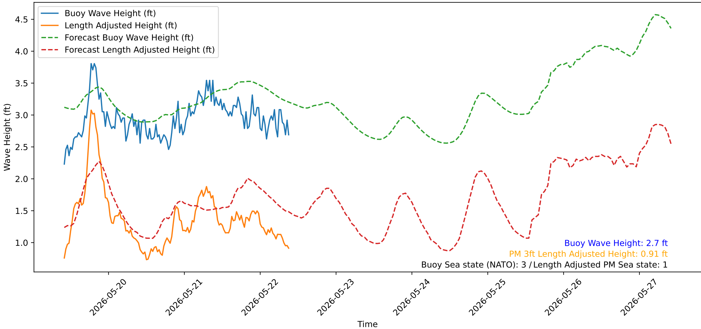
Wave Heights over Time for Green Beach at 2026-05-22 09:51:14
