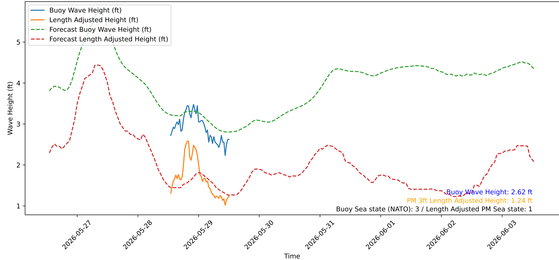
Wave Heights over Time for Oceanside Harbor at 2026-05-29 13:00:21
