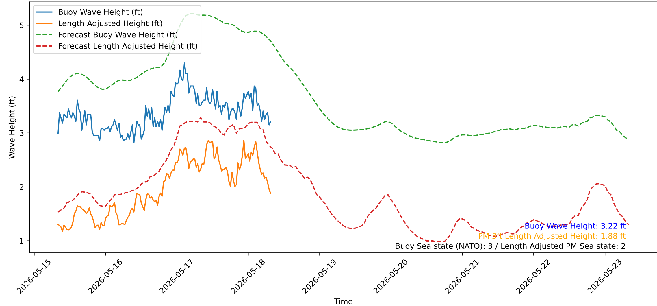
Wave Heights over Time for Oceanside Harbor at 2026-05-18 08:00:32
