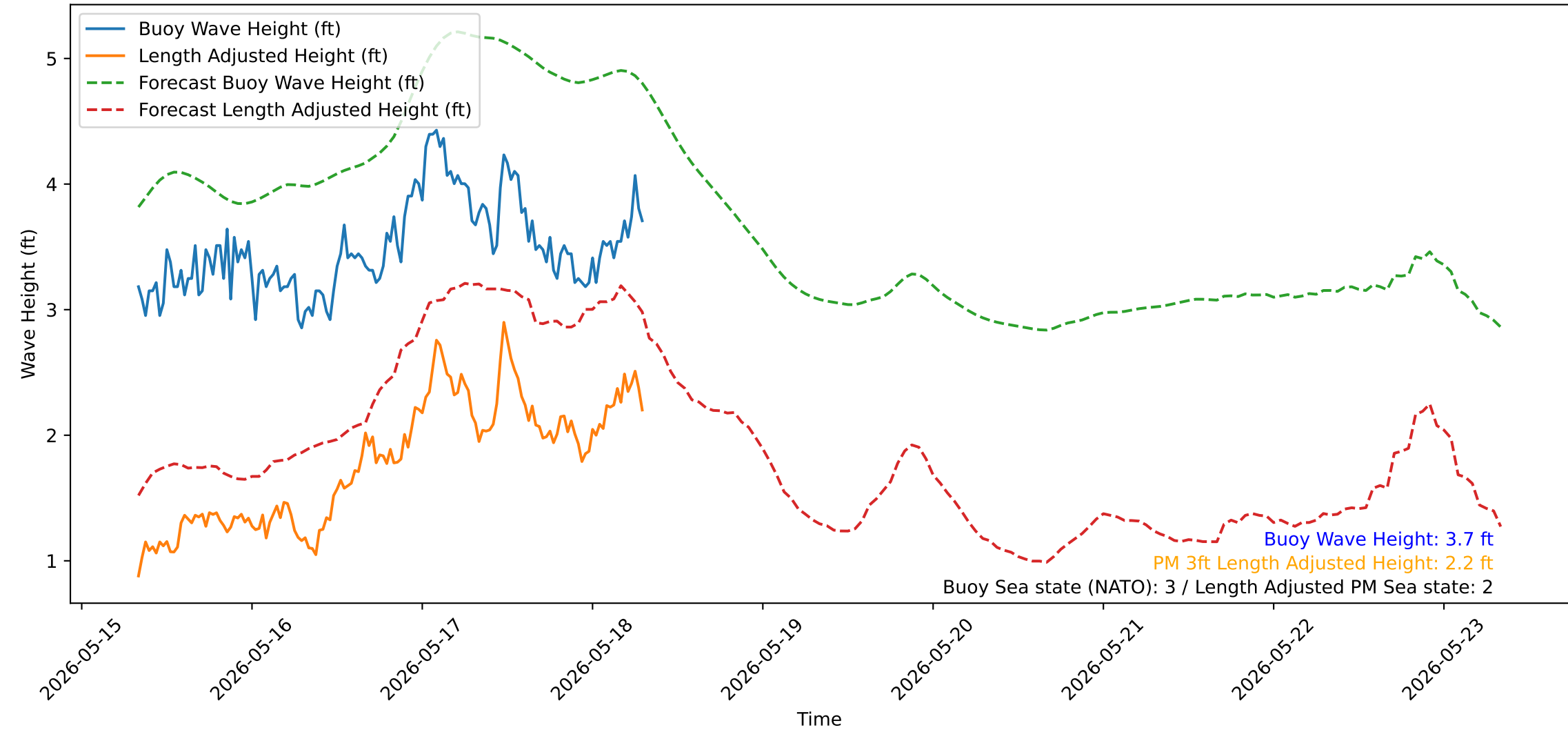
Wave Heights over Time for Green Beach at 2026-05-18 08:01:14
