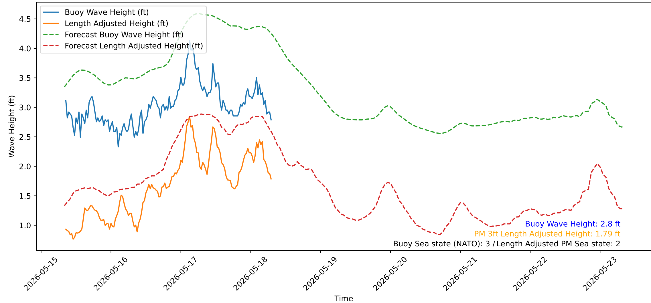
Wave Heights over Time for Red Beach at 2026-05-18 08:00:51
