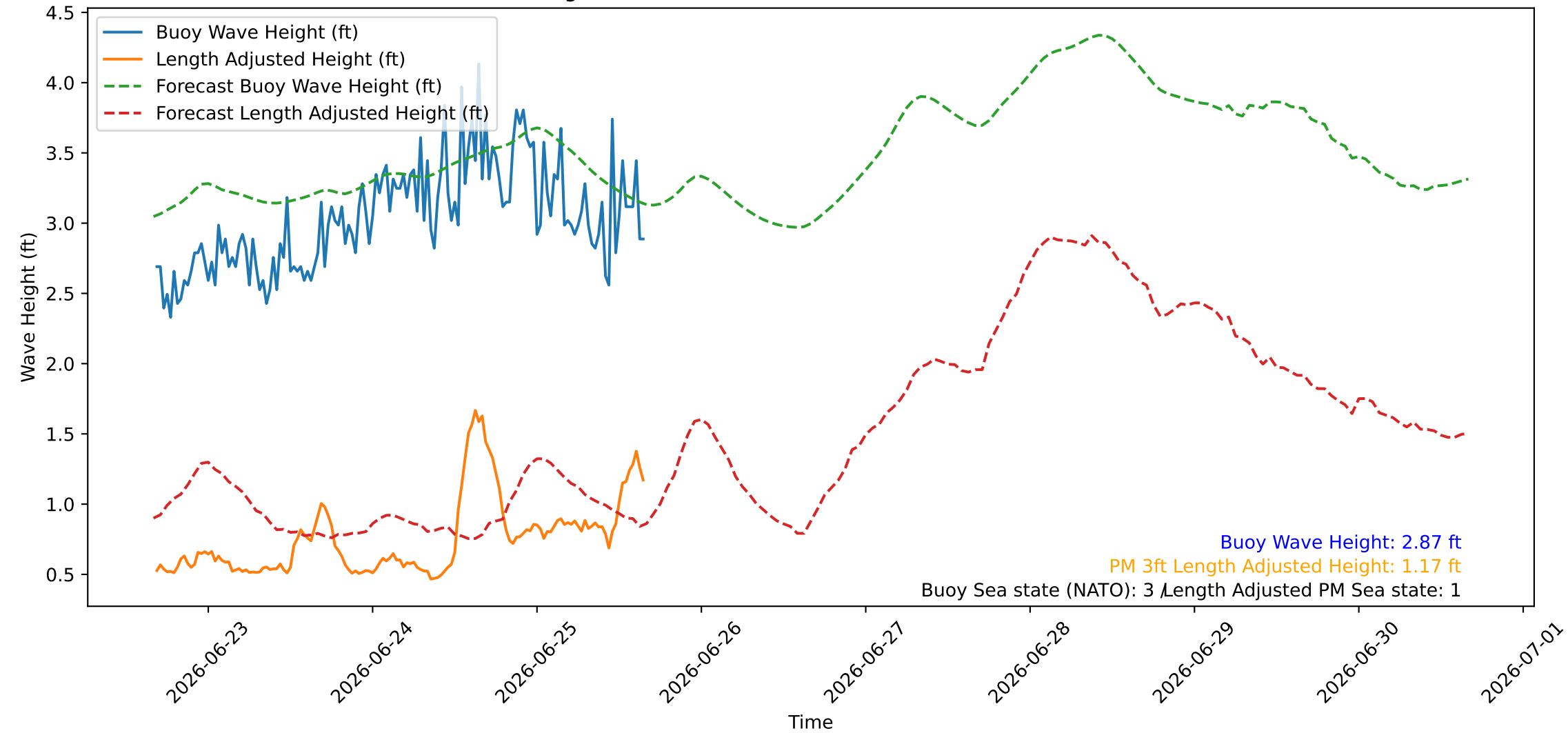
Wave Heights over Time for Red Beach at 2026-06-25 16:10:45
