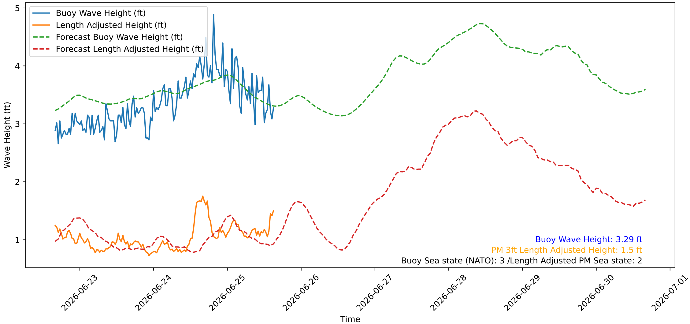
Wave Heights over Time for Oceanside Harbor at 2026-06-25 16:10:26
