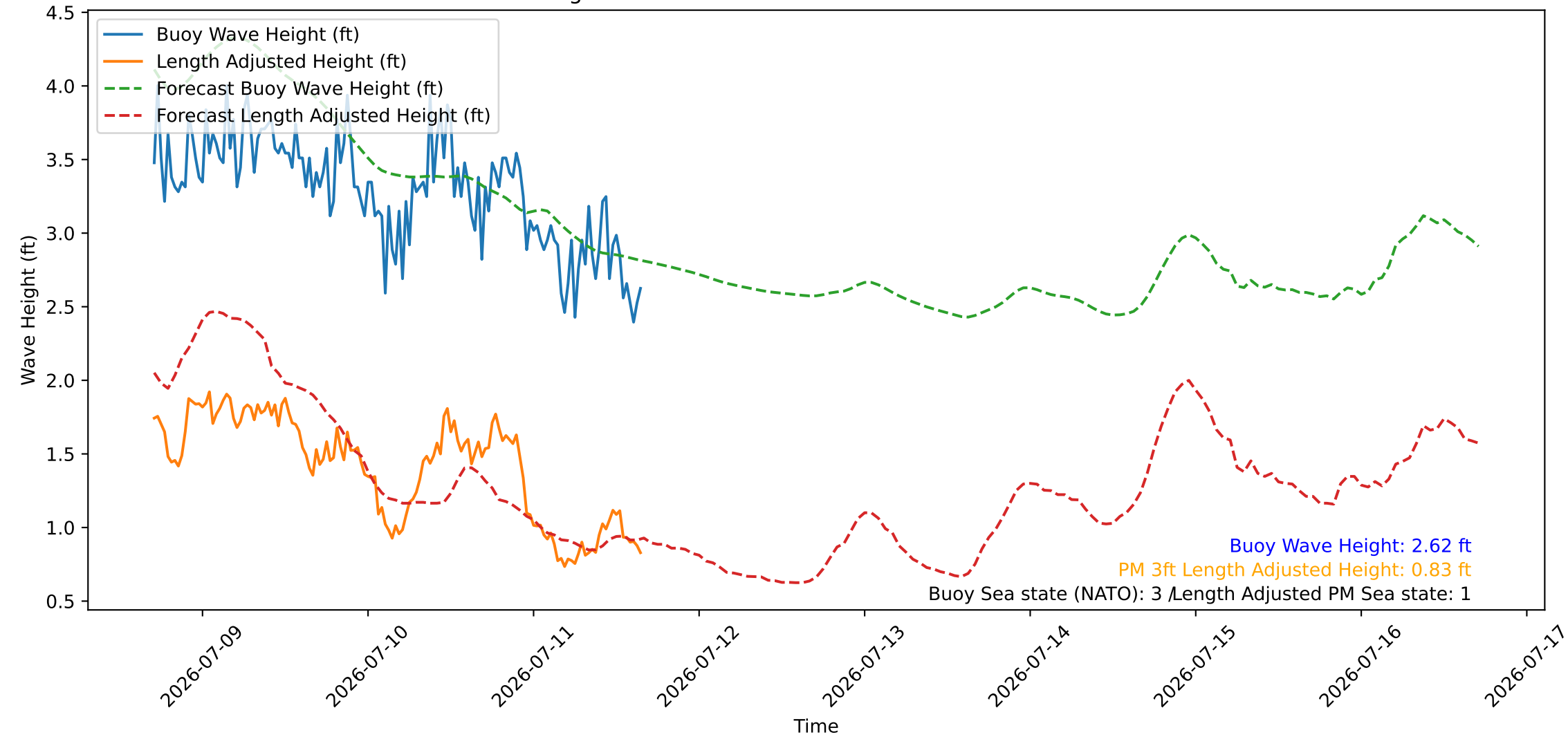
Wave Heights over Time for Red Beach at 2026-07-11 16:40:45
