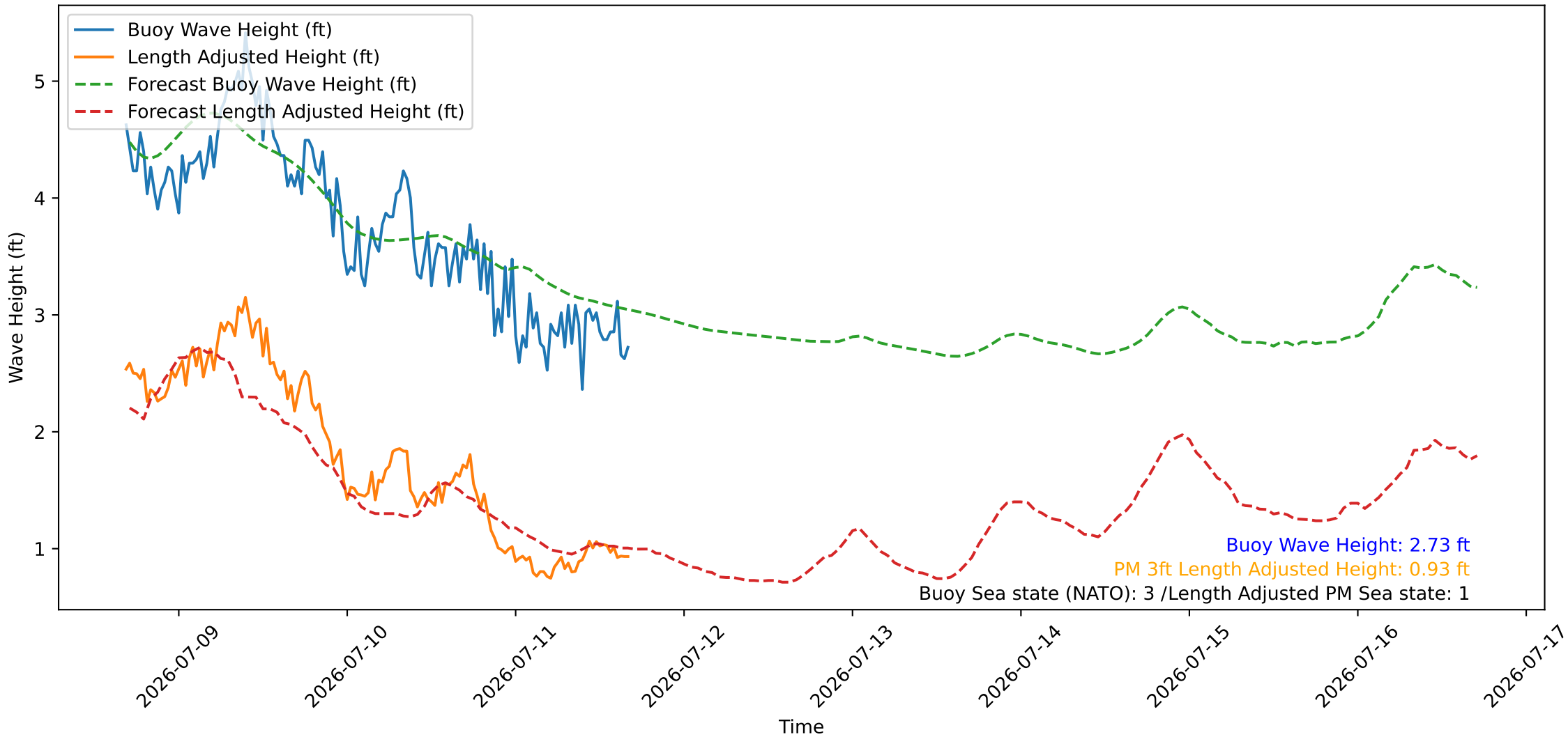
Wave Heights over Time for Oceanside Harbor at 2026-07-11 16:40:26
